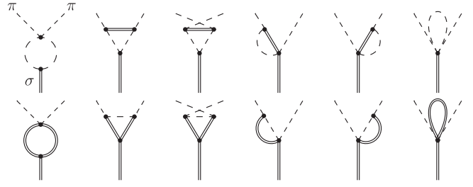
FIG. 11. NLO diagrams that contribute to the resonance structure of f_0/\sigma in \chi\text{PT}_\sigma . Ultraviolet divergences arising from the loops are absorbed (in the usual way) by counterterms in the NLO Lagrangian.
