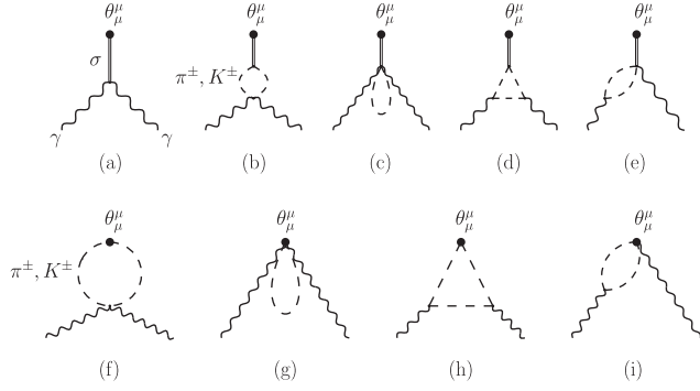
FIG. 8. Lowest order contributions to \langle \gamma_1, \gamma_2 | \tilde{\theta}_\mu^\mu(0) | \text{vac} \rangle in \chi\text{PT}_\sigma . Diagram (a) is generated by the contact term proportional to g_{\sigma\gamma\gamma} , while diagrams (d), (e), (h), and (i) are each accompanied by an additional crossed amplitude (diagrams not shown). Similar loop diagrams have been considered in \chi\text{PT}_3 for K_S \rightarrow \gamma\gamma [33], K_L \rightarrow \pi^0\gamma\gamma [53], and \gamma\gamma \rightarrow \pi^0\pi^0 [55,56].
