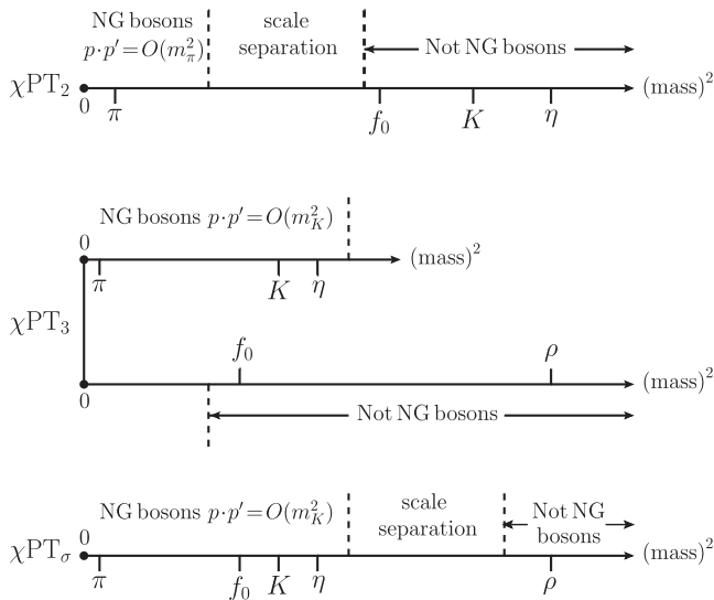
FIG. 4. Scale separations between NG sectors and other hadrons for each type of chiral perturbation theory \chi\text{PT} discussed in this paper. Note that scale separation in \chi\text{PT}_2 [chiral SU(2)_L \times SU(2)_R , top diagram] is ensured by limiting extrapolations in momenta p, p' to O(m_\pi) [not O(m_K) ]. In conventional three-flavor theory \chi\text{PT}_3 (middle diagram), there is no scale separation: the non-NG boson f_0(500) sits in the middle of the NG sector \{\pi, K, \eta\} . Our three-flavor proposal \chi\text{PT}_\sigma (bottom diagram) for O(m_K) extrapolations in momenta implies a clear scale separation between the NG sector \{\pi, K, \eta, \sigma = f_0\} and the non-NG sector \{\rho, \omega, K^*, N, \eta', \dots\} .
