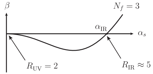
FIG. 9. Drell-Yan ratios R_{\text{UV}} and R_{\text{IR}} associated with the proposed \beta/\psi function. For e^+e^- \rightarrow hadrons at high energies with 0 < \alpha_s < \alpha_{\text{IR}} , the strong coupling \alpha_s runs to zero, and the result R_{\text{UV}} is perturbative (asymptotic freedom). However, if \alpha_s is at \alpha_{\text{IR}} , it cannot run, so we get a nonperturbative result R_{\text{IR}} associated with short -distance scaling at the infrared fixed point.
