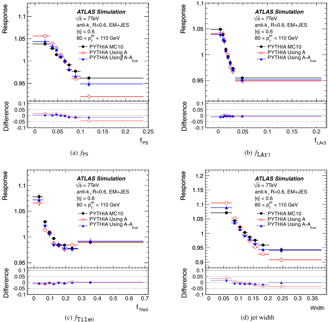
Fig. 47 Average jet response calculated using truth jets ( full circles ), using the reconstructed asymmetry A ( open circles ), and using A - A_{true} ( triangles ) as a function of the calorimeter layer energy fraction f_{PS} ( a ), f_{LAr3} ( b ), f_{Tile0} ( c ) and the lateral jet width ( d ) in the PYTHIA MC10 sample before applying GS calibration. The lower part
