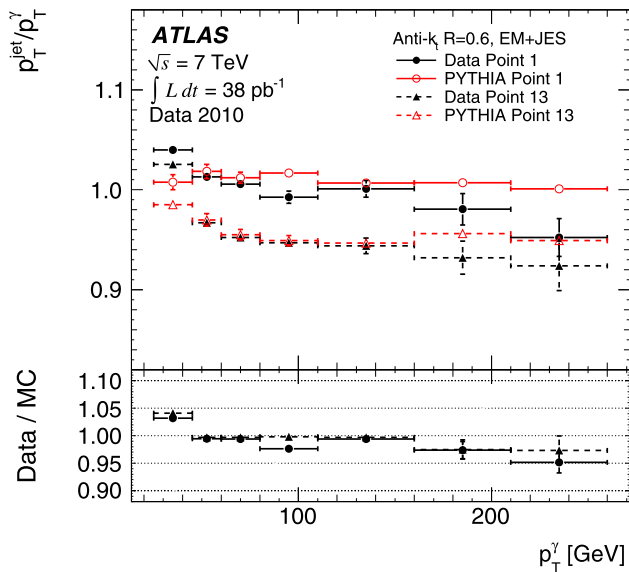
Fig. 29 Average jet response as determined by the direct p_T balance technique with the nominal selection (Point 1) and with a set of relaxed radiation suppression cuts (Point 13), for anti- k_r jets with R = 0.6 calibrated with the EM+JES scheme within |\eta| < 1.2 as a function of the photon transverse momentum for data and Monte Carlo simulation. Only statistical uncertainties are shown
