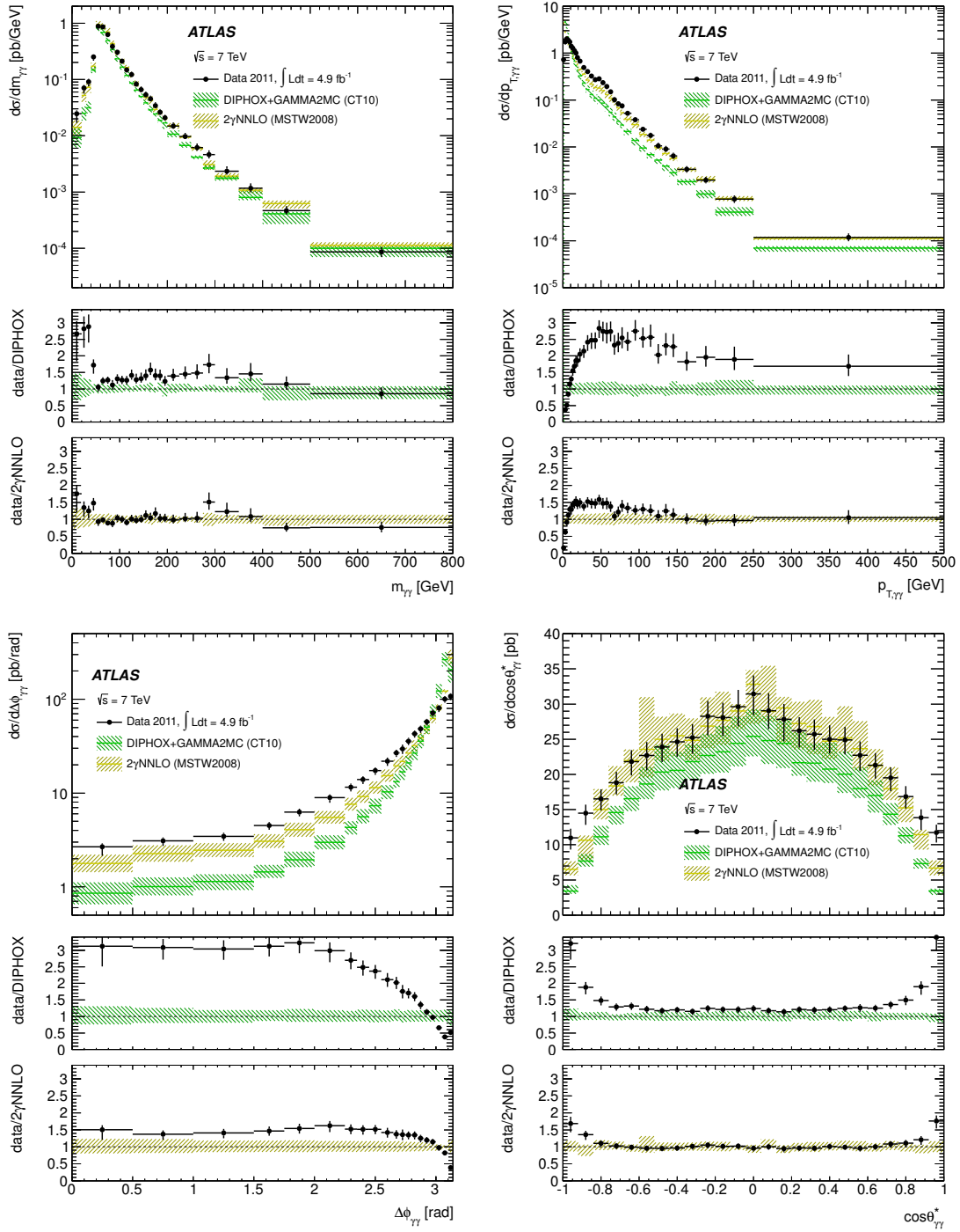
Figure 5. Comparison between the experimental cross sections and the predictions obtained with DIPHOX+GAMMA2MC (NLO) and 2 \gamma NNLO (NNLO): m_{\gamma\gamma} (top left), p_{T,\gamma\gamma} (top right), \Delta\phi_{\gamma\gamma} (bottom left), \cos\theta_{\gamma\gamma}^* (bottom right). Black dots correspond to data with with error bars for their total uncertainties, which are dominated by the systematic component. The theoretical uncertainties include contributions from the limited size of the simulated sample, from the scale choice and from uncertainties on the parton distribution functions and on the hadronization and underlying event corrections.
