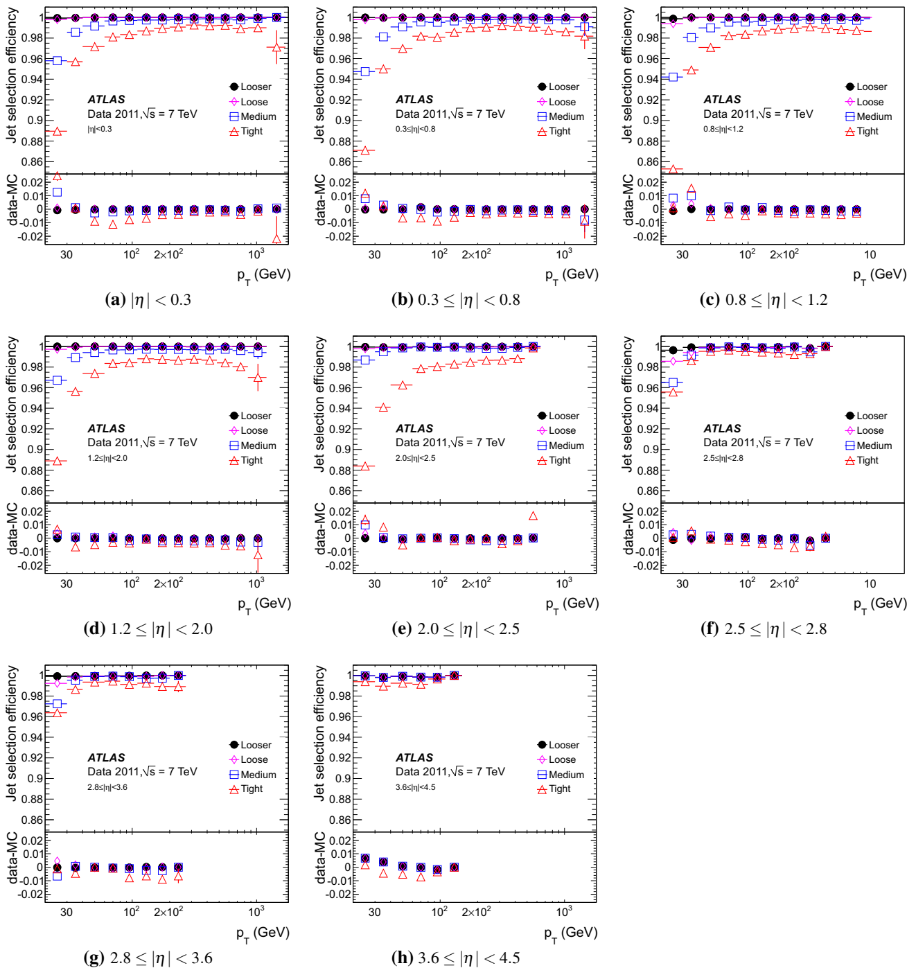
Fig. 5 Jet quality selection efficiency for anti- k_r jets with R = 0.4 measured with a tag-and-probe technique as a function of p_T^{\text{jet}} in various \eta ranges, for the four sets of selection criteria. Only statistical uncertainties are shown. Differences between data and MC simulations are also shown
