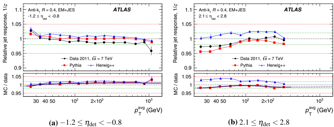
Fig. 12 Relative jet response ( 1/c ) as a function of the average jet p_T of the dijet system for anti- k_r jets with R = 0.4 calibrated with the EM+JES scheme, separately for a -1.2 \leq \eta_{\text{det}} < -0.8 and b
