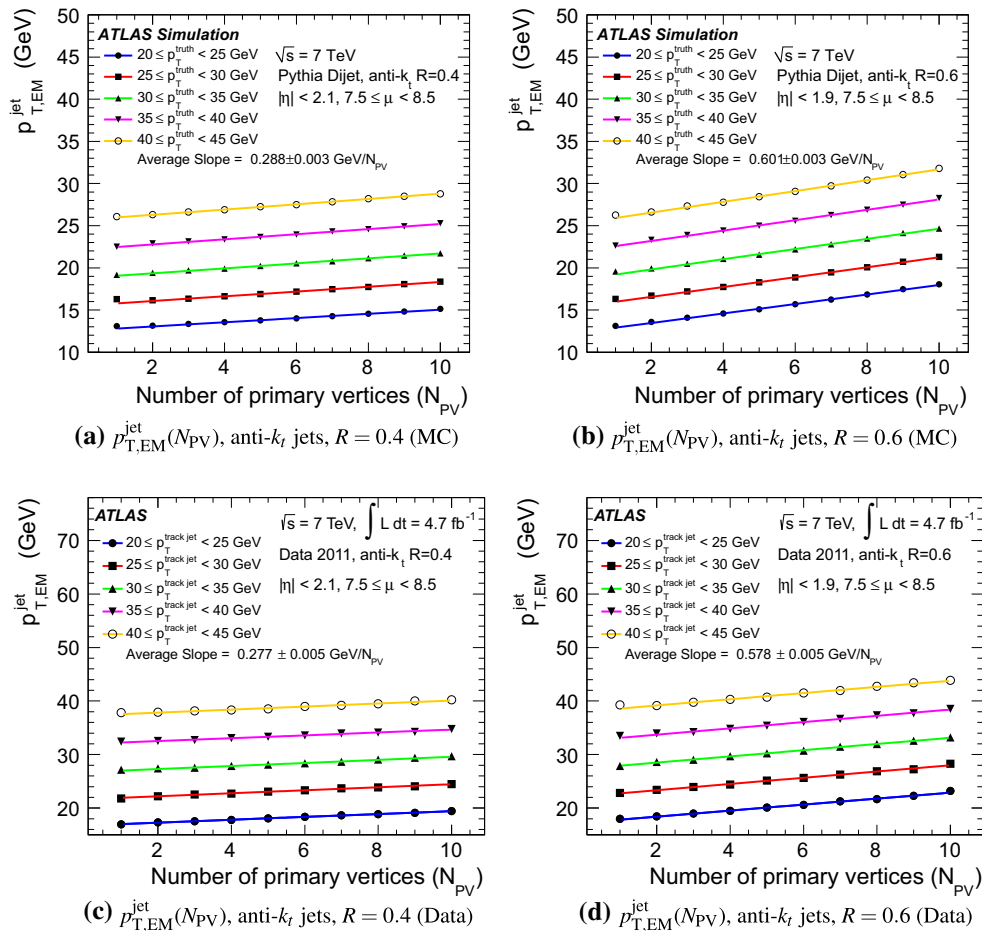
Fig. 6 The average reconstructed transverse momentum p_{T,EM}^{jet} on EM scale for jets in MC simulations, as function of the number of reconstructed primary vertices N_{PV} and 7.5 \leq \mu < 8.5 , in various bins of truth-jet transverse momentum p_T^{truth} , for jets with a R = 0.4 and b
