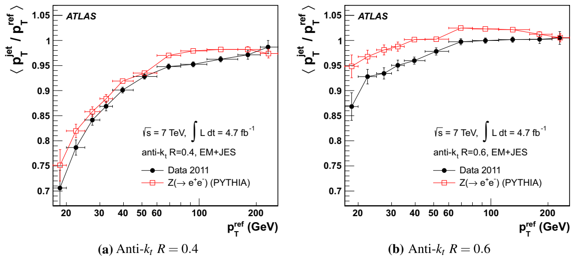
Fig. 17 Mean p_T balance obtained in the data and with the PYTHIA simulation. Results for anti- k_t jets with distance parameter a R = 0.4 and R = 0.6 calibrated with the EM+JES scheme are shown. Only statistical uncertainties are shown
