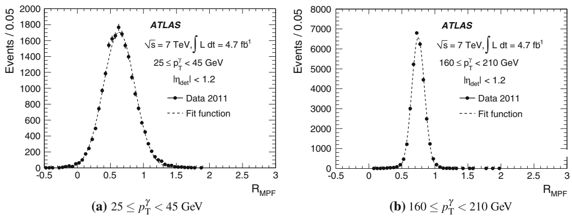
Fig. 21 MPF response distributions in the \gamma -jet data for a 25 \leq p_T^\gamma < 45 GeV and b 160 \leq p_T^\gamma < 210 GeV when using topo-clusters at the EM scale. The dashed lines represent the fits with a Gaussian function.
