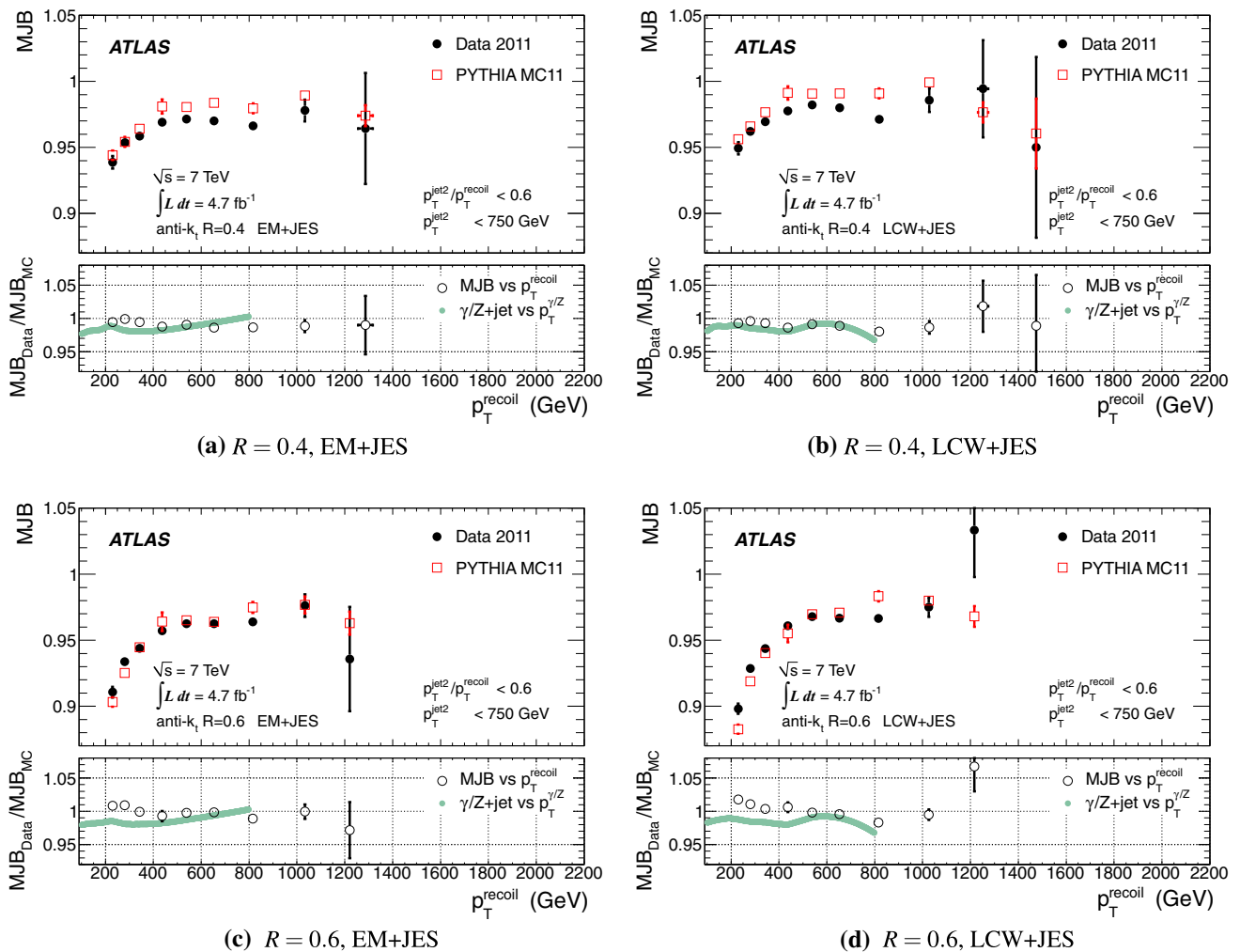
Fig. 29 Multijet balance as a function of the recoil system p_T^{\text{recoil}} for anti- k_r jets with (a, b) R = 0.4 and (c, d) R = 0.6 , calibrated with the (a, c) EM+JES scheme and with the (b, d) LCW+JES scheme, for both data and MC simulations. The non-leading jets in the data with p_T < 750 GeV are corrected by the combination of \gamma -jet and Z-jet in situ calibrations as described in Sect. 11.1. The open points in the
