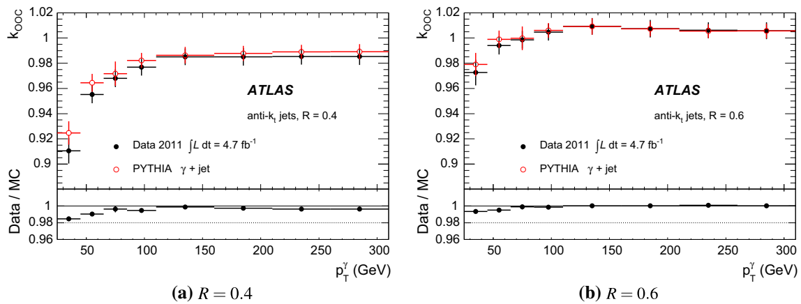
Fig. 26 Out-of-cone radiation factor k_{OOC} relating the p_T of the photon with the p_T of the truth jet as a function of the photon transverse momentum, measured using charged particles, for anti- k_t jets with a
