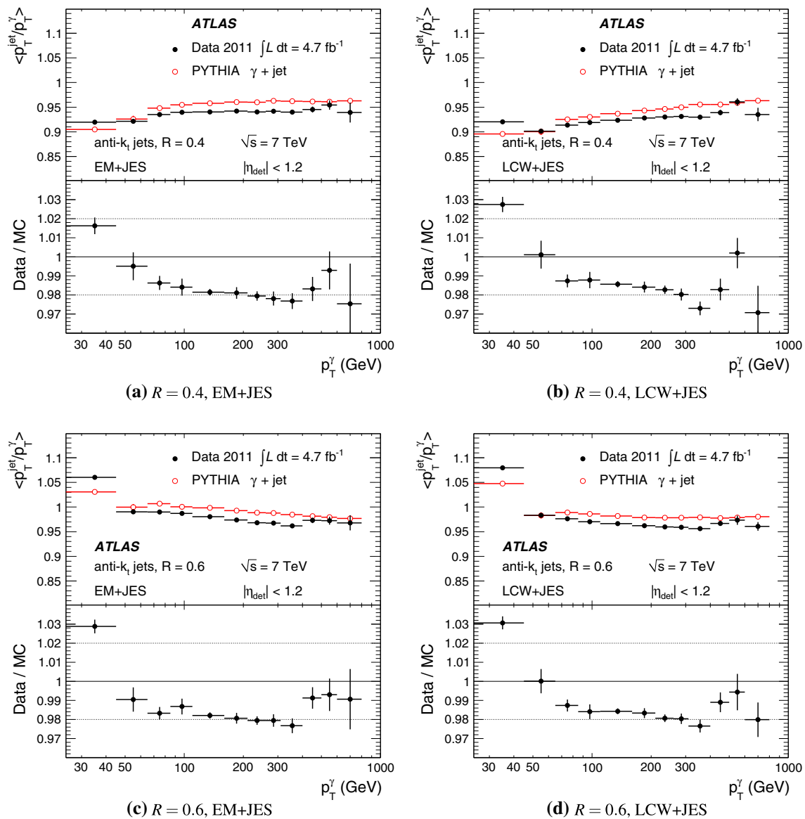
Fig. 24 Average jet response as determined by the DB technique in \gamma -jet events for anti- k_r jets with (a, b) R = 0.4 and (c, d) R = 0.6 , calibrated with the (a, c) EM+JES scheme and with the (b, d) LCW+JES
