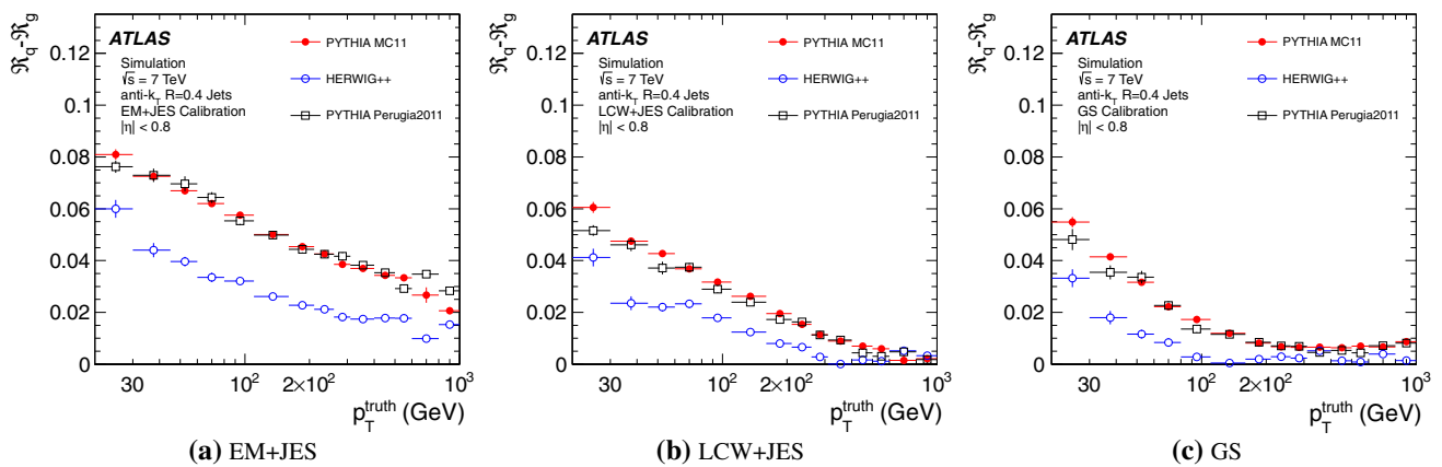
Fig. 51 Difference in jet response \mathcal{R} = p_T^{\text{jet}}/p_T^{\text{truth}} of isolated jets initiated by light quarks and gluons as a function of the true jet p_T , for anti- k_r jets with R = 0.4 in the barrel calorimeter. Three different calibration schemes are shown for a the EM+JES calibration, b the LCW+JES
