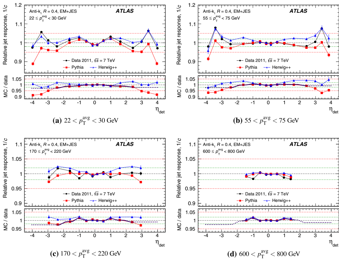
Fig. 11 Relative jet response ( 1/c ) as a function of the jet pseudorapidity for anti- k_r jets with R = 0.4 calibrated with the EM+JES scheme, separately for a 22 \leq p_T^{\text{avg}} < 30 GeV, b 55 \leq p_T^{\text{avg}} < 75 GeV, c 170 \leq p_T^{\text{avg}} < 220 GeV and d 600 \leq p_T^{\text{avg}} < 800 GeV. The lower parts of the figures show the ratios between the data and MC relative
