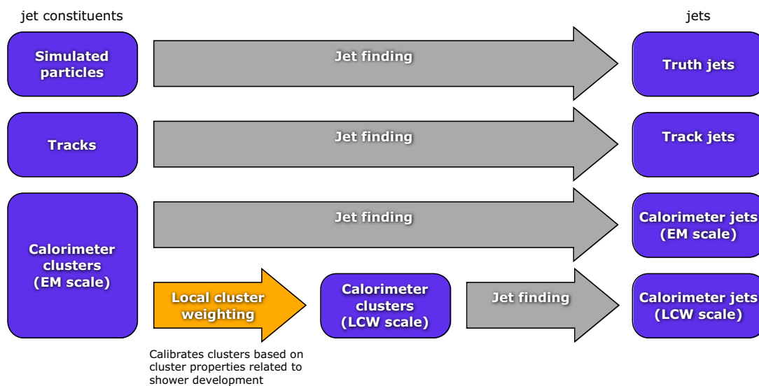
Fig. 2 Overview of the ATLAS jet reconstruction. After the jet finding, the jet four momentum is defined as the four momentum sum of its constituents
