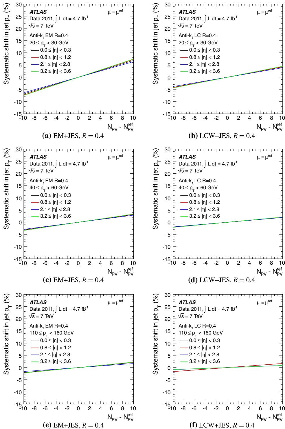
Fig. 46 The fractional systematic shift due to mis-modelling of the effect of in-time pile-up on the transverse momentum p_{T,EM+JES}^{jet} of jets reconstructed with the anti- k_r algorithm with R = 0.4 , and calibrated with the EM+JES scheme, is shown as a function of (N_{PV} - N_{PV}^{ref}) in a ,
