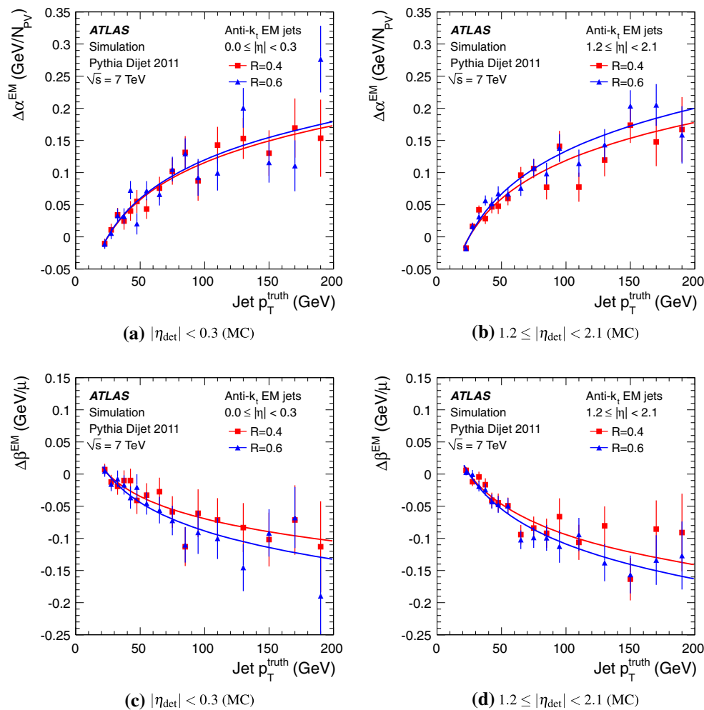
Fig. 45 The difference from the average \alpha^{\text{EM}}(\eta_{\text{det}}) of the in-time pile-up signal contribution per reconstructed primary vertex ( \Delta(\partial p_{T,\text{EM}}^{\text{jet}}/\partial N_{\text{PV}})(p_T^{\text{truth}}) ) as a function of the true jet transverse momentum p_T^{\text{truth}} , for MC-simulated jets reconstructed with anti- k_t R = 0.4 and R = 0.6 at the EM scale, in two different regions a |\eta_{\text{det}}| < 0.3 and b 1.2 \leq |\eta_{\text{det}}| < 2.1 of the ATLAS calorimeter. In c and
