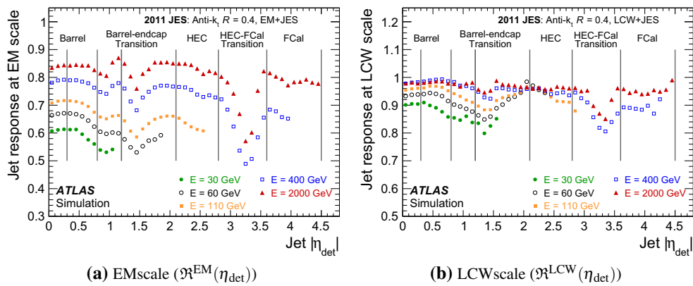
Fig. 4 Average response of simulated jets formed from topo-clusters, calculated as defined in Eq. (1) and shown in a for the EM scale ( \mathfrak{R}^{EM} ) and in b for the LCW scale ( \mathfrak{R}^{LCW} ). The response is shown separately for various truth-jet energies as function of the uncorrected (detector) jet
