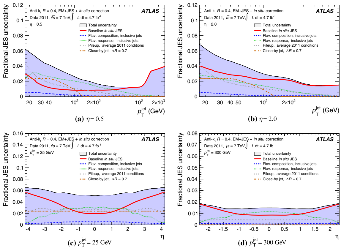
Fig. 63 Sample-dependent fractional jet energy scale systematic uncertainty as a function of a, b p_T^{\text{jet}} and c, d jet pseudorapidity for anti- k_r jets with distance parameter of R = 0.4 calibrated using the
