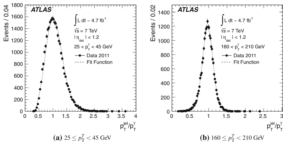
Fig. 22 Jet response distributions in the \gamma -jet data for a 25 \leq p_T^\gamma < 45 GeV and b 160 \leq p_T^\gamma < 210 GeV as measured by the DB technique for anti- k_r jets with R = 0.6 at the EM+JES scale. The dashed lines represent fits of Gaussian functions, except in the lowest bin
