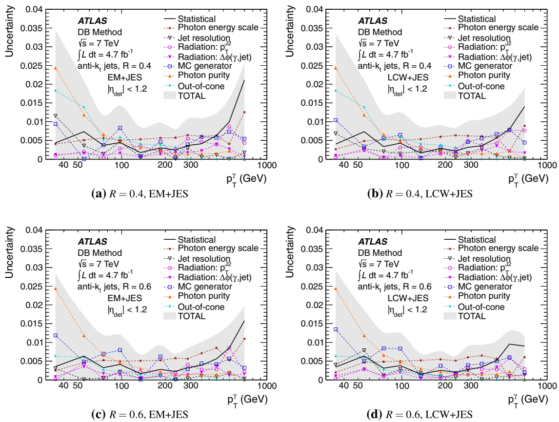
Fig. 28 Systematic uncertainties on the data-to-MC ratio of the jet response, as determined by the DB technique in \gamma -jet events, for anti- k_r jets with (a, b) R = 0.4 and (c, d) R = 0.6 , calibrated with the (a, c)
