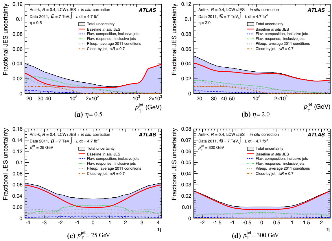
Fig. 64 Sample-dependent fractional jet energy scale systematic uncertainty as a function of a, b p_T^{\text{jet}} and c, d jet pseudorapidity for anti- k_r jets with distance parameter of R = 0.4 calibrated using the
