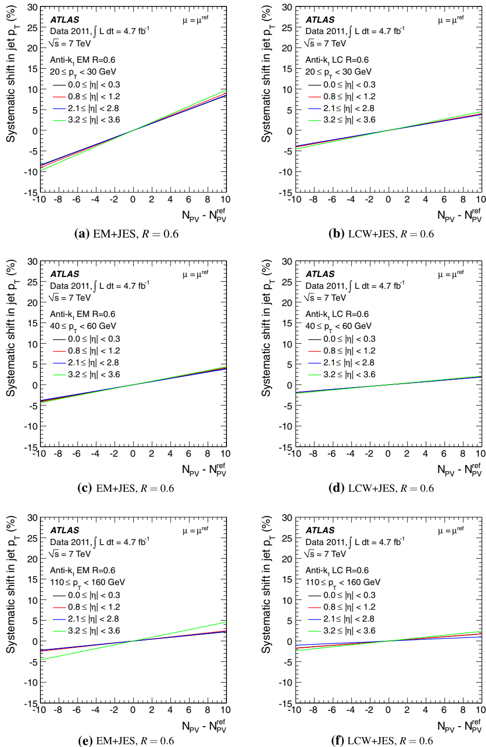
Fig. 47 The fractional systematic shift due to mis-modelling of the effect of in-time pile-up on the transverse momentum p_{T,EM+JES}^{jet} of jets reconstructed with the anti- k_t algorithm with R = 0.6 and calibrated with the EM+JES scheme, is shown as a function of (N_{PV} - N_{PV}^{ref}) in a ,
