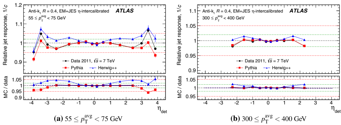
Fig. 34 Relative jet response, 1/c , as a function of the jet \eta_{det} for anti- k_r jets with R = 0.4 calibrated with the EM+JES scheme and in addition the derived \eta -intercalibration. Results are shown separately for a 55 \leq p_T^{avg} < 75 GeV and b 300 \leq p_T^{avg} < 400 GeV. For all points included in the original calibration ( |\eta_{det}| < 2.8 ), the data are corrected
