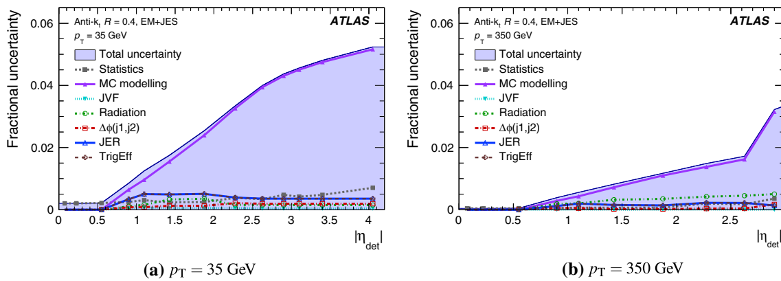
Fig. 13 Summary of uncertainties on the intercalibration as a function of the jet \eta_{\text{det}} for anti- k_T jets with R = 0.4 calibrated with the EM+JES scheme, separately for a p_T = 35 GeV and b p_T = 350 GeV.
