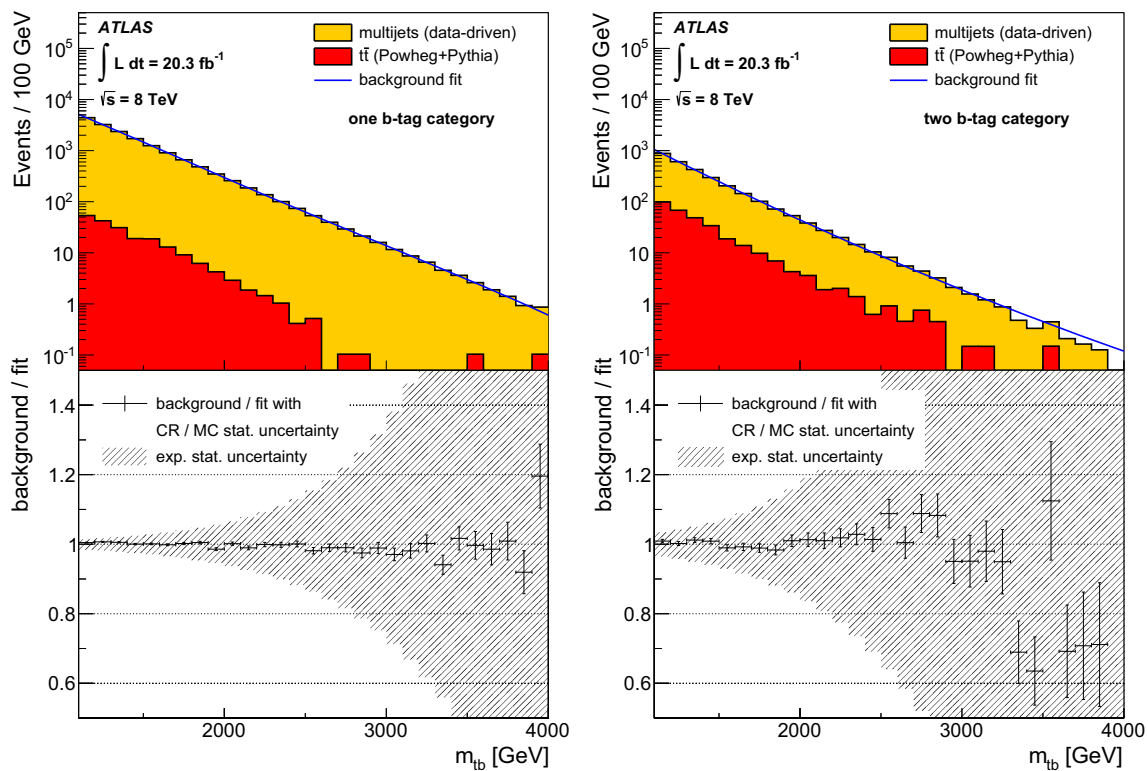
Fig. 4 Fit to the m_{tb} distribution from the initial background estimate in the one b -tag category ( left ) and in the two b -tag category ( right ). The ratio background/fit is also shown, where the uncertainties are the
