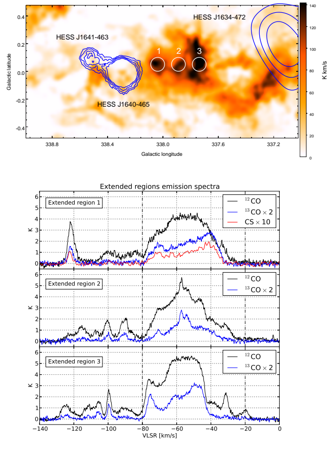
Figure 6. Top: Integrated ^{12}\text{CO} emission image [K km/s] between -80 and -20 km/s from l = 339^\circ to l = 337^\circ . Blue contours indicate the positions of HESS J1640–465 and HESS J1641–463 (Abramowski et al. 2014b). Contours for the TeV source HESS J1634–472 are also shown in blue for completeness (Aharonian et al. 2006). Bottom: Average ^{12}\text{CO}(1-0) (black) and ^{13}\text{CO}(1-0) (blue) emission spectra in three circular regions indicated above in white. CS(1-0) emission from 7 mm observations is displayed in red for extended region 1. ^{13}\text{CO} and CS(1-0) emission have been scaled by a factor of 2 and 10 respectively for clarity. Vertical dashed lines indicate the integration range used to produce the image in the top panel.
