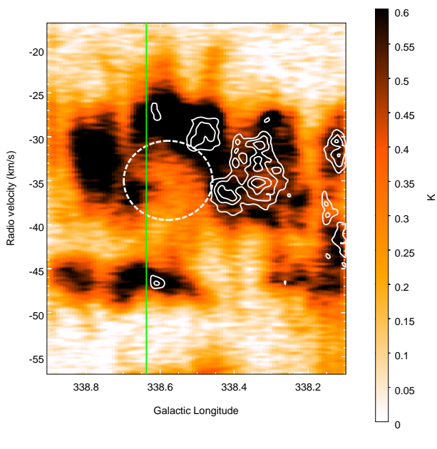
Figure 4. Position-velocity image [K] (in Galactic longitude) of ^{12}\text{CO}(1-0) emission towards the bubble feature seen towards HESS J1641–463 in the region indicated in Figure 3. The approximate position of the cavity discussed in text is indicated by the dashed white ellipse. The solid white contours indicate CS(1-0) emission detected in our 7 mm observations. Note that the extent of the coverage in 7 mm only reaches the vertical green line in longitude.
