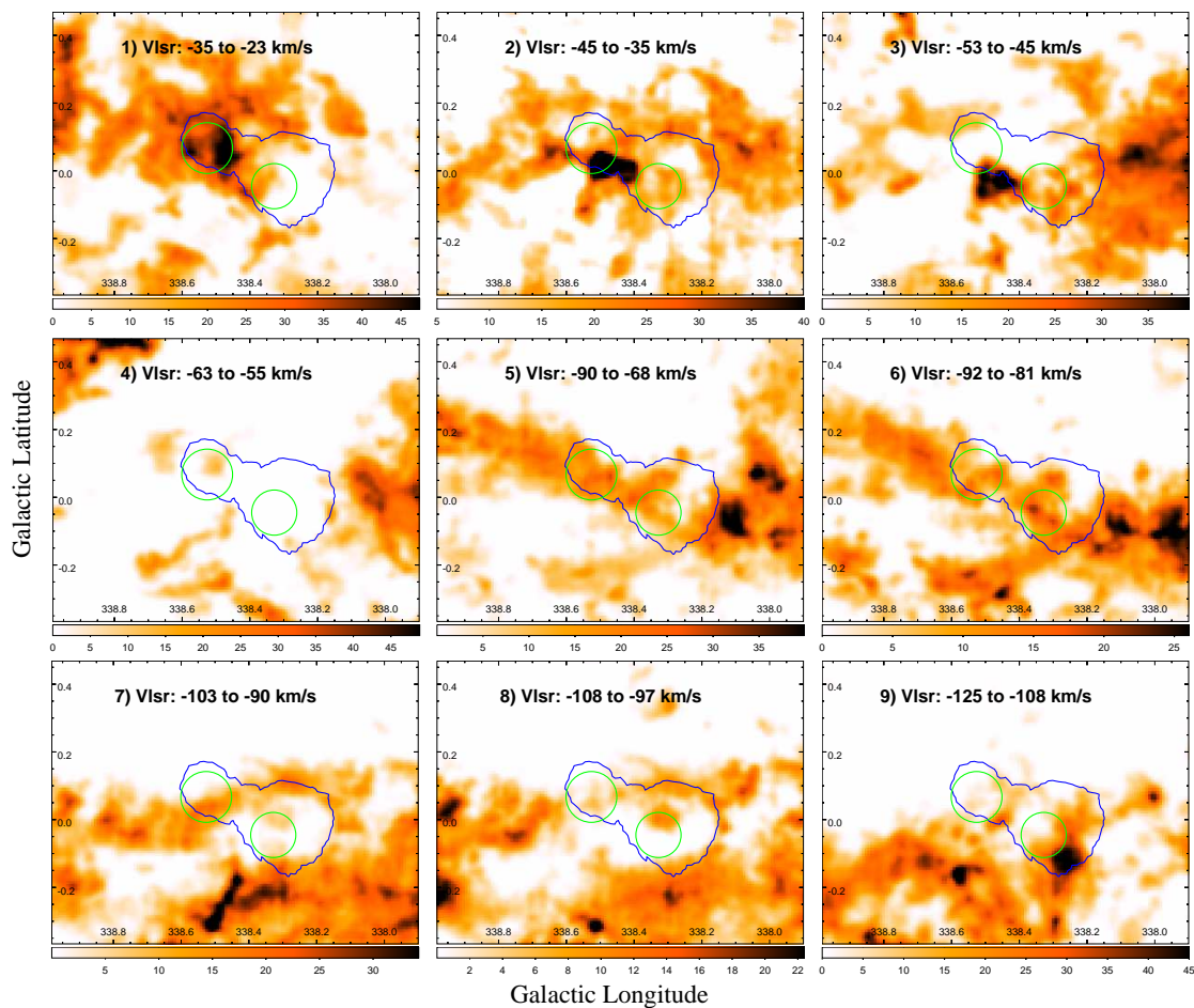
Figure 2. Integrated ^{12}\text{CO}(1-0) emission images [K km/s] over indicated velocity intervals. Single blue 5\sigma significance H.E.S.S. contour used for clarity. The position and extent of SNR G338.5+0.1 and SNR G338.3-0.0 are indicated by the left and right solid green circles respectively in each panel.
