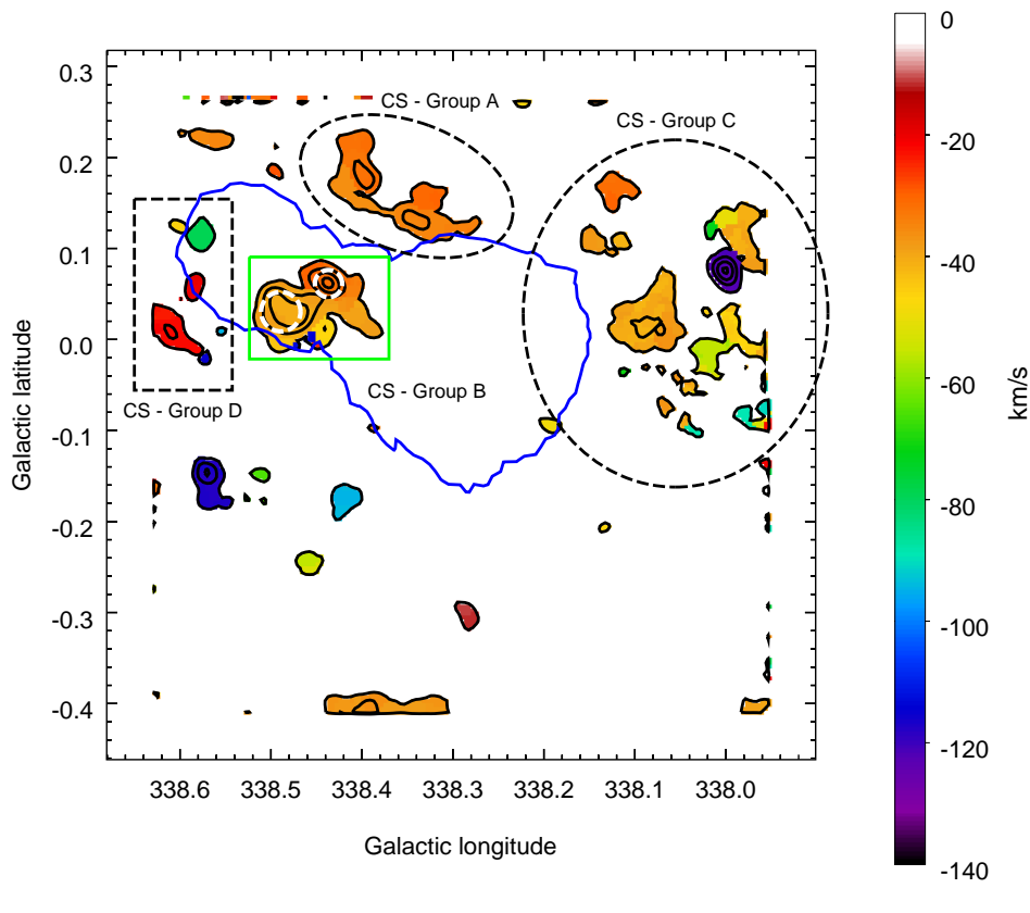
Figure 7. Velocity of peak pixel CS(1-0) map [km/s] in the 7 mm observations region. Overlaid solid black contours show the intensity of the peak pixel. H.E.S.S. 5\sigma significance contour is in solid blue. Regions of interest discussed in the text are labelled by black dashed ellipses. The CS - Group B region, however, is outlined by a solid green box and indicates the integration region for the position-velocity plot shown in Figure 9. Dashed white circles indicate apertures used to extract spectra for Bridge Core 1 (left circle) and Bridge Core 2 (right circle) discussed in the text.
