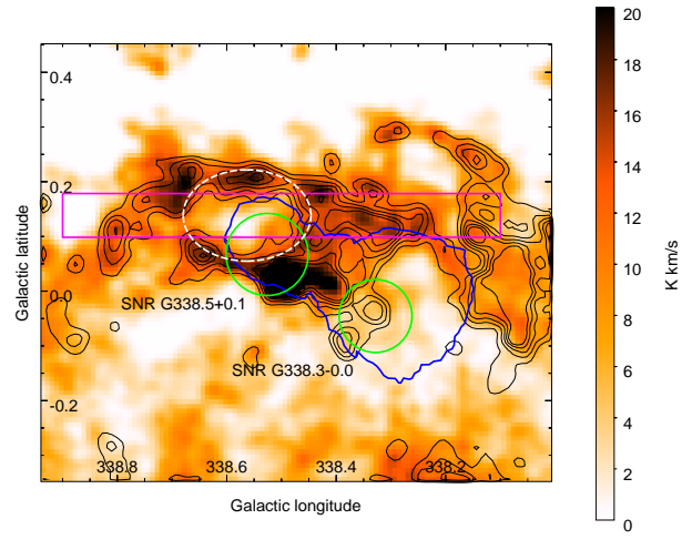
Figure 3. Mopra ^{12}\text{CO}(1-0) emission image [K km/s] integrated between -40 and -35 km/s. Single solid blue contour is 5\sigma significance from H.E.S.S. observations towards HESS 1640–465 and HESS 1641–463. The white dashed ellipse is the approximate position of a ring feature discussed in the text and the solid magenta box is the integration region for the position-velocity plot shown in Figure 4. Overlaid black contours are from Mopra ^{13}\text{CO}(1-0) observations. SNRs are indicated by green circles.
