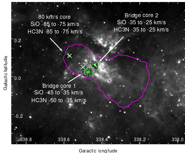
Figure 10. Spitzer 8.0 \mu\text{m} image towards HESS J1640–465 and HESS J1641–463. Single magenta contour is 5 \sigma significance from H.E.S.S. observations. Green solid contours are integrated SiO(1–0) emission. Dashed black contours are integrated HC 3 N(5–4, F=4–3) emission. The velocities over which they are integrated are as labelled. White Xs indicate positions of observed CH 3 OH (I) masers.
