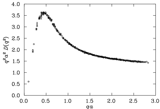
Figure 3. The gluon propagator multiplied by q^2 as a function of q for the large lattice, after the cylindrical cut.
