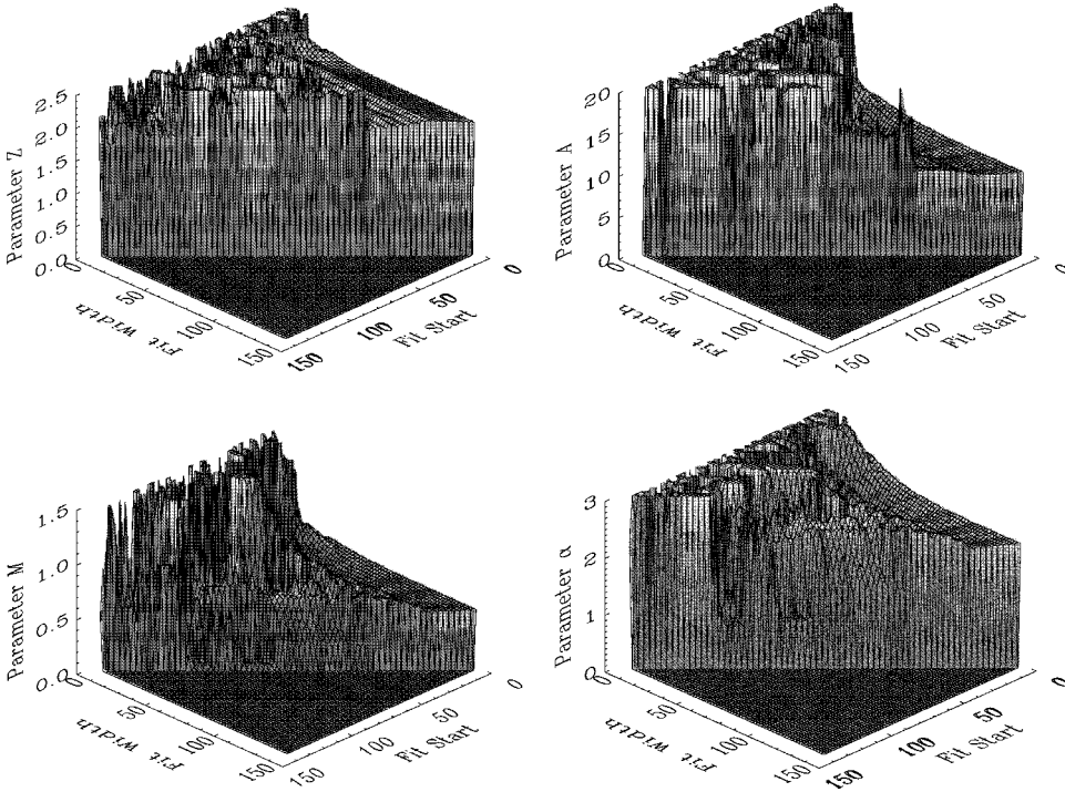
FIG. 14. Stability plots for model A. All the parameter values are stable over the region of interest.
