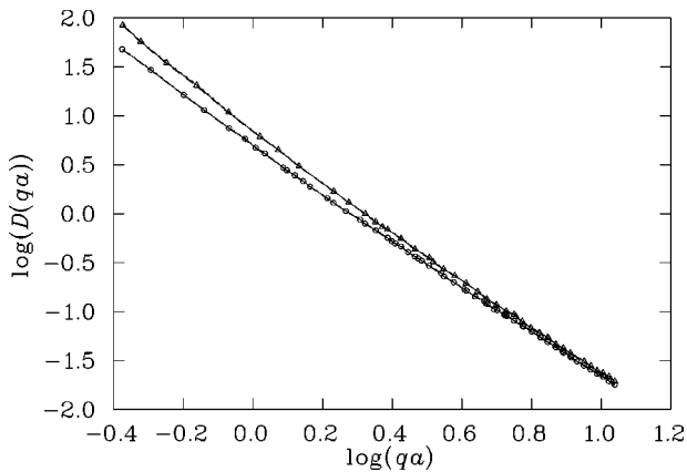
FIG. 10. The dimensionless, unrenormalized gluon propagator as a function of \ln(qa) for the two values of \beta . The triangles denote the data for the small (coarse) lattice at \beta=6.0 , while the circles denote the data for \beta=6.2 . The lines represent linear interpolations between the data points.
