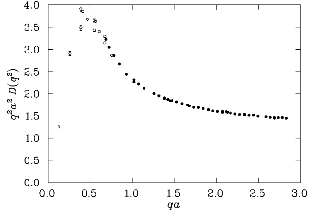
FIG. 7. The gluon propagator from the small lattice multiplied by q^2 a^2 . The points displayed in this plot lie within a cylinder of radius \Delta\hat{q}a < 1 \times 2\pi/16 directed along the diagonal (x,y,z,t) = (1,1,1,1) of the lattice. The solid points also lie within a cone of 20^\circ measured from the diagonal at the origin.
