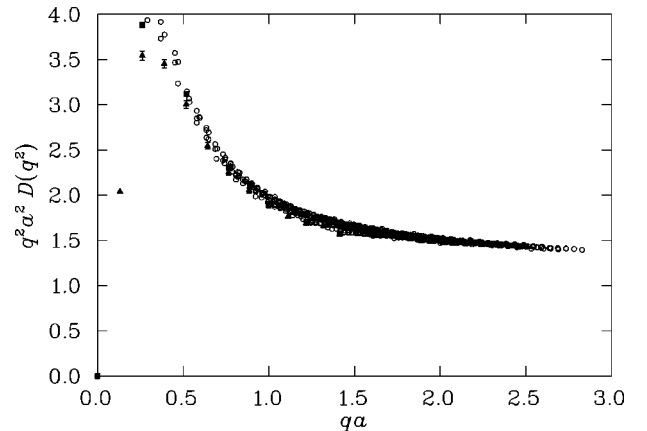
FIG. 5. The gluon propagator from the fine lattice multiplied by q^2 a^2 plotted as a function of momenta qa . The symbols are as in Fig. 2.
