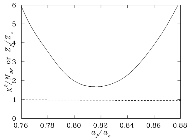
FIG. 11. \chi^2 per degree of freedom as a function of the ratio of lattice spacings for matching the small and fine lattice data, using \hat{q} as the momentum variable. The dashed line indicates the ratio R_Z of the renormalization constants.
