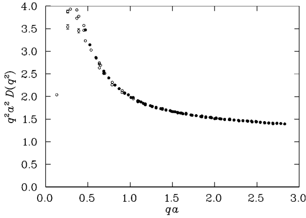
FIG. 9. The gluon propagator from the fine lattice multiplied by q^2 a^2 . The points displayed in this plot lie within a cylinder of radius \Delta \hat{q} a < 1.5 \times 2\pi/32 directed along the diagonal of the lattice. The solid points also lie within a cone of 20^\circ measured from the diagonal at the origin.
