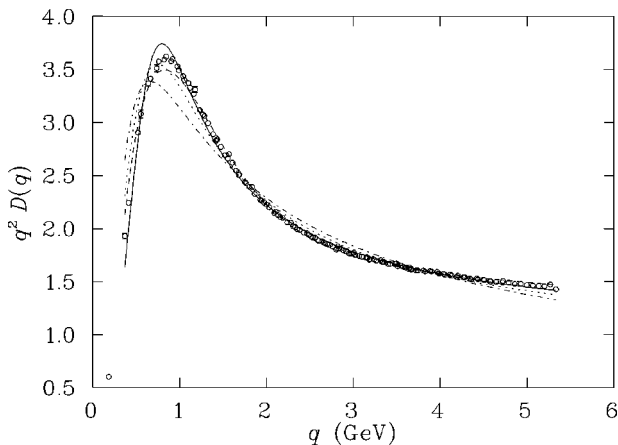
FIG. 17. The gluon propagator multiplied by q^2 , with nearby points averaged. The lines illustrate the best fit of various other models. The solid line is model B, the dotted line is Cornwall I, the dash-dotted line is Marenzoni et al. and the dashed line is model C.
