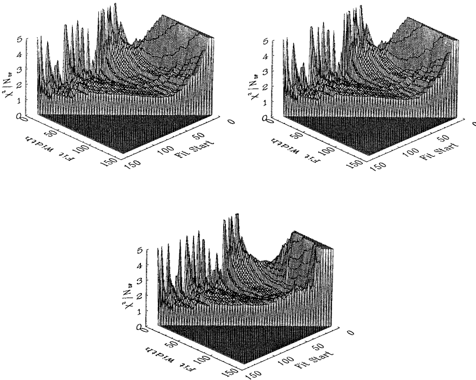
FIG. 13. \chi^2 per degree of freedom for fits of model A (top left), model B (top right) and model C (bottom). The “Fit start” axis indicates the starting point for the fit, while the “Fit width” axis indicates the number of points included in the fit. The most inclusive fits are in the near right-hand corner, with the smallest value for the starting point and the largest number of points included. We see that model A is stable over a wide variety of fitting ranges, while the other two models fail to account properly for the data in the infrared.
