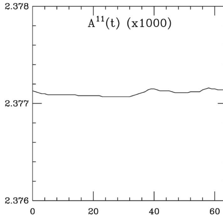
FIG. 1. Plots of the (1,1) color component of \sum_{\vec{x}} \vec{A}_4(\vec{x}, t) as a function of t for one gauge fixed configuration on the small lattice (left), and on the large lattice (right).
