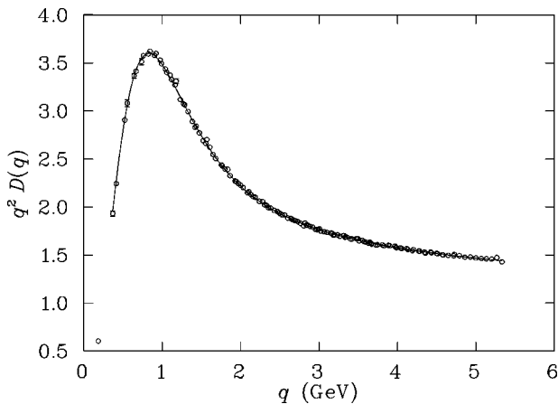
FIG. 15. The gluon propagator multiplied by q^2 , with nearby points averaged. The line illustrates our best fit of model A defined in Eq. (5.14). The fit is performed over all points shown, excluding the one at the lowest momentum value, which may be sensitive to the finite volume of the lattice. The scale is taken from the value for the string tension quoted in Ref. [23].
