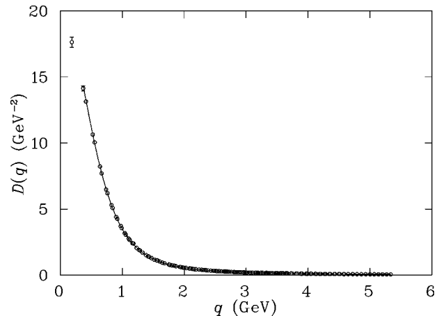
FIG. 16. The gluon propagator in physical units. The line illustrates our best fit of model A, as in Fig. 15.
