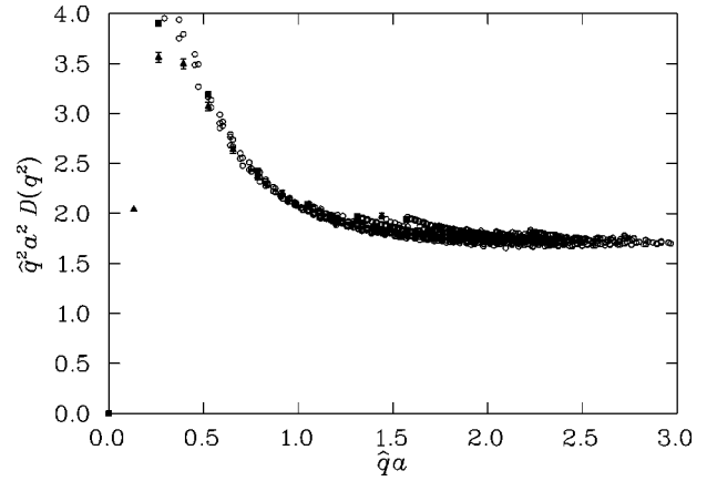
FIG. 4. The gluon propagator from the fine lattice multiplied by \hat{q}^2 a^2 plotted as a function of momenta \hat{q}a . The symbols are as in Fig. 2.
