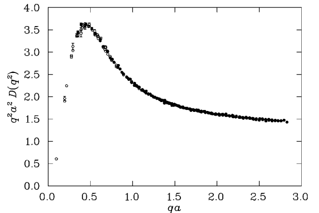
FIG. 8. The gluon propagator from the large lattice multiplied by q^2 a^2 . The points displayed in this plot lie within a cylinder of radius \Delta\hat{q}a < 2 \times 2\pi/32 directed along the diagonal of the lattice. The solid points also lie within a cone of 20^\circ measured from the diagonal at the origin.
