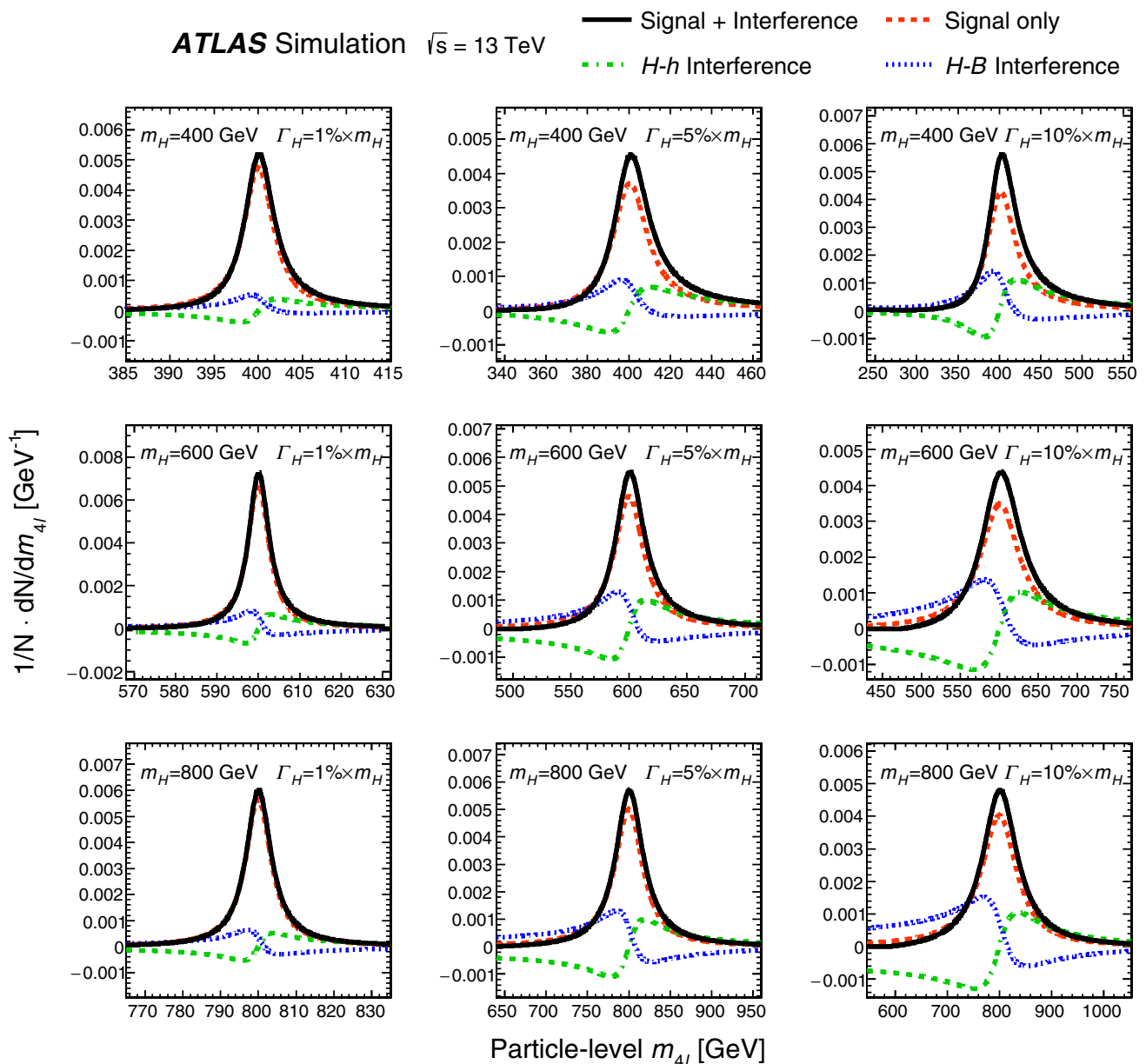
Fig. 2 Particle-level four-lepton mass m_{4\ell} model for signal only (red), H-h interference (green), H-B interference (blue) and the sum of the three processes (black). Three values of the resonance mass m_H (400, 600, 800 GeV) are chosen, as well as three values of the resonance width \Gamma_H (1, 5, 10% of m_H ). The signal cross section, which determines the
