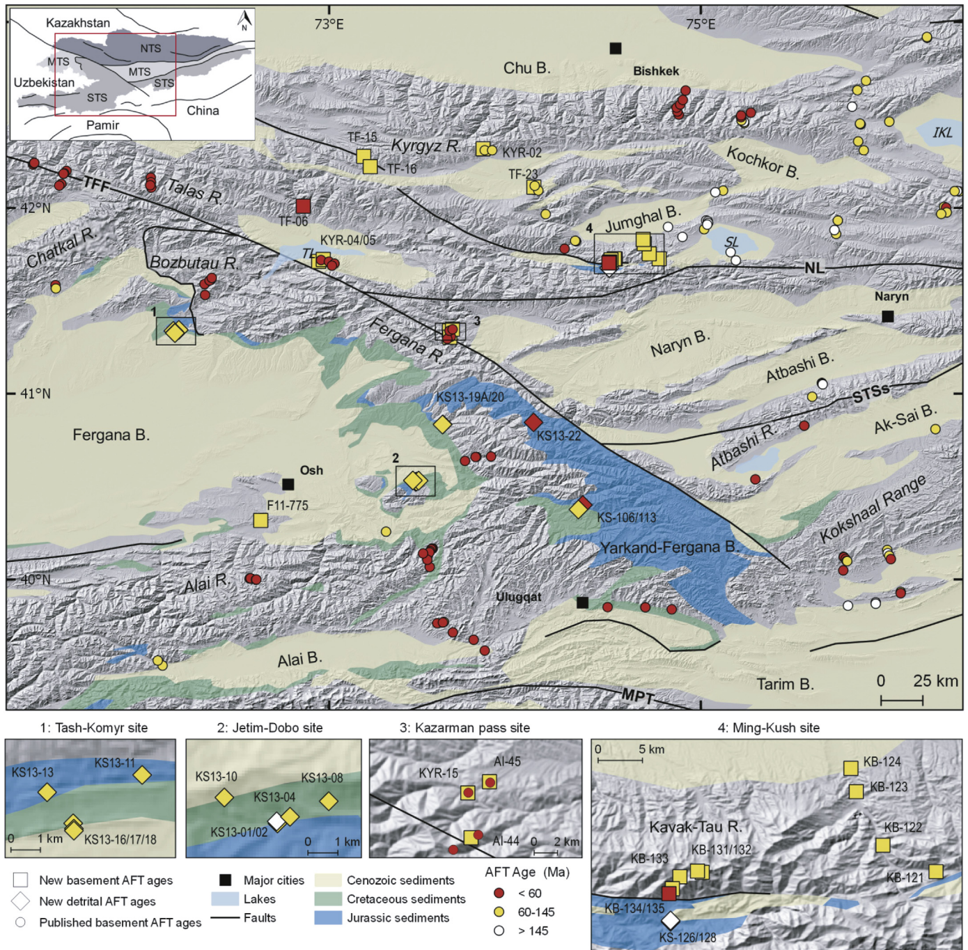
Figure 2. Shaded relief map of the study area with indication of the sample locations and Jurassic, Cretaceous and Cenozoic sediments. Non-coloured areas represent the crystalline and pre-Mesozoic basement. Detail maps: (1) Tash-Komyr site (Fergana Basin); (2) Jetim-Dobo site (Fergana Basin); (3) Kazarman pass site; (4) Ming-Kush site. Compilation of available published apatite fission-track (AFT) ages from crystalline and pre-Mesozoic basement rocks is based on data from Sobel et al. (2006a, b), Glorie et al. (2010, 2011), De Grave et al. (2011a, 2012, 2013), Macaulay et al. (2013, 2014), Bande et al. (2015a, 2017), Käšner et al. (2016) and are indicated as circles. Squares reflect new crystalline and pre-Mesozoic AFT ages and diamonds reflect new detrital AFT ages from this study. Colours of the symbols indicate the age range as shown on the map. NL = Nikolaev Line, TFF = Talas-Fergana Fault, STSS = South Tien Shan suture, MPT = Main Pamir Thrust, NTS = North Tien Shan, MTS = Middle Tien Shan, STS = South Tien Shan, SL = Song-Kul lake, IKL = Issyk-Kul lake, TL = Toktogul lake.
