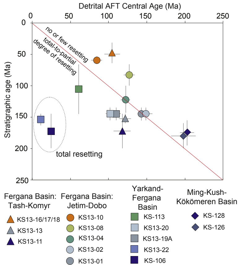
Figure 6. Plot of the detrital AFT results (with error bars) showing the relation between the central AFT age and stratigraphic age for each detrital sample. The red line indicates the 1:1 relationship between the vertical and horizontal axis. Extensive burial of the Jurassic samples of the Yarkand-Fergana Basin (e.g. KS-106 and KS13-22) below the AFT total annealing zone caused total resetting of the AFT age system. The Jurassic samples of the Ming-Kush-Kökömeren Basin plot on the right side of the red 1:1 line, indicating that the AFT age system of these samples are (almost) not reset due to post-depositional burial.
