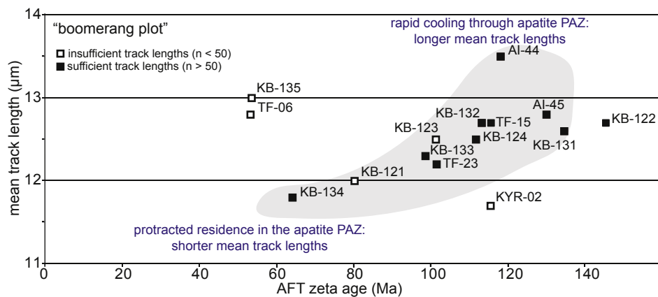
Figure 7. Boomerang plot (Green et al., 1986) on which the new basement AFT data of samples of the Northern Tien Shan and Middle Tien Shan are plotted. The mean track length and mean zeta age are displayed on the vertical and horizontal axis, respectively. Samples with sufficient track length data ( n > 50 ) are displayed as full squares, while the samples with insufficient track length data ( n < 50 ) are displayed as open squares. The boomerang plot expresses the relation between AFT age and mean track length, indicative for cooling rate through the apatite partial annealing zone. Rapid basement cooling (130–100 Ma) through the apatite partial annealing zone is characterized by higher mean track lengths. Lower track lengths are characteristic for samples with an AFT age between 100 and 65 Ma, which indicates that these samples experienced a protracted cooling through the apatite partial annealing zone.
