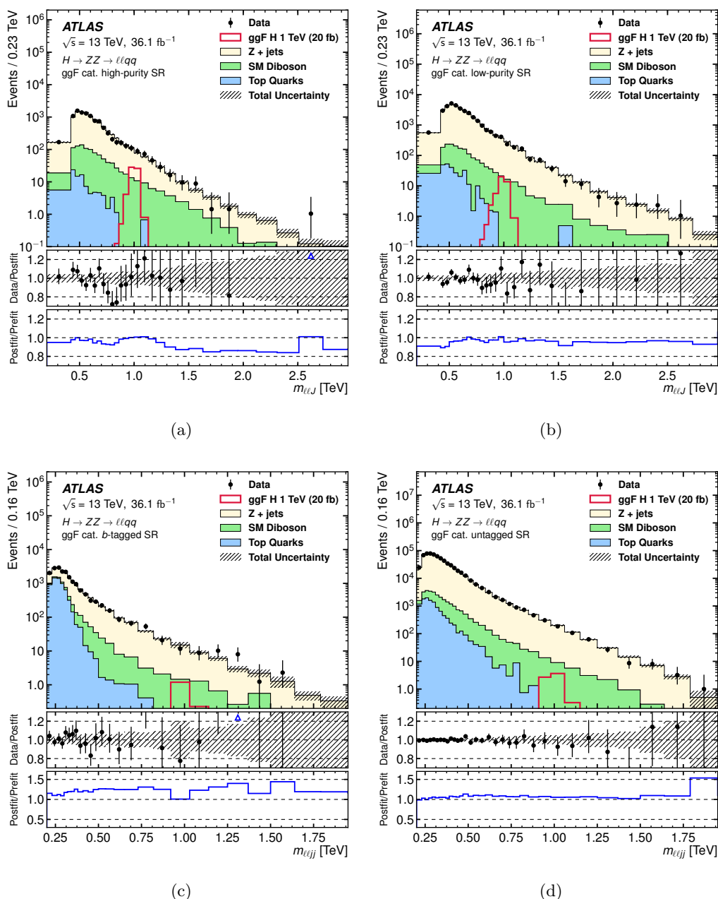
Figure 8. Comparisons of the observed data and expected background distributions of the final discriminants of the ggF category for the H \rightarrow ZZ \rightarrow \ell\ell q\bar{q} search: m_{\ell\ell J} of (a) high-purity and (b) low-purity signal regions; m_{\ell\ell jj} of (c) b -tagged and (d) untagged signal regions. For illustration, expected distributions from the ggF production of a 1 TeV Higgs boson with \sigma \times \mathcal{B}(H \rightarrow ZZ) = 20 \text{ fb} are also shown. The middle panes show the ratios of the observed data to the background predictions. The uncertainty in the total background prediction, shown as bands, combines statistical and systematic contributions. The blue triangles in the middle panes indicate bins where the ratio is nonzero and outside the vertical range of the plot. The bottom panes show the ratios of the post-fit and pre-fit background predictions.
