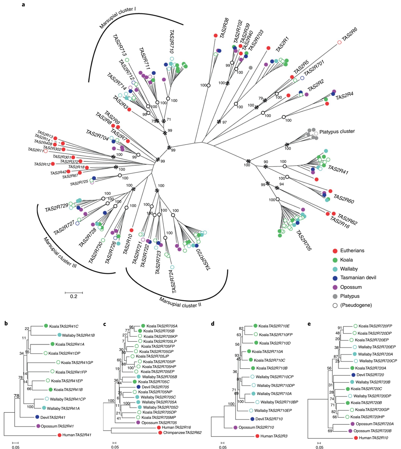
Fig. 2 | Taste receptor analysis in koalas and other mammals identifies three marsupial-specific expansions and further koala-specific duplications.
