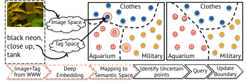
Figure 1: The sequence of steps in our approach: first three blocks (in dashed red) are done once and the last three are performed iteratively. The semantic space is found using the deep representations where semantic concepts are clustered (clothes, military and aquarium in this example). Subsequently, the algorithm queries the uncertain points (in red circles) at each iteration and updates the decision boundary of the classifier (black dashed lines).
