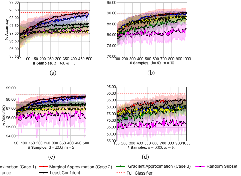
Figure 2: Results from running our approach on ImageNet dataset. Through active labelling using a fraction of images, we are able to perform comparably to the full classifier trained on the fully labelled dataset (in dashed line). As shown, lower dimension of the semantic space shows better improvement with each new observation. Our approaches are also consistently better than choosing a random subset.
