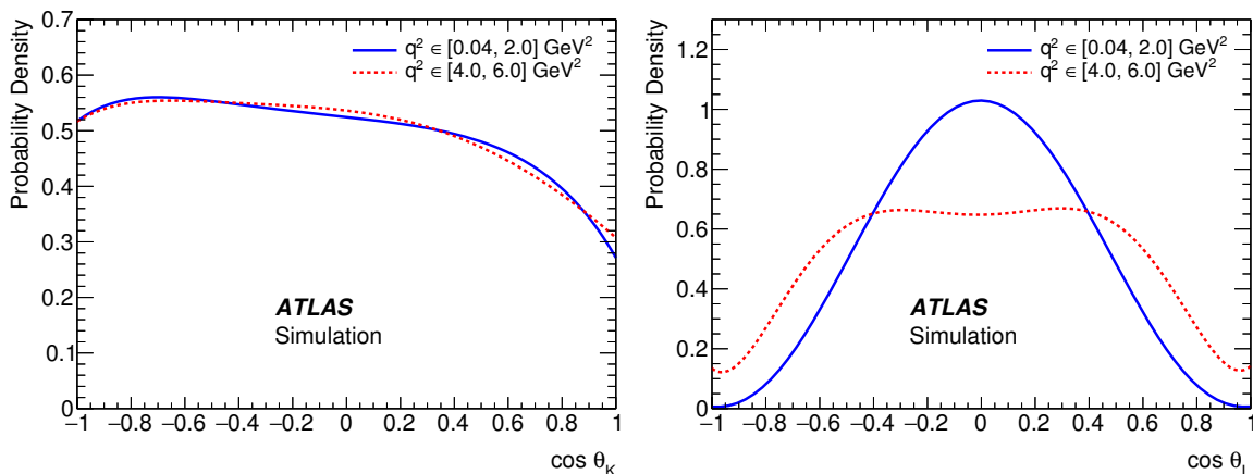
Figure 2. The acceptance functions for (left) \cos \theta_K and (right) \cos \theta_L for (solid) q^2 \in [0.04, 2.0] \text{ GeV}^2 and (dashed) q^2 \in [4.0, 6.0] \text{ GeV}^2 , that shape the angular decay rate of equation (2.1).
