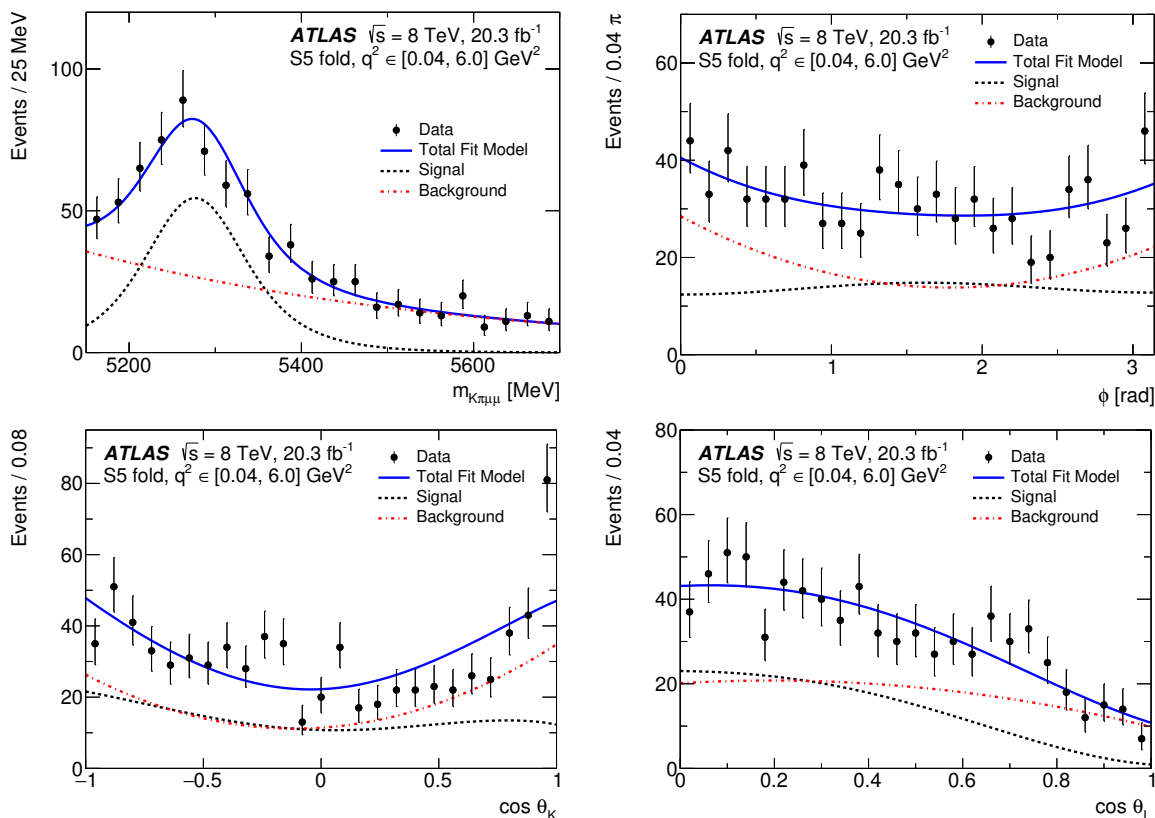
Figure 9. The distributions of (top left) m_{K^*\pi\mu\mu} , (top right) \phi , (bottom left) \cos \theta_K , and (bottom right) \cos \theta_L obtained for q^2 \in [0.04, 6.0] \text{ GeV}^2 . The (blue) solid line is a projection of the total pdf, the (red) dot-dashed line represents the background, and the (black) dashed line represents the signal component. These plots are obtained from a fit using the S_5 folding scheme.
