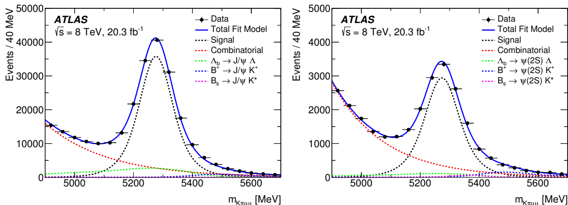
Figure 3. Fits to the K\pi\mu\mu invariant mass distributions for the (left) K^*J/\psi and (right) K^*\psi(2S) control region samples. The data are shown as points and the total fit model as the solid lines. The dashed lines represent (black) signal, (red) combinatorial background, (green) \Lambda_b background, (blue) B^+ background and (magenta) B_s^0 background components.
