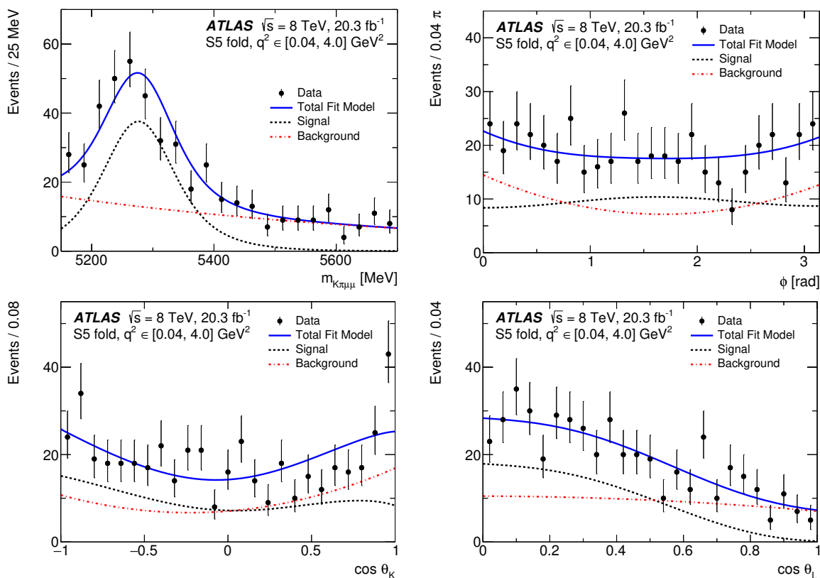
Figure 7. The distributions of (top left) m_{K\pi\mu\mu} , (top right) \phi , (bottom left) \cos\theta_K , and (bottom right) \cos\theta_L obtained for q^2 \in [0.04, 4.0] \text{ GeV}^2 . The (blue) solid line is a projection of the total pdf, the (red) dot-dashed line represents the background, and the (black) dashed line represents the signal component. These plots are obtained from a fit using the S_5 folding scheme.
