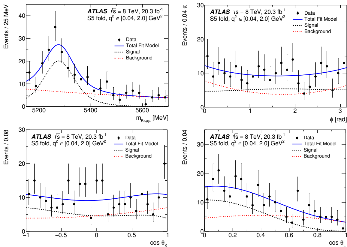
Figure 4. The distributions of (top left) m_{K\pi\mu\mu} , (top right) \phi , (bottom left) \cos\theta_K , and (bottom right) \cos\theta_L obtained for q^2 \in [0.04, 2.0] GeV 2 . The (blue) solid line is a projection of the total pdf, the (red) dot-dashed line represents the background, and the (black) dashed line represents the signal component. These plots are obtained from a fit using the S_5 folding scheme.
