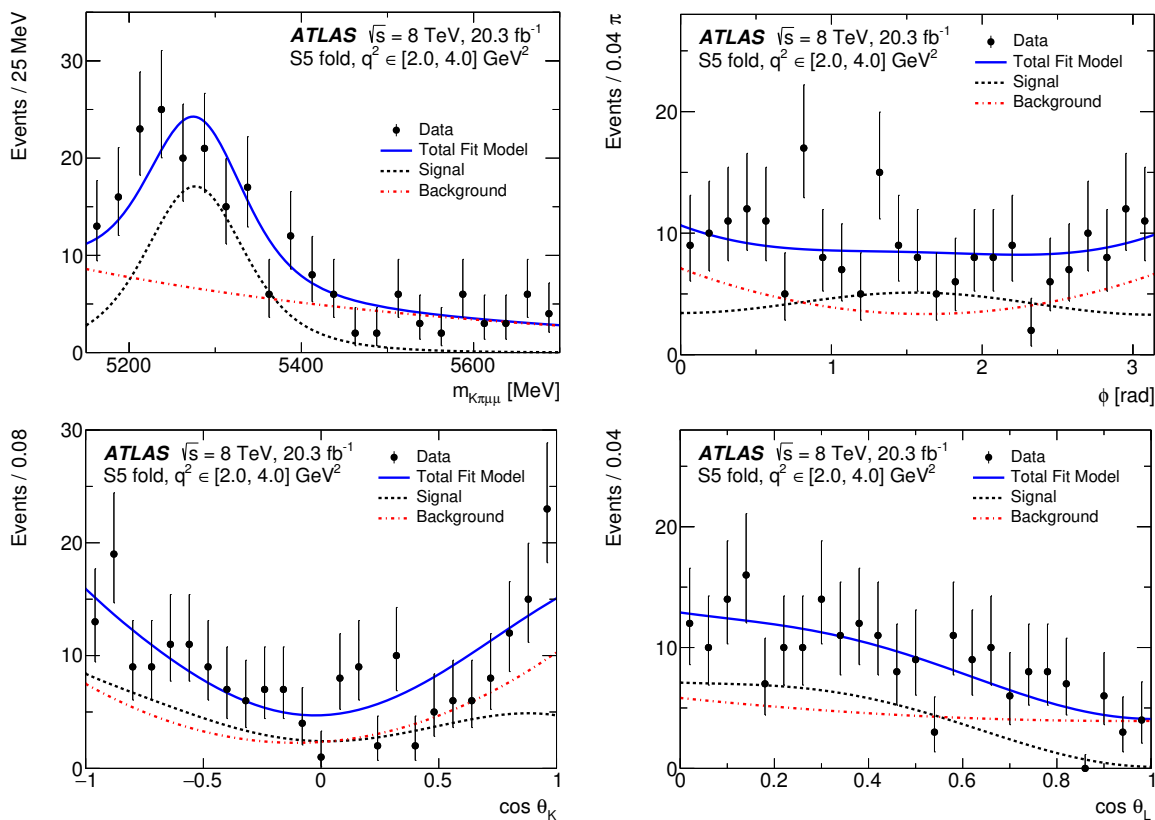
Figure 5. The distributions of (top left) m_{K\pi\mu\mu} , (top right) \phi , (bottom left) \cos\theta_K , and (bottom right) \cos\theta_L obtained for q^2 \in [2.0, 4.0] \text{ GeV}^2 . The (blue) solid line is a projection of the total pdf, the (red) dot-dashed line represents the background, and the (black) dashed line represents the signal component. These plots are obtained from a fit using the S_5 folding scheme.
