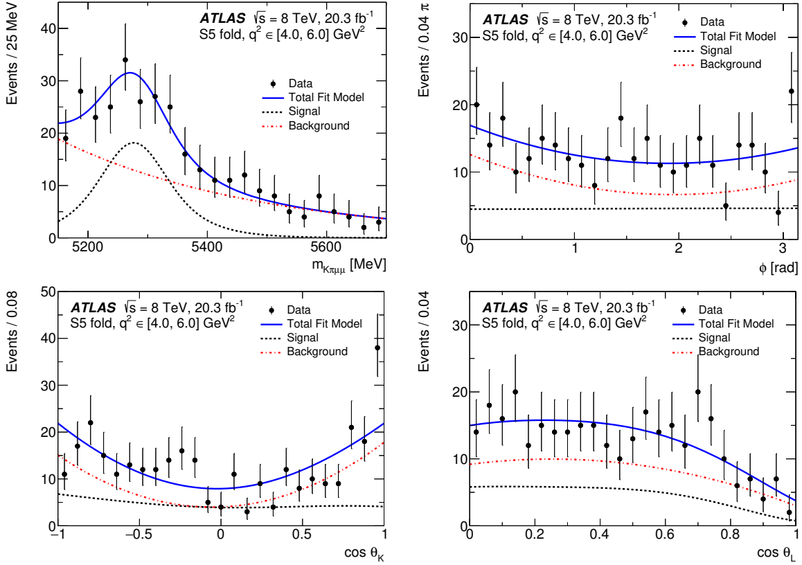
Figure 6. The distributions of (top left) m_{K\pi\mu\mu} , (top right) \phi , (bottom left) \cos\theta_K , and (bottom right) \cos\theta_L obtained for q^2 \in [4.0, 6.0] \text{ GeV}^2 . The (blue) solid line is a projection of the total pdf, the (red) dot-dashed line represents the background, and the (black) dashed line represents the signal component. These plots are obtained from a fit using the S_5 folding scheme.
