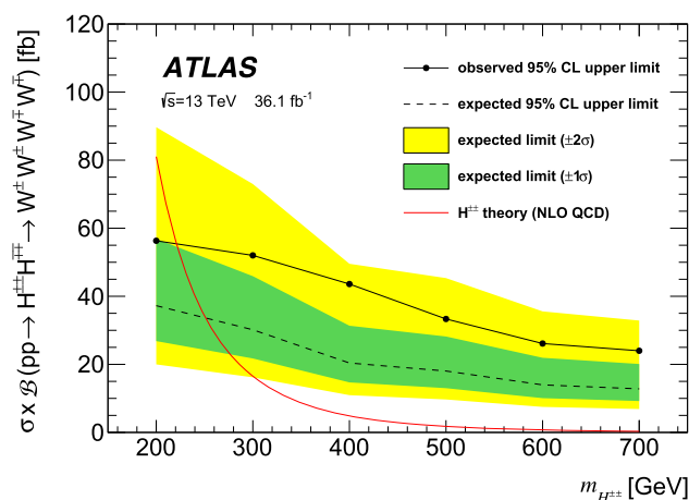
Fig. 5 Observed and expected upper limits for pp \rightarrow H^{\pm\pm} H^{\mp\mp} \rightarrow W^{\pm} W^{\pm} W^{\mp} W^{\mp} cross-section times branching fraction at 95% CL obtained from the combination of 2\ell^{SS} , 3\ell and 4\ell channels. The region above the observed limit is excluded by the measurement. The bands represent the expected exclusion curves within one and two standard deviations. The theoretical prediction [3] including the NLO QCD corrections [33] is also shown and is excluded for m_{H^{\pm\pm}} < 220 GeV
