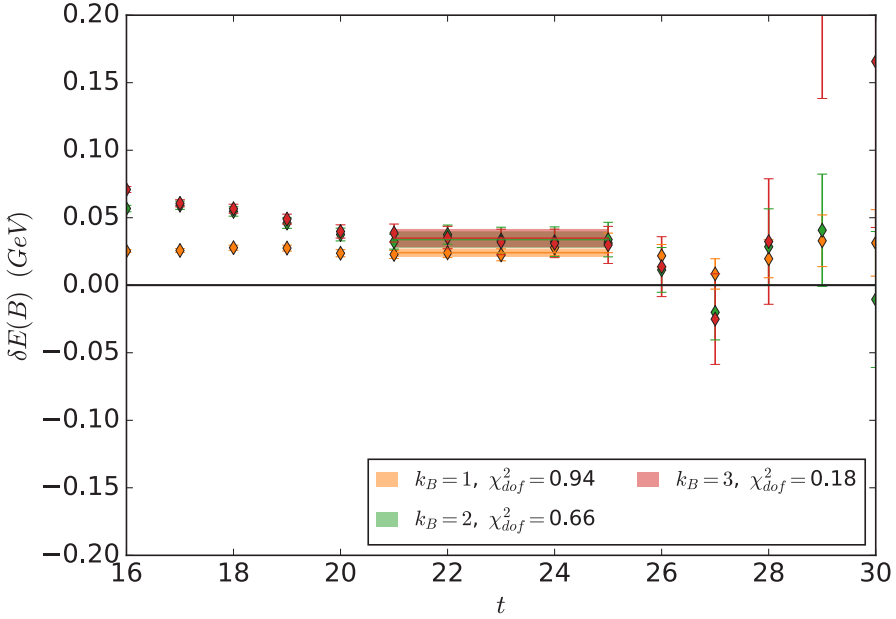
Figure 5. The spin-averaged proton effective energy shift as a function of Euclidean time (in lattice units), obtained using a smeared source and U(1) \times SU(3) eigenmode sink. Results are shown for k_B = 1, 2, 3 (with magnetic field strength increasing away from zero), along with the selected fits and reduced \chi^2 .
