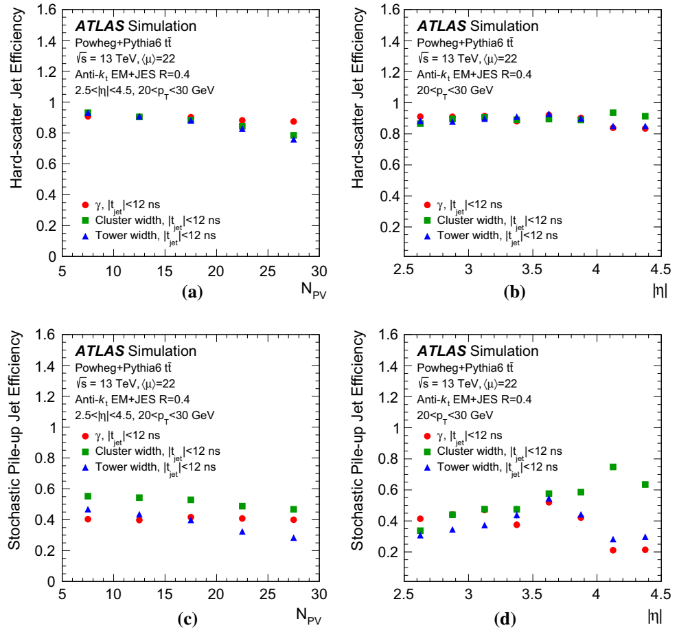
Fig. 10 Hard-scatter jet efficiency as a function of a number of reconstructed primary vertices N_{PV} and b pseudorapidity |\eta| , as well as stochastic pile-up jet efficiency as a function of c number of reconstructed primary vertices N_{PV} and d pseudorapidity |\eta| at 90% efficiency of selecting hard-scatter jets in simulated t\bar{t} events
