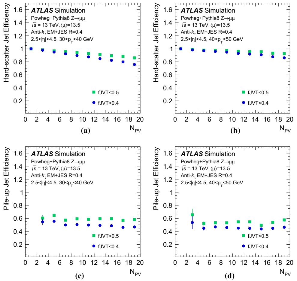
Fig. 16 Efficiency in simulated Z+jets events as a function of N_{PV} for hard-scatter forward jets with a 30 \text{ GeV} < p_T < 40 \text{ GeV} and b 40 \text{ GeV} < p_T < 50 \text{ GeV} , and for pile-up forward jets with c 30 \text{ GeV} < p_T < 40 \text{ GeV} d 40 \text{ GeV} < p_T < 50 \text{ GeV}
