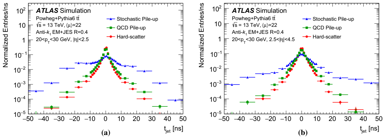
Fig. 5 Distribution of the jet timing t_{jet} for hard-scatter, QCD pile-up and stochastic pile-up jets in the a central and b forward region
