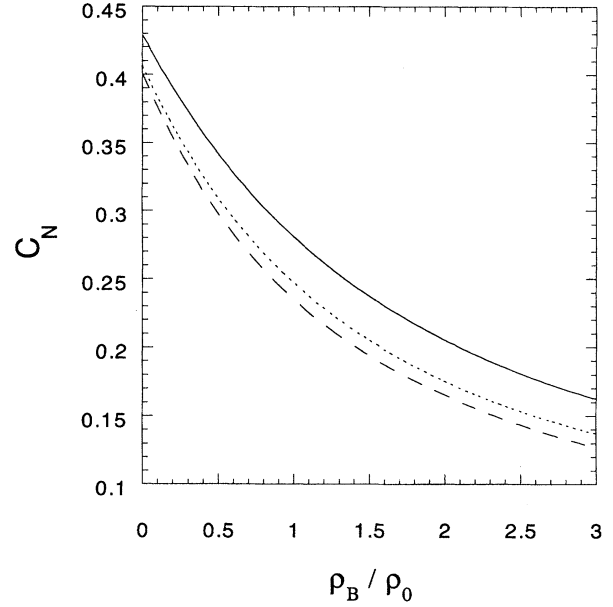
FIG. 1. Quark-scalar density for various bag radii ( R_0 ) as a function of \rho_B . The solid, dotted and dashed curves show C_N for R_0 = 0.6, 0.8 , and 1.0 fm, respectively. The quark mass is chosen to be 5 MeV.
