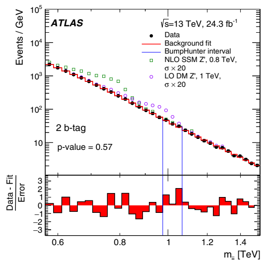
(c) Two b -tag, low mass
