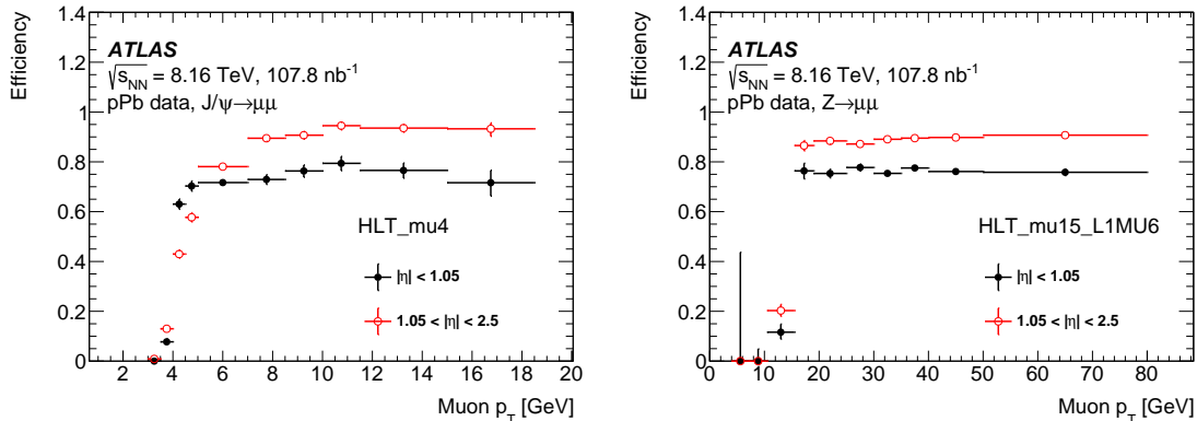
Figure 24. Low- p_T (left) and high- p_T (right) trigger efficiency as a function of the muon p_T in the barrel region (full black circles) and in the endcap region (empty red circles) in p+Pb collision data. The error bars show the statistical uncertainties only.
