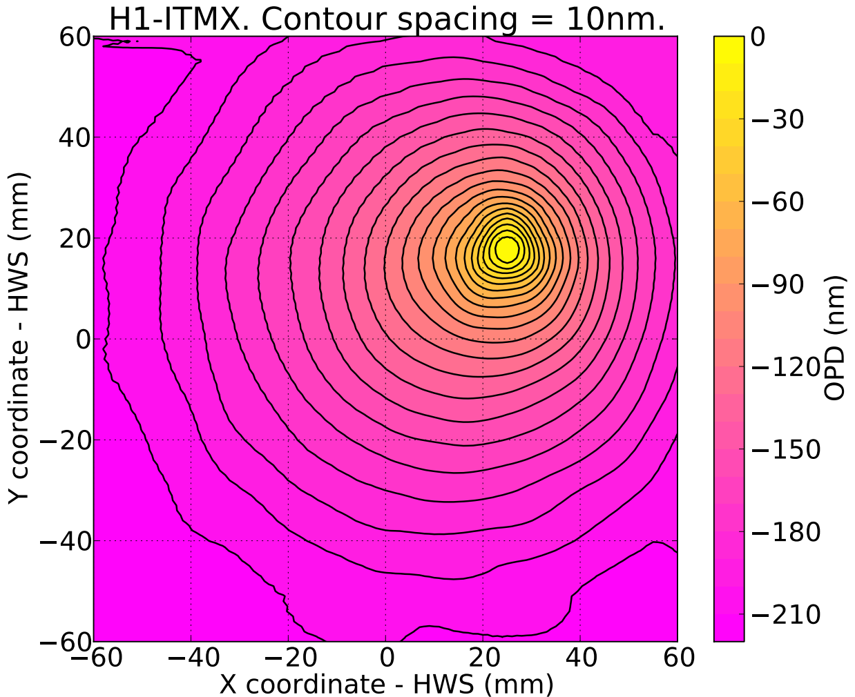
FIG. 2. Hartmann sensor measurement of optical path distortion (thermo-refractive plus thermo-elastic) from a single point absorber on H1-ITMX. Cold reference taken at GPS time: 1180 229 513 s, hot measurement taken 3322 s later at GPS time: 1180 232 835 s. This measurement corresponds to approximately 27 \pm 2.5 mW power absorbed in the point.
