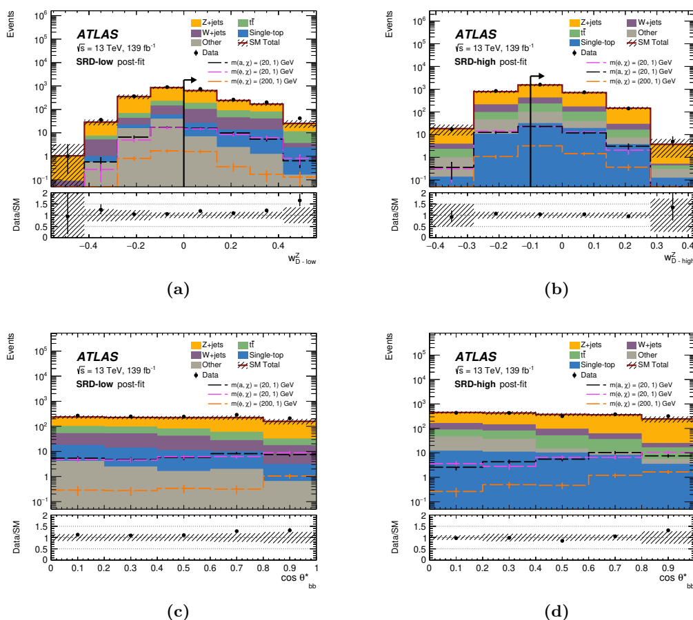
Figure 7. Post-fit distribution of (a) w_{D\text{-low}}^Z and (c) \cos\theta_{bb}^* in SRD-low and (b) w_{D\text{-high}}^Z and (d) \cos\theta_{bb}^* in SRD-high. Where relevant, the signal region selection is indicated by a black arrow. In each of (a)–(d) the lower plot shows the ratios of the observed yields to the post-fit predicted background yields. The “Other” category includes contributions from diboson and t\bar{t} + W/Z/H production. The shaded band represents the total uncertainty of the background prediction. The last bin includes the overflow events.
