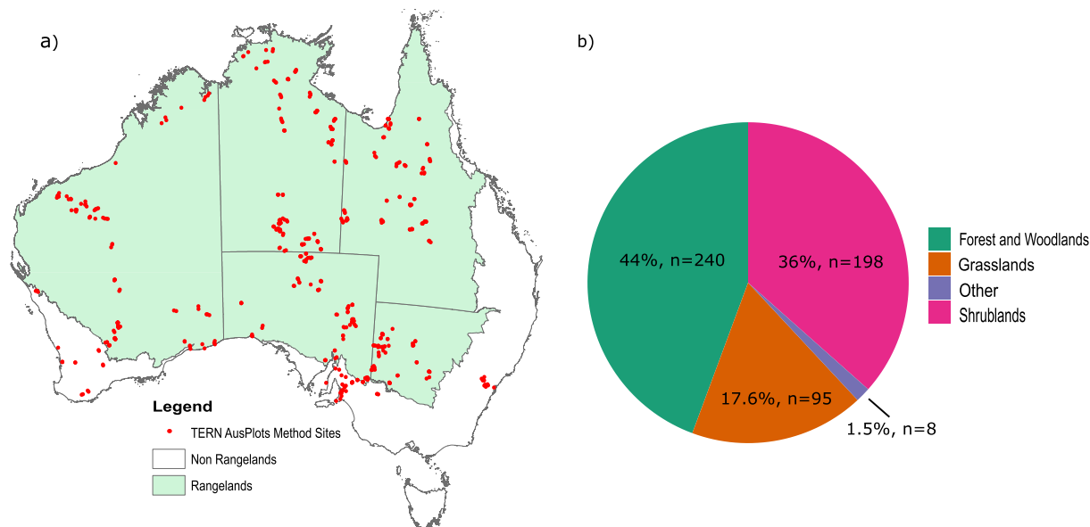
Fig. 1 (a) Location of TERN Ecosystem Surveillance plots surveyed using the AusPlots Rangelands method from 2011–2017. Areas in green denote rangeland habitat (b) number (n) and proportion (%) of TERN Ecosystem Surveillance plots grouped by vegetation type.
