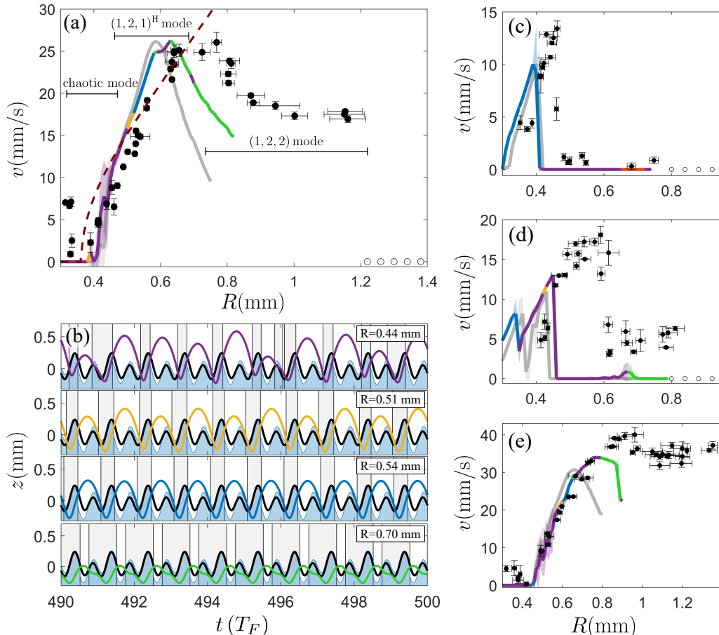
Figure 5: Speed of a superwalker as a function of its size at fixed \Gamma_{80} = 3.8 and \Delta\phi = 130^\circ . (a) Comparison of the speed-size characteristics of a droplet from numerical simulations (solid curves) with experimental results of Valani et al. (2019) (black circles with empty circles indicating coalescence) and the stroboscopic model of Oza et al. (2013) (dashed curve) at \Gamma_{40} = 0.6 . For the stroboscopic model, we set the adjustable parameters of the impact phase and the non-dimensional drag coefficient to \sin(\Phi) = 0.2 and C = 0.17 respectively, while the other parameters were chosen to match the experiments of Valani et al. (2019). The black horizontal bars indicate where different bouncing modes in experiments were observed. Panel (c), (d) and (e) show the speed-size characteristics at \Gamma_{40} = 0 , \Gamma_{40} = 0.3 and \Gamma_{40} = 1 respectively. In each panel the grey curve is for fixed parameter values of K = 0.70 and B = 0.60 , and multicoloured curve represents when K is varied as a linear function of the droplet radius R according to (2.11) with a fixed B = 0.60 . The colours on this curve represent a chaotic bouncing mode in purple, (2, 4, 2) mode in yellow, (1, 2, 1)^H mode in blue, (1, 2, 1)^L mode in green and (1, 2, 2) mode in red. Termination of the solid curves indicate coalescence. The typical bouncing modes from panel (a) at different droplet radii are shown in panel (b). In this panel, the grey regions indicate times at which the droplet is in contact with the bath.
