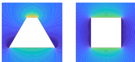
Figure 2: The magnetic field in the z -direction measured across the XZ plane of both a frustum and cube permanent magnet.
