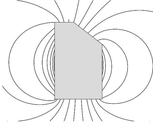
FIGURE 2.2: The magnetic flux lines of the polyhedral magnet shown in Figure 2.1. The flux lines travel from the north pole (top) of the magnet to the south pole (bottom) of the magnet. The flux lines behave similarly to that of a cuboidal magnet in most regions due to the magnet being almost cuboidal. However, in the top right region, the flux lines differ from those of a cuboidal magnet due to the chamfer.
