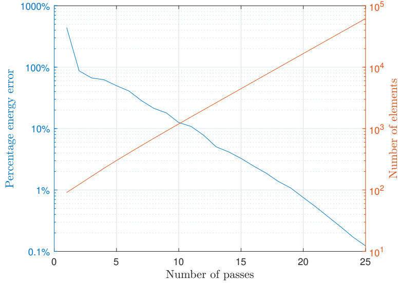
FIGURE 5.4: Percentage energy error and number of tetrahedral elements in the ANSYS Maxwell simulation for d = 0.5 as the number of passes of automatic mesh generation is increased.
