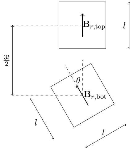
FIGURE 5.6: Two cube magnets with a side length of l maintaining a constant distance of 3l/2 between their centres. The force and torque on the bottom magnet is calculated as it is rotated an angle \theta about its centre.
