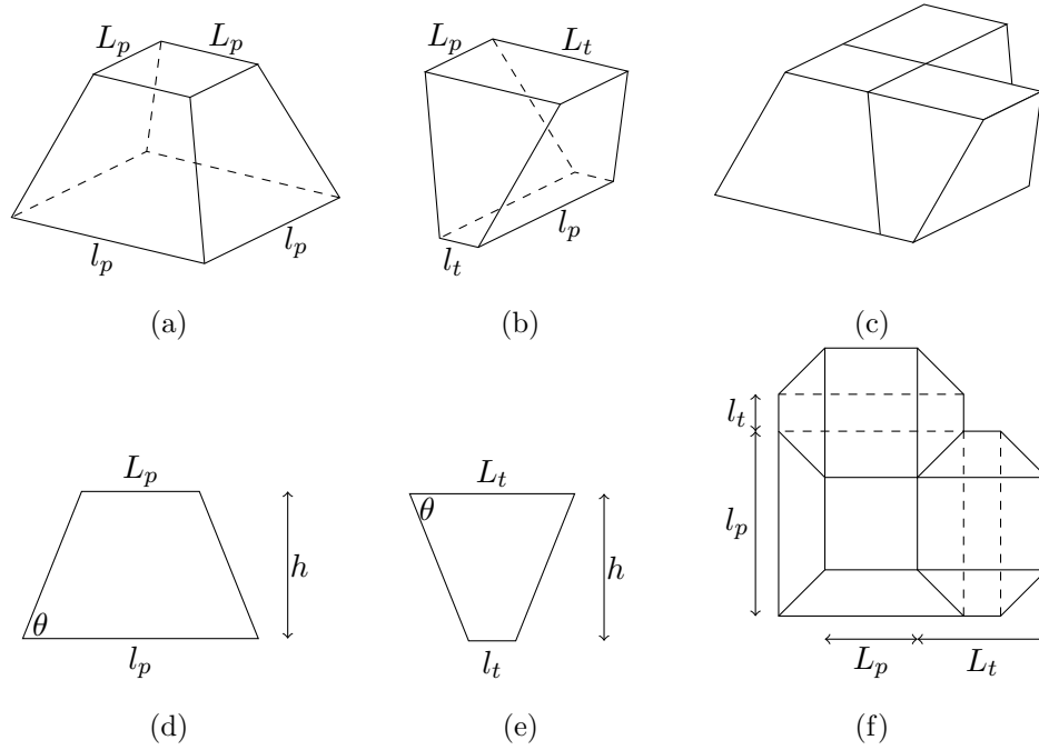
FIGURE 4.10: Three dimensional views and schematics of a pyramid frustum (a,d), a tetrahedral frustum (b,e), and the repeating unit (c,f).
