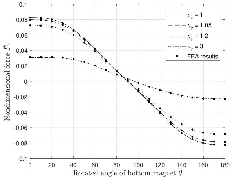
FIGURE 5.10: Nondimensional vertical force F_V on the bottom magnet as it rotates for varying relative permeabilities \mu_r . Finite element results are depicted using large dots, indicating strong agreement with the results using the above methodology.
