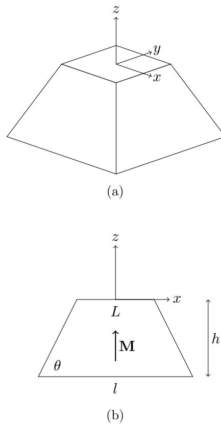
FIGURE 4.4: Three-dimensional view (a) and schematic (b) of a right square pyramid frustum permanent magnet with magnetisation vector \mathbf{M} . The origin is located at the centre of the top surface and both rectangular surfaces are parallel to the XY -plane. The frustum has a nondimensional height h , a top surface side length L , and bottom surface side length l . The four angled surfaces form an angle \theta with the bottom surface.
