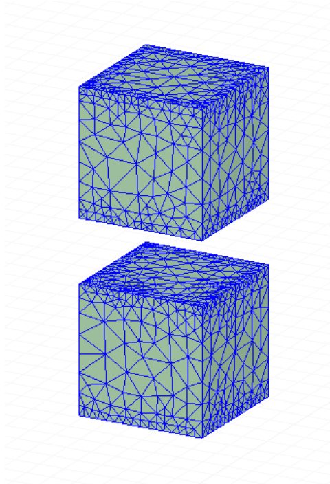
FIGURE 5.3: The mesh generated by ANSYS Maxwell after 25 passes of automatic mesh refinement for the magnetic configuration shown in Figure 5.2. This mesh uses approximately 58,000 tetrahedral elements with quadratic shape functions, with approximately 4,500 elements per magnet and 49,000 elements in the region between and around the magnets.
