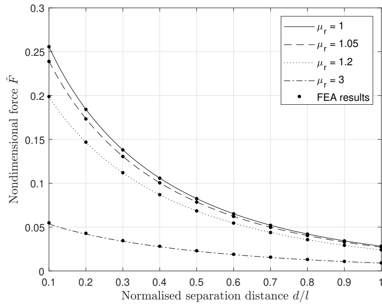
FIGURE 5.5: Nondimensionalised force between the two magnets in Figure 5.2 for \mu_r = 1 (calculated using [1]), \mu_r = 1.05 , \mu_r = 1.2 , and \mu_r = 3 . The forces calculated using the methodology presented in this paper are denoted with lines, with finite element simulations represented with large dots. The methodology presented above is in strong agreement with the finite element simulations, indicating correct force results.
