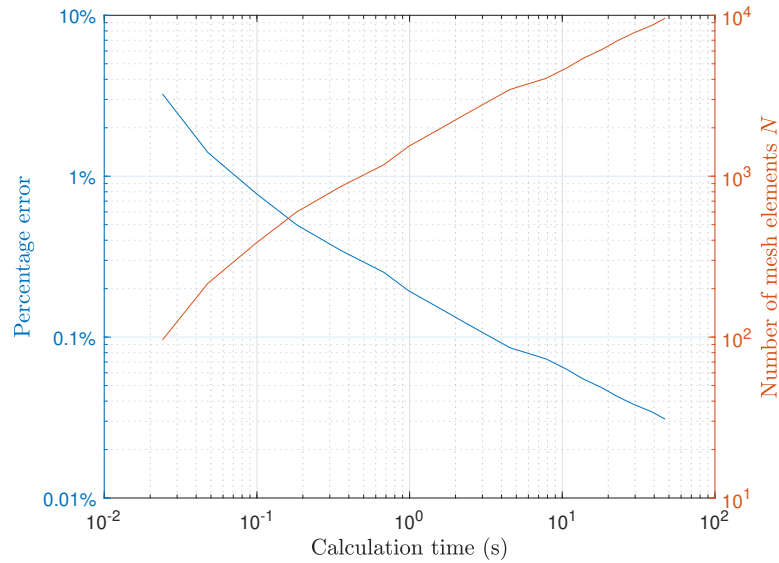
FIGURE 5.13: Percentage error in the calculation of vertical force F_V between the magnets shown in Figure 5.2 with d = l and \mu_r = 1 as mesh density, and thus calculation time, is increased. The number of surface mesh elements N is also plotted, showing an inverse trend when compared to the percentage error.
