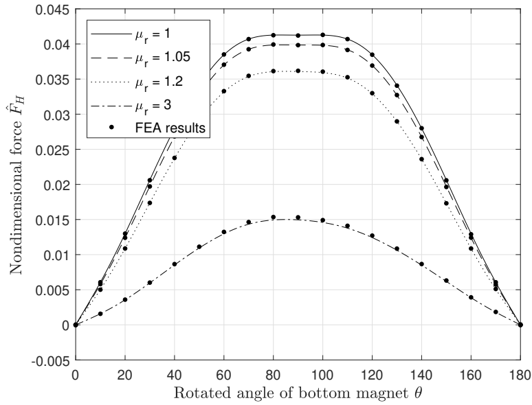
FIGURE 5.9: Nondimensional horizontal force F_H on the bottom magnet as it rotates for varying relative permeabilities \mu_r . Finite element results are depicted using large dots, indicating strong agreement with the results using the above methodology.
