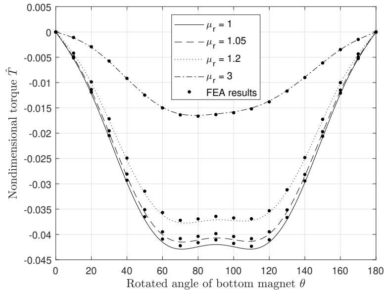
FIGURE 5.8: Nondimensional torque on the bottom magnet about the axis of rotation of the magnet as it rotates for varying relative permeabilities \mu_r . Finite element results are depicted with large dots, indicating some agreement with the results using the above methodology, with the FEA results being approximately 2% smaller in magnitude for low permeabilities.
