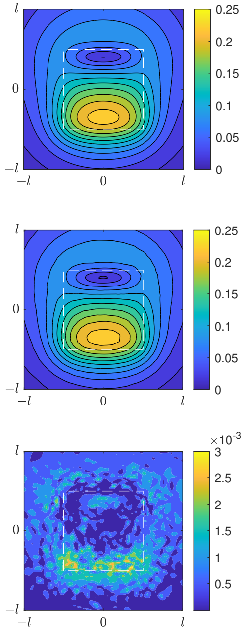
FIGURE 5.12: The magnetic field strength |\mathbf{B}| normalised by B_r on the plane between the two magnets in Figure 5.6 when \theta = 90^\circ . The projections of the magnets onto the plane are displayed using white dashed lines. The field was calculated using the methodology in this paper (top) and finite element simulations (middle), with the absolute error between the two calculated (bottom). This shows strong agreement, with a maximum error of 0.3% of the remanence magnetisation.
