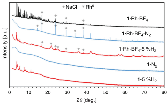
Fig. 4. PXRD patterns of 1 -Rh-BF 4 as-synthesised and samples resulting from the thermal treatment of 1 and 1 -Rh-BF 4 samples. Samples reduced (red) and calcined (blue) as indicated in labels.
