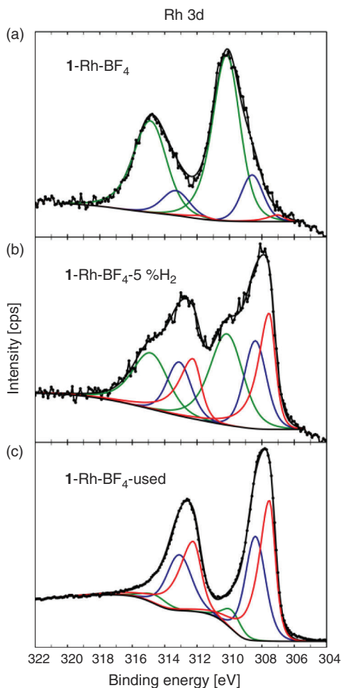
Fig. 10. (a) Selected, representative high-resolution Rh 3d spectra of 1 -Rh-BF 4 , (a) as synthesised; (b) after heat treatment in 5% H 2 ; and (c) after CO 2 hydrogenation catalysis testing. The red doublets were assigned to Rh 0 , blue for both Rh I and Rh III , and green for Rh III (see Supplementary Material). Peak assignments for Rh I and Rh III from the literature were used for peak assignment as detailed in Table S4 (Supplementary Material).
