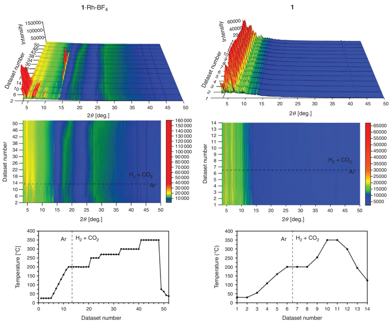
Fig. 5. In situ PXRD study for 1 -Rh-BF 4 and 1 . Diffractograms are stacked according to dataset number and colours are indicative of intensity. Dashed lines designate change in sample atmosphere composition. Temperature profile during experiment is displayed at the bottom.
