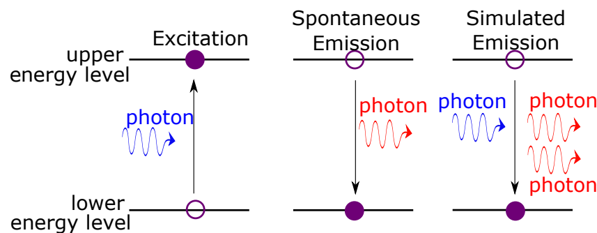
Figure 4.4: ( left ) Excitation of an electron from a low to higher energy level due to absorption of energy from a photon. ( middle ) The emission of a photon when an electron spontaneously decays to a lower energy level. ( right ) An incident photon interacts with an excited atom, causing the electron to decay to a lower energy level and emit a photon.
