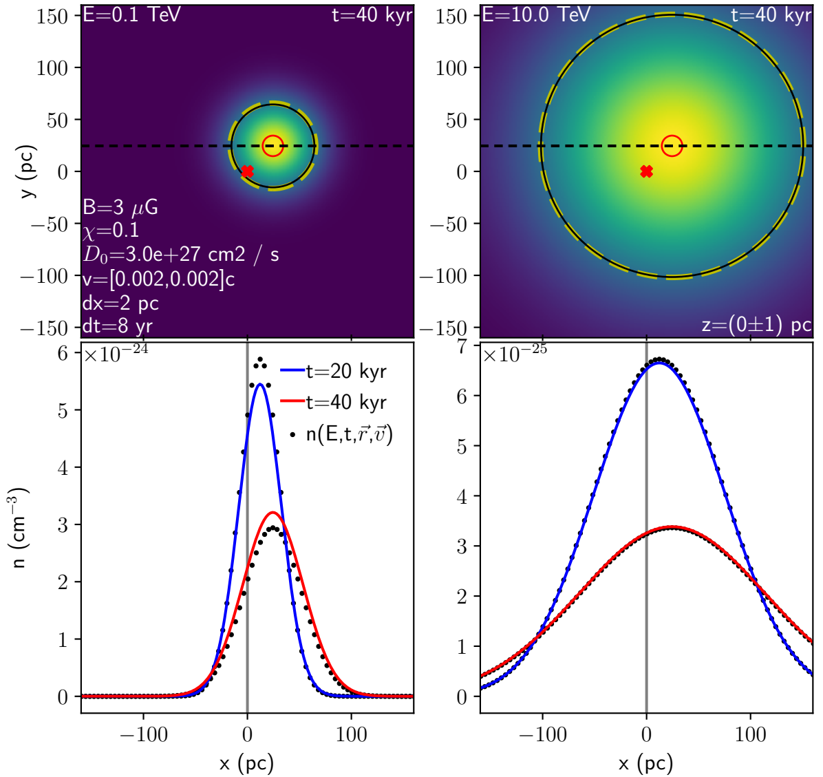
Figure 7.11: Electron injection into a 2D grid at x = y = t = 0 and experiencing diffusion and advection with v = [0.002c, 0.002c] . ( Top ) The number density distribution after 40 kyr. The black and yellow dashed circles represent the 2D variance radius ( R_{\text{var}} ) and the radius containing 1\sigma = 68\% of electrons ( R_{\sigma} ) respectively. The red circle describes the R_{\sigma} containment radius for an advection-only scenario. Finally, the red cross represents the electron source position at x = y = 0 ( Bottom ) Comparing the numerical solution (lines) and analytical solution (dots, see Eq. 7.36 ) at t = 20 and 40 kyr along y = (vt \pm 1) pc (dashed horizontal line in the bottom panel). The vertical grey line shows the electron source position at x = 0 .
