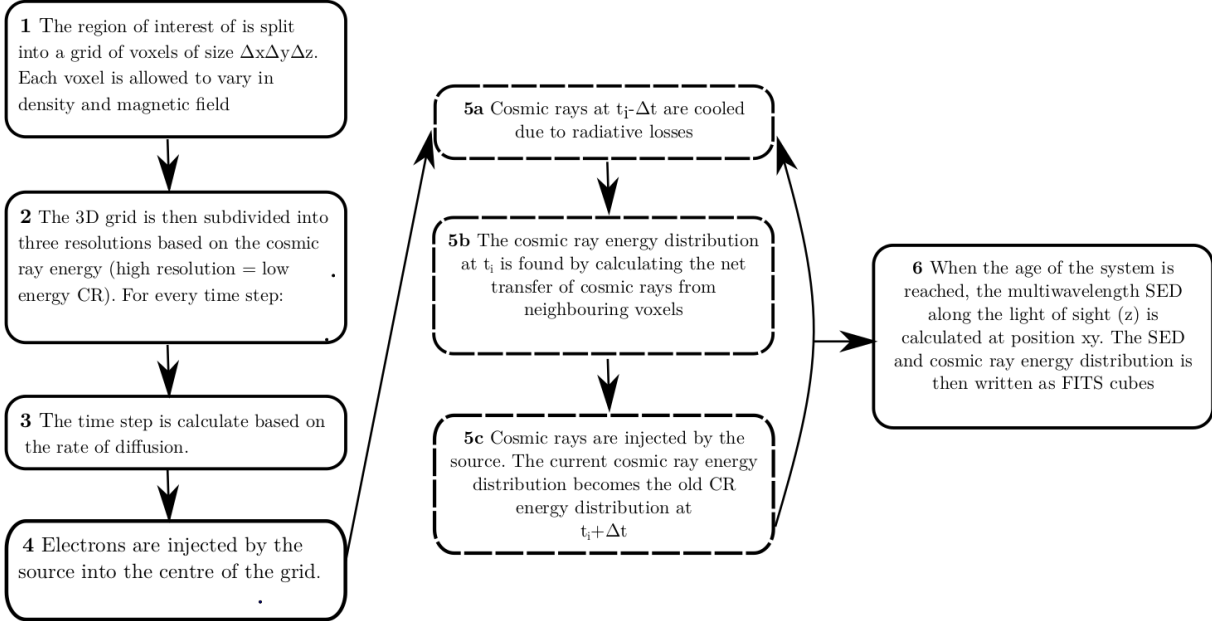
Figure 7.3: A flow-chart description of the steps Multizone uses to calculate the electron energy distribution and subsequent SED by numerically solving the transport equation.
