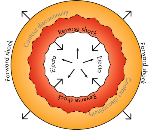
Figure A.2: Illustration of the forward and reverse shocks of a SNR in its Sedov-Taylor phase of its evolution. Image courtesy of Vink, 2020
