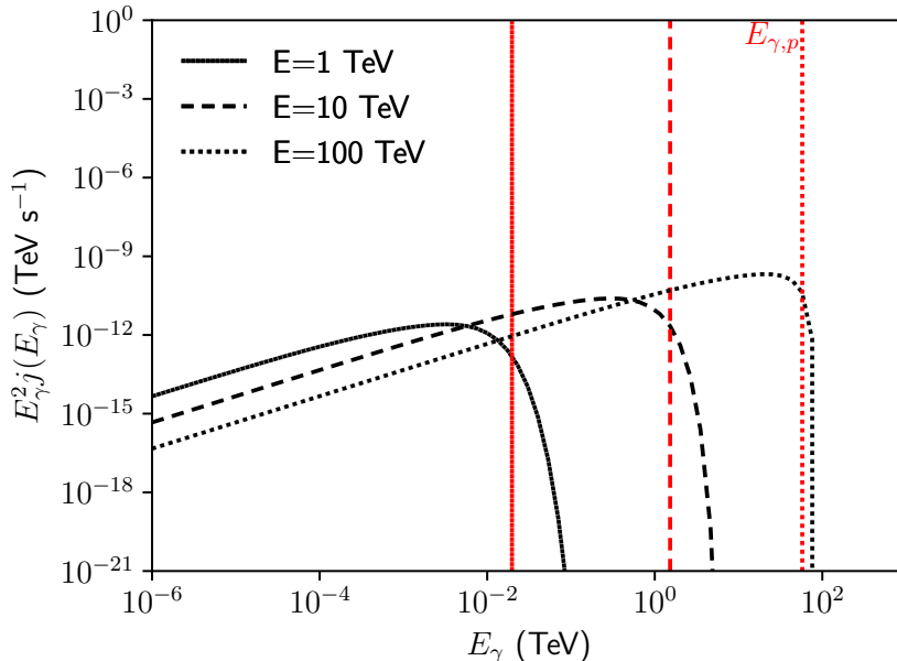
Figure 2.18: IC spectrum from an electron of energy E interacting with the CMB. The red vertical lines represent the energy at which the inverse Compton emission approximately peaks assuming a CMB photon has energy \approx 7 \times 10^{-4} eV.
