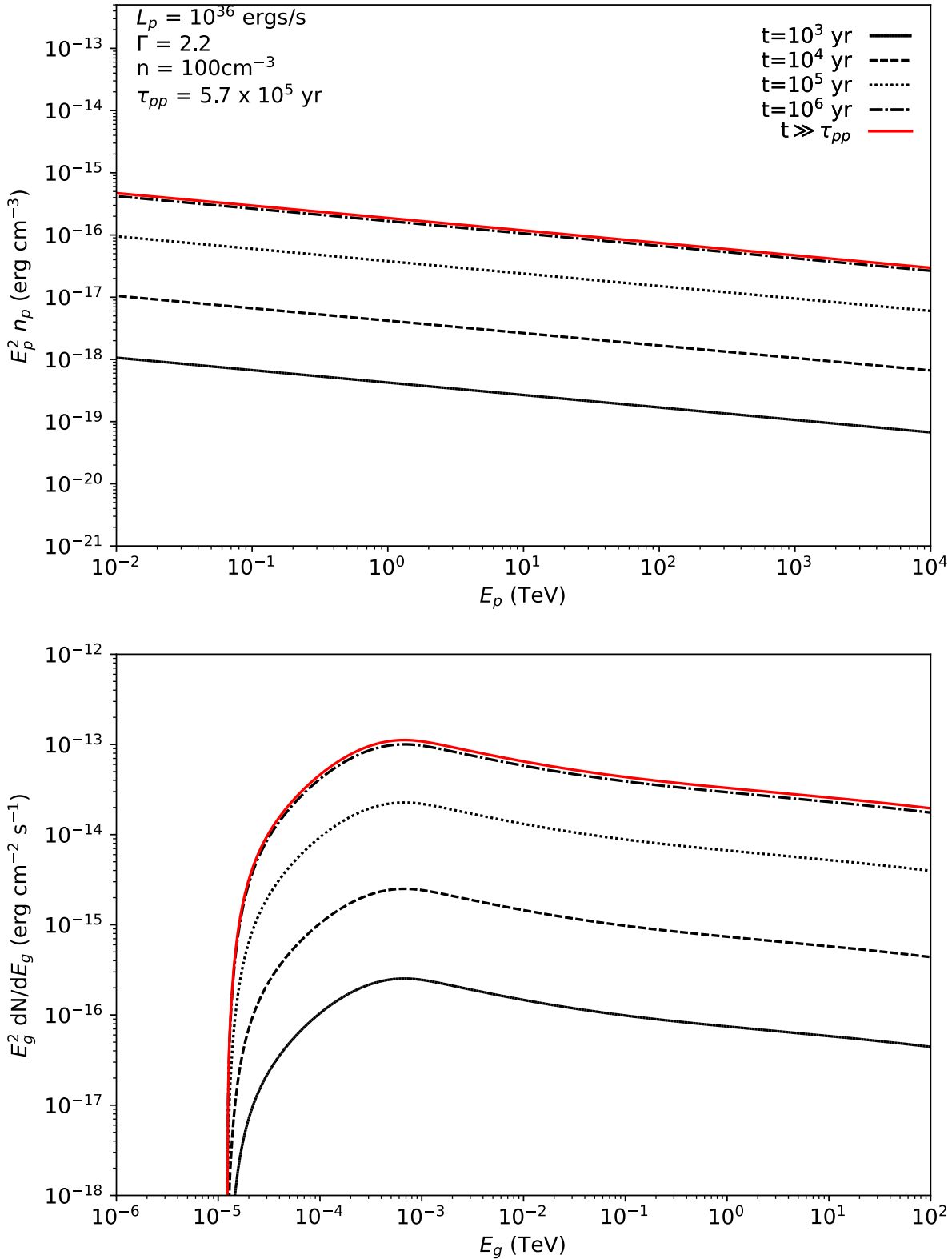
Figure 5.3: Evolution of the cosmic-ray energy density distribution (top) and subsequent gamma-ray spectrum (bottom) for a continuous source injecting protons following a power law spectrum as given by Eq. 5.29. The steady state ( t \gg \tau_{pp} , see Eq. 5.30) is represented by the solid red line. L_p is the energy of cosmic rays injected per second into the system.
