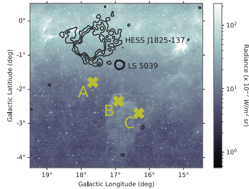
Figure 10. Infrared emission in the 8.26 \mu\text{m} band towards GeV-ABC (Egan, Price & Kraemer 2003). Overlaid are the HESS significance contours towards HESS J1825-137 at 1\sigma , 2\sigma , and 3\sigma (H. E. S. S. Collaboration 2018).
