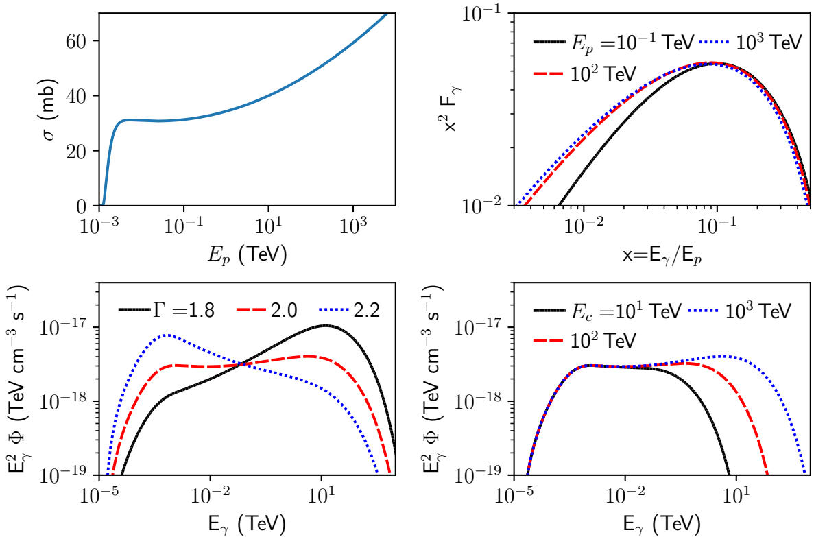
Figure 2.14: ( top-left ) Proton-proton interaction cross section as given by Eq. 2.41. ( top-right ) Hadronic gamma-ray emission from a cosmic-ray proton with energy E_p and target density n_H = 1 \text{ cm}^{-3} ( bottom ) Gamma-ray spectra from p-p interactions from cosmic-rays protons with an exponential cutoff power law distribution ( dN/dE \propto E^{-\Gamma} \exp(-E/E_c) ) with E_c = 10^3 \text{ TeV} ( left ) and \Gamma = 2.0 ( right ).
