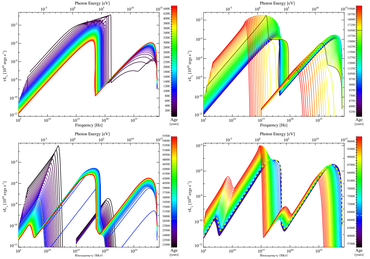
Figure 2.5: Theoretical time evolution of the multi-wavelength SED of a PWN inside a SNR. See text for more information. Image courtesy of Gelfand et al., [2009].
