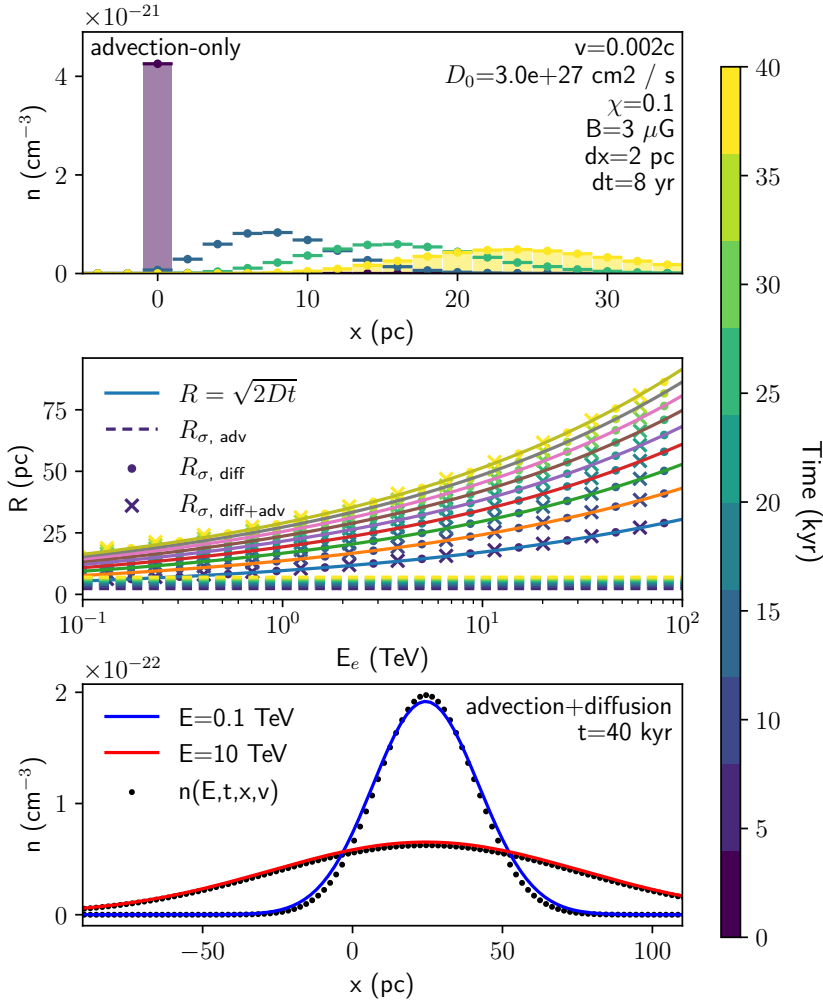
Figure 7.10: Advection and diffusion of the electron number density with velocity v = 0.002c with identical parameters as per Fig. 7.5. (top) Dispersion of electrons for an advection-only scenario. (middle) A comparison of the 1D diffusive variance radius ( R = \sqrt{2Dt} ) and the radius containing 68% of electrons after advection ( R_\sigma ) for an advection-only, diffusion only and diffusion + advection scenarios at different ages of the system. (bottom) The numerical (solid lines) and analytical (dots) electron number density distribution at t = 40 kyr for electron energies E = 0.1 and 10 TeV.
