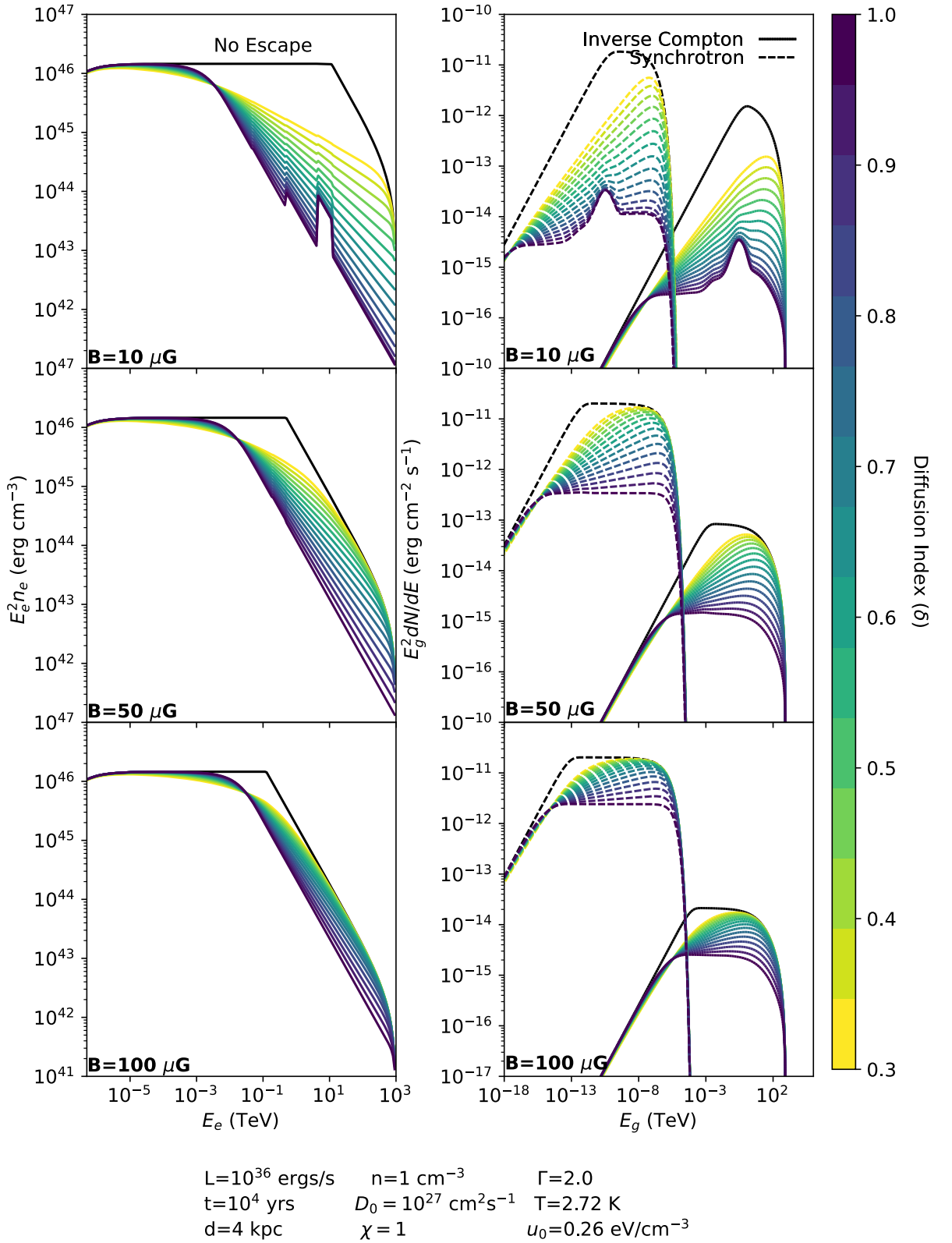
Figure 5.12: Variation of the electron energy density distribution ( left ) and subsequent synchrotron and inverse Compton SED ( right ) for a continuous source of electrons escaping a cloud with radius 10 pc in the different diffusion regimes ( \delta ). Kolmogorov regime: \delta = \frac{1}{3} , Kraichnan regime: \delta = 0.5 and Bohm regime: \delta = 1 . A magnetic field of 10 \mu G ( top ), 50 \mu G ( middle ) and 100 \mu G ( bottom ) was utilised. The black line represents a situation where there is no escape of electrons.
