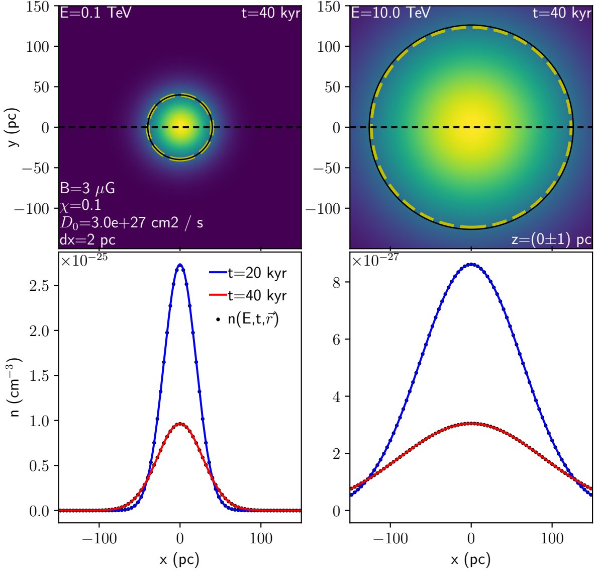
Figure 7.5: Distribution of electrons injected into a 3D grid at x = y = z = t = 0 and subjected to diffusion. ( Top ) The number density distribution taken at slice z = (0 \pm 1) pc and time 40 kyr. The black and yellow dashed circles represent the 2D variance radius ( R_{\text{var}} ) and the radius containing 1\sigma = 68\% of electrons ( R_{\sigma} ) in the 2D slice respectively. ( Bottom ) Comparing the numerical solution (lines) and analytical solution (dots, see Eq. 7.9 ) at t = 20 and 40 kyr along y = (0 \pm 1) pc (dashed horizontal line in the bottom panel).
