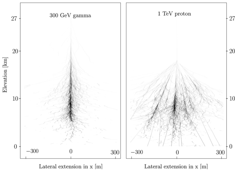
Figure 3.3: Monte Carlo simulations of a air shower triggered by a 0.3 TeV gamma ray ( left ) vs an air shower triggered by a 1 TeV cosmic-ray proton ( right ). Image courtesy of Aharonian et al., 2008
