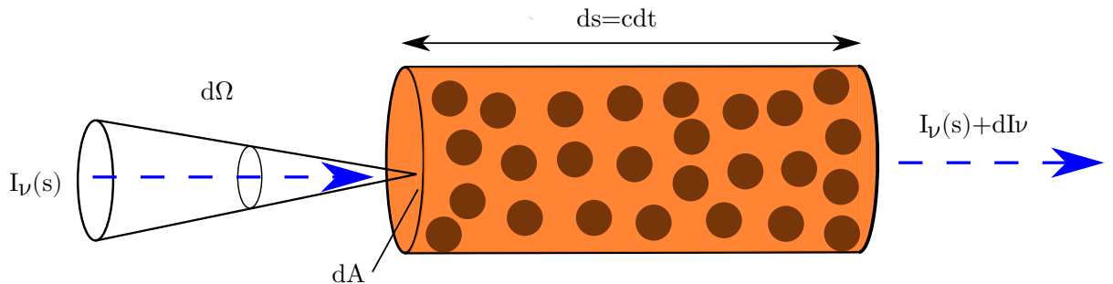
Figure 4.3: A cloud of thickness ds is illuminated by a background source with intensity I_\nu(s) . Photons of frequency \nu are emitted and re-emitted by particles (dark circles) within the cloud, changing the intensity by dI_\nu .
