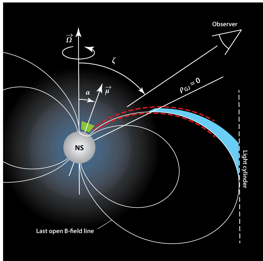
Figure 2.2: Magnetosphere structure of a pulsar with spin velocity \vec{\Omega} at angle \alpha to the magnetic field axis and angle \zeta to the observer. The acceleration site for the polar cap model and outer gap model is shown in green and blue respectively while the site for the slot gap model is enclosed by the red-dashed lines. Image courtesy of Caraveo, 2014.
