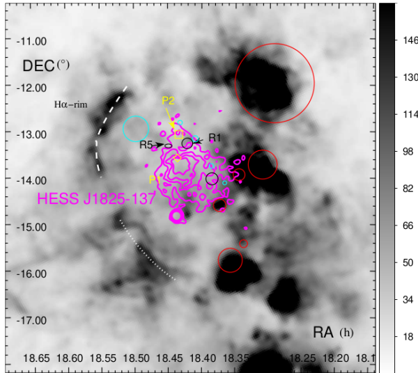
Figure 4.7: H\alpha intensity towards HESS J1825-137. The dashed and dotted lines represent two H\alpha rim-like features associated with the progenitor SNR of HESS J1825-137. Image courtesy of (Voisin et al., 2016)
