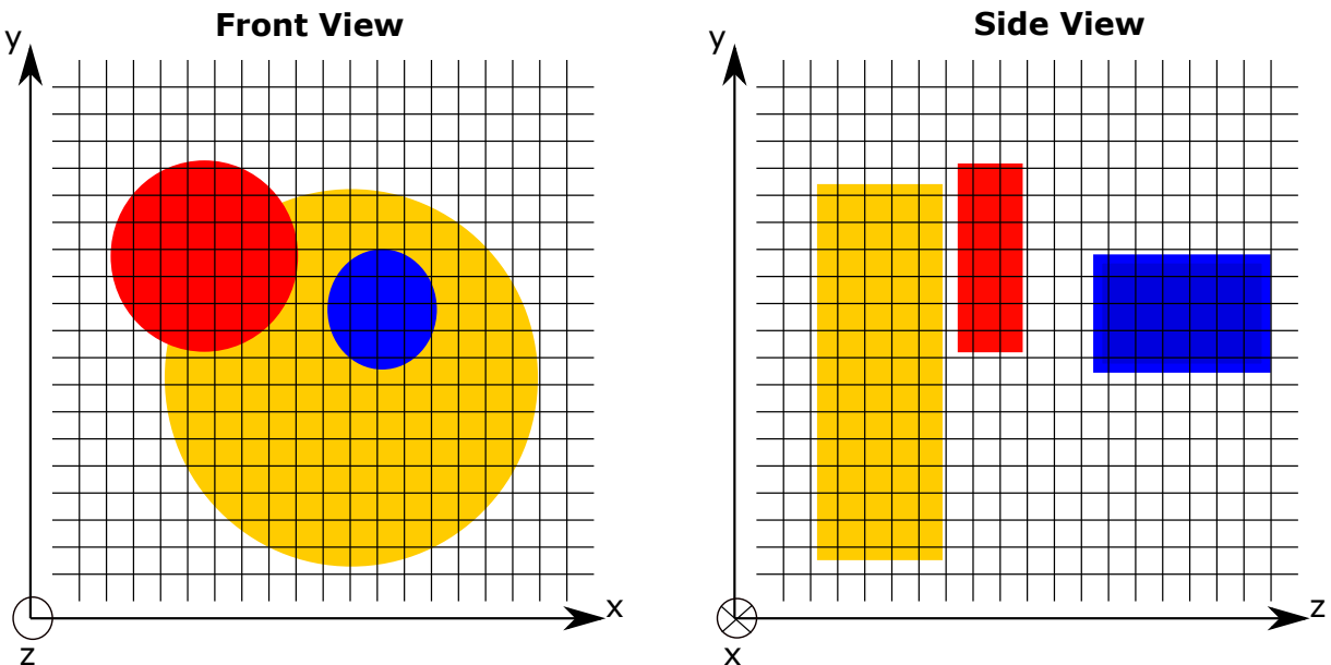
Figure 7.1: Front ( left ) and side ( right ) view of an example region of interest showing three clouds of different densities and sizes. To numerically solve the transport equation, the region of interest is split into a 3D grid of voxels.
