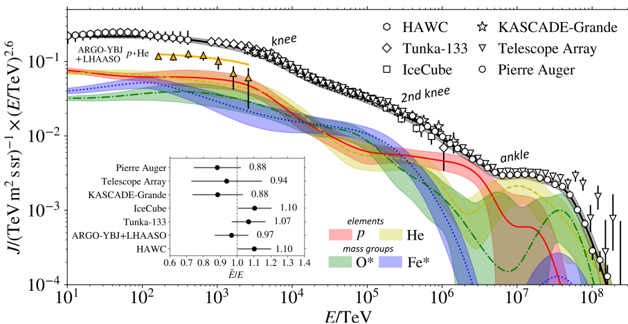
Figure 2.13: Cosmic-ray (and high-energy electron) energy spectrum at Earth as measured by multiple ground-based observatories. Image courtesy of Schroeder et al., [2019]
