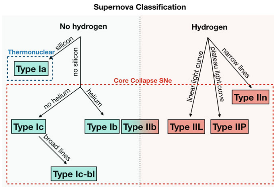
Figure A.1: Supernovae are historically categorised into different classifications based on their absorption line and light curves. Image courtesy of Vink, 2020.
