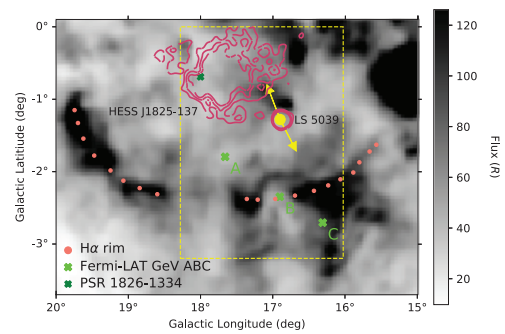
Figure 4. H \alpha emission from the FWHM survey towards HESS J1825-137 and surrounding regions (Finkbeiner 2003). HESS J1825-137 can be seen by \sigma = 1, 2, and 3 purple TeV contours with PSR J1826-1334 represented by the dark green cross and LS-5039 by the yellow dot lying to the lower right with yellow radio jets described by Paredes et al. (2002). GeV regions GeV-A, GeV-B, and GeV-C can be seen as green neon crosses. The H \alpha rims noted by Stupar, Parker & Filipovic (2008) and Voisin et al. (2016) are shown by pink dots. A closer look at the region contained within yellow box is shown in Fig. 5.
