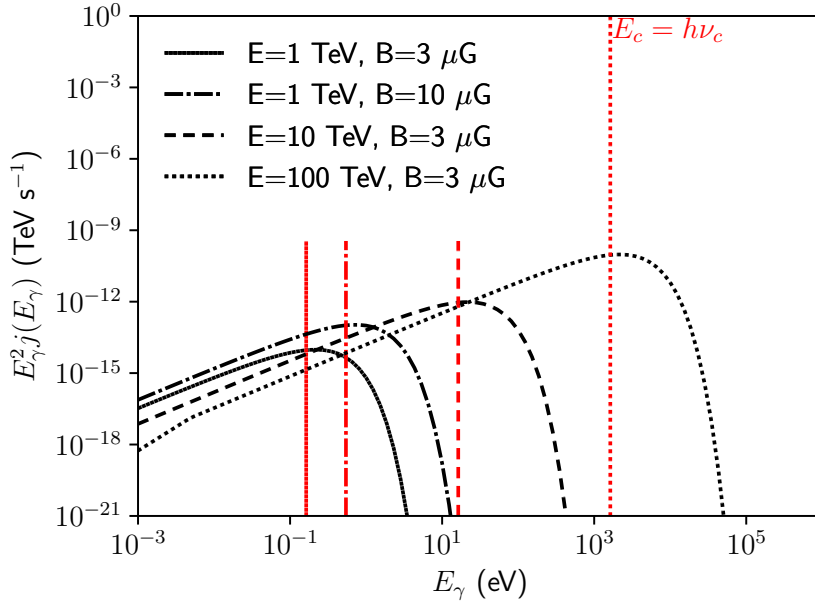
Figure 2.16: Synchrotron emission from an electron with energy E in magnetic field B . The red vertical lines represent the equivalent critical energy ( E_c = h\nu_c ).
