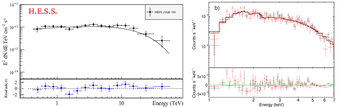
Figure 2.9: TeV ( left ) and X-ray ( right ) SED towards HESS J1826-130 as seen by H.E.S.S. and Suzaku respectively. Images courtesy of H.E.S.S. Collaboration et al., 2020 and Duvdovich et al., 2019 respectively.
