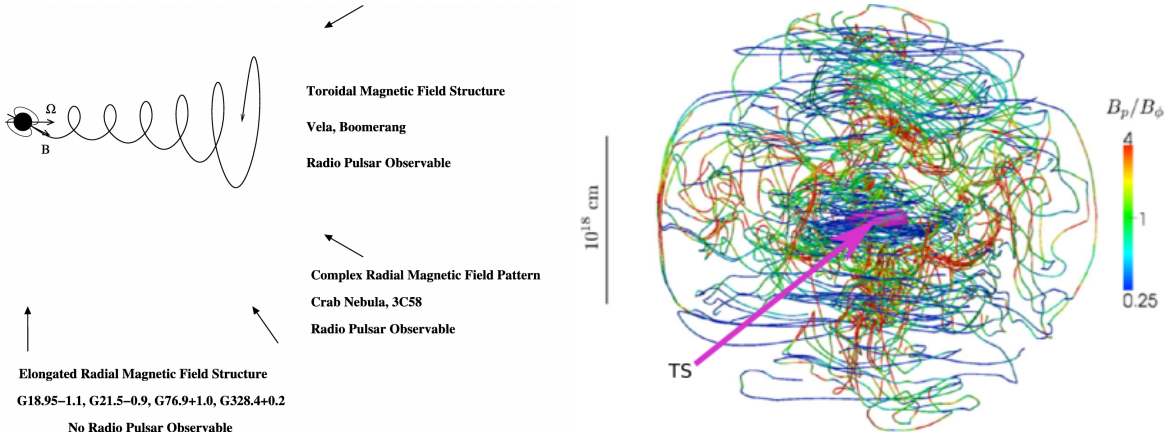
Figure 2.4: ( left ) Expansion of the PWN magnetic field lines and how the viewing angle alters the way the magnetic field structure appears at Earth. Image courtesy of Kothes et al., [2006] ( right ) Simulated magnetic field lines of a stage 1 PWN. Azimuthal orientated field lines are shown in blue while radial field lines are shown in red. The termination shock is indicated by magenta and indicated by the arrow. Image adapted from Porth et al., [2014]
