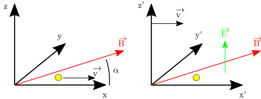
Figure 2.15: An electron travelling at velocity \vec{v} in the x-direction of the lab frame ( left ) with a uniform magnetic field on the x-y plane at angle \alpha to the x-axis. The rest frame of the particle ( right ) travels at velocity \vec{v} to the lab frame. The pure magnetic field \vec{B} (i.e. no electric fields) in the lab frame appears as a mixture of magnetic field \vec{B}' and electric field \vec{E}' in rest frame.
