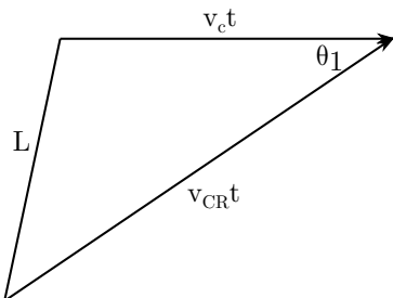
Figure B.2: A ISM cloud travelling at speed v_c in a ‘sea’ of cosmic rays. In time t , the cosmic rays in path L with speed v_{\text{CR}} will enter the cloud.
