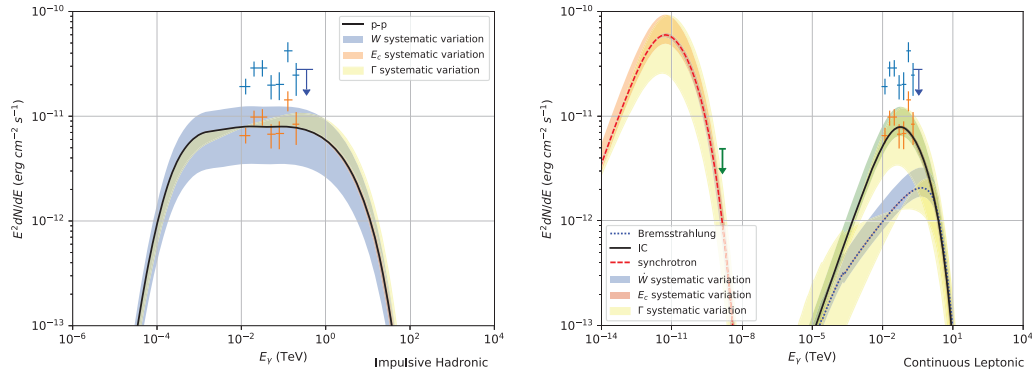
Figure 8. SED example for GeV-B with impulsive hadronic SED (left-hand panel) and continuous leptonic SED (right-hand panel). This assumes that HESS J1825-137 (at age 40 kyr) is the source of acceleration. The upper data points represent the total SED as measured by Fermi -LAT. The lower data points is 34.0 per cent of this spectra due to source being only GeV-B. The green arrow is the ROSAT X-ray upper limit towards GeV-ABC. The blue, pink, and yellow shaded regions represent the systematic variation of energy budget ( W ) or injection luminosity ( \dot{W} ), cutoff energy and spectral index, respectively. See Tables 2 and 3 for input parameters.
