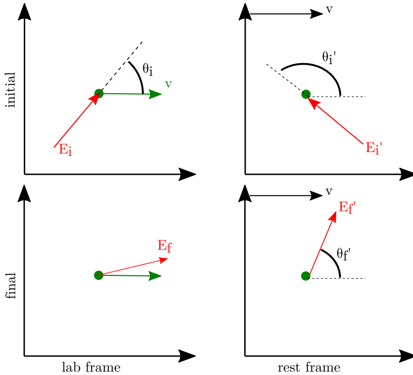
Figure 2.17: A photon with energy E_i scatters off an electron (travelling at velocity v ) at angle \theta in the lab frame ( left ). In the rest frame of the electron ( right ), the photon collides with electron at angle \theta' and energy E'_i . The top and bottom panels describe the situation before and after the collision respectively. After scattering the photon has energy E_f and E'_f in the lab frame and electron rest frame respectively
