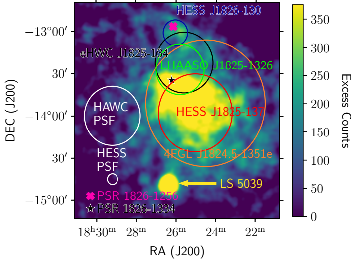
Figure 2.8: HESS excess counts map towards HESS J1825-137 from H.E.S.S. Collaboration et al., [2019]. The spatial position and extent of HESS J1825-137 and the equivalent Fermi -LAT, HAWC and LHAASO sources are shown together with PSR J1826-1334 (star) and PSR J1826-1256 (cross).
