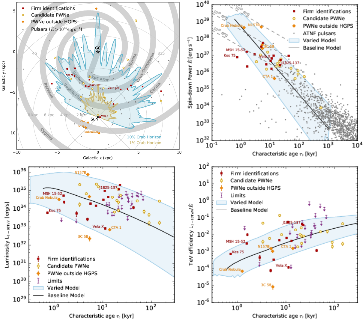
Figure 2.6: ( top-left ) An illustration of the Milky Way spiral arm structure and the location of identified and candidate PWN from the H.E.S.S. HGPS. Spin down power ( top-right ), TeV luminosity ( bottom-left ) and TeV efficiency ( bottom-right ) vs the characteristic age of known PWN. Images from H.E.S.S. Collaboration et al., 2018b.
