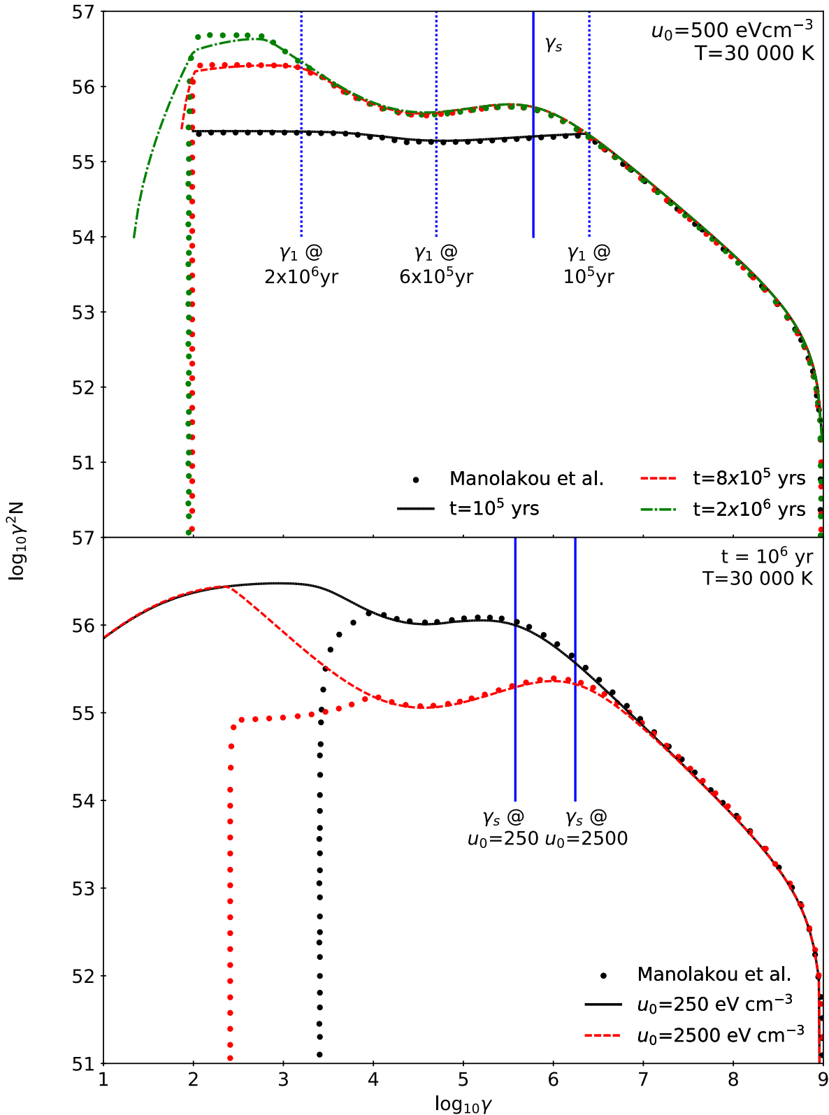
Figure 5.7: Comparison of Newsedprod (solid lines) and results by Manolakou et al., [2007] (dots) where electrons between Lorentz factors \gamma_{\min} = 10^2 and \gamma_{\max} = 10^9 are injected with power law spectrum ( \Gamma = 2.0 ) into a medium with number density and magnetic field n = 1 \text{ cm}^{-3} and B = 10 \mu\text{G} respectively. Electrons are not allowed to escape the cloud ( v_{\text{esc}} = 0 ). (top) Time evolution of electrons against a soft photon field of temperature T = 30000 \text{ K} and energy density u_0 = 500 \text{ eV cm}^{-3} . The positions of \gamma_1 (see [Eq. 5.48]) are shown by the solid vertical blue lines. (bottom) The age of the system is kept constant at 10^6 \text{ yr} while the energy density of the photon field is allowed to vary. Note that the variation at lower Lorentz factors is due to different values of \gamma_{\min} chosen by Manolakou et al., [2007].
