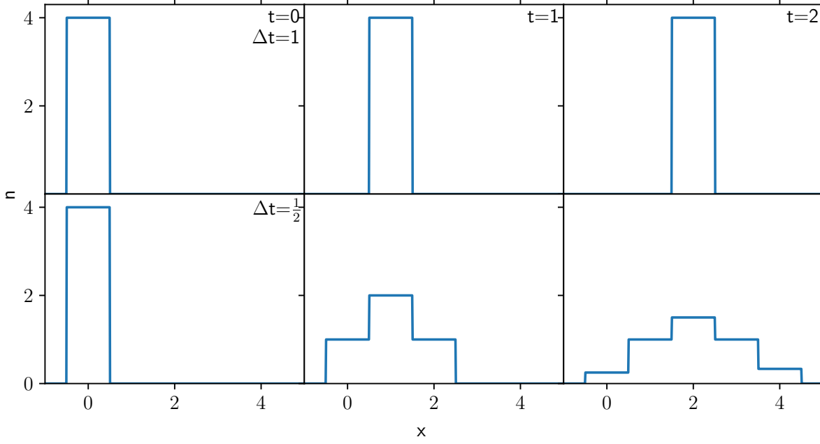
Figure 7.9: The application of finite difference methods for an initial distribution following distribution ( n(-0.5 \leq x < 0.5) = 4 ) at t = 0 with velocity v = 1 . The voxel width ( \Delta x = 1 ) remains constant while the time steps are 1 ( top ) and 0.5 ( bottom ).
