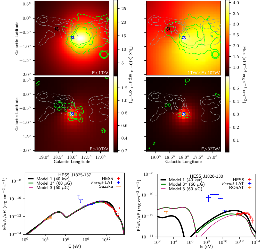
Figure 10. Comparison of the 40 kyr isotropic diffusion - Model 1 (40 kyr, black ), Model 3* (Model 1 + 60 \mu G, green ) and Model 3 (60 \mu G, purple ). The morphology plots towards HESS J1825-137 for Model 3 (60 \mu G) are shown in the top and top-middle panels. See Table 2 for model parameters.
