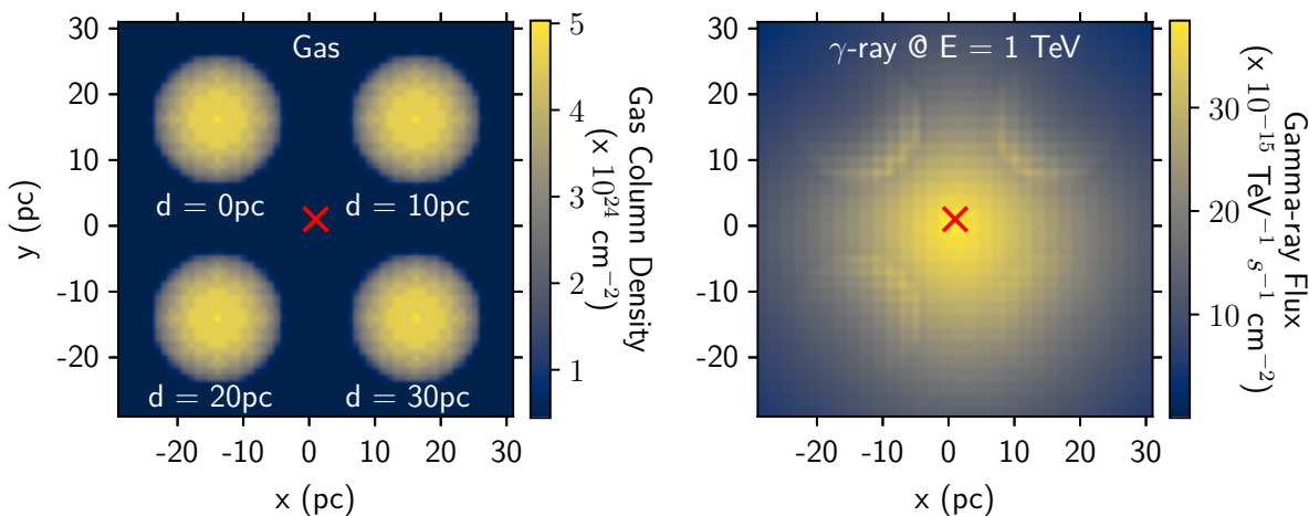
Figure 4.6: (Left) Four spherical gas clouds located 4 kpc from the Earth at distances d along the line of sight ( z -axis runs in/out of page) from a source of electrons (red cross). (Right) Total gamma-ray flux (inverse Compton and Bremsstrahlung) 40 kyr after electron injection commences.
