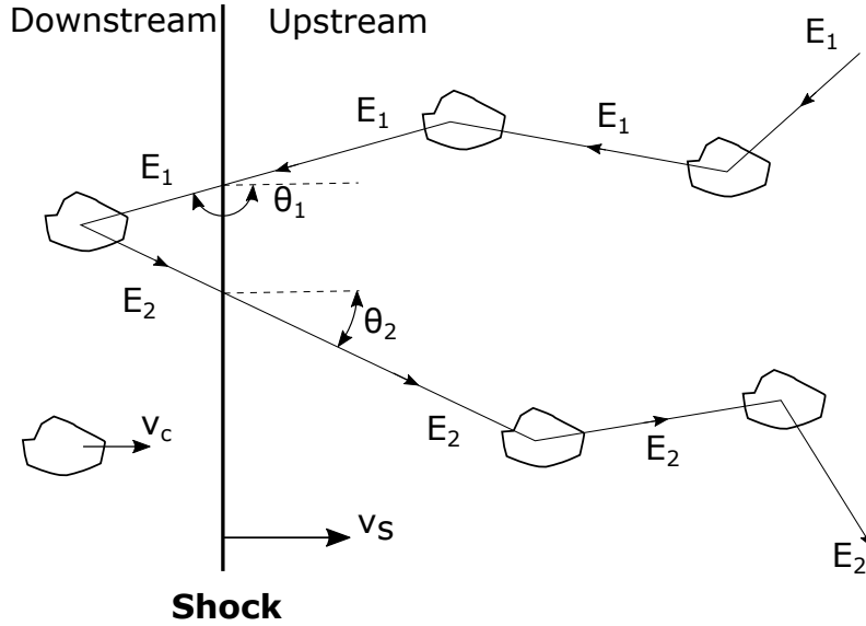
Figure B.4: Aa cosmic ray of energy E_1 travels upstream to downstream of the shock with no change of energy. The cosmic ray scatters off magnetic field turbulence in a cloud downstream of the shock and passes back upstream of the shock with energy E_2 . This process can repeat or the cosmic ray can escape the system.
