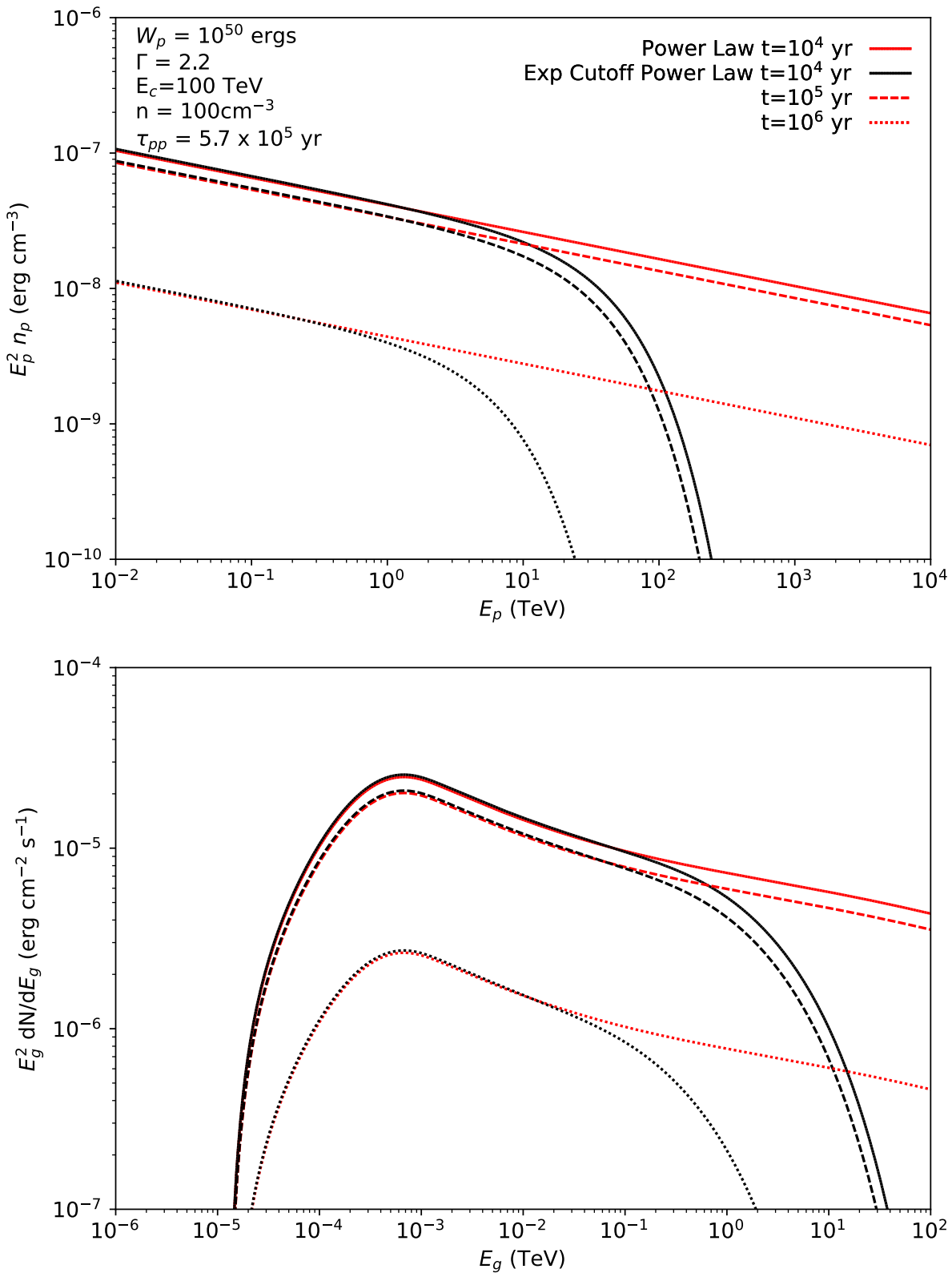
Figure 5.1: Evolution of the cosmic-ray energy density distribution ( top ) and subsequent gamma-ray SED ( bottom ) for an impulsive source injecting protons following a power law spectrum ( \propto E^{-\Gamma} , red) and an exponential cutoff power law spectrum ( \propto E^{-\Gamma} \exp(-E/E_c) , black) as given by Eq. 5.20 . W_p is the total energy of cosmic-ray protons injected at t = 0.1q
