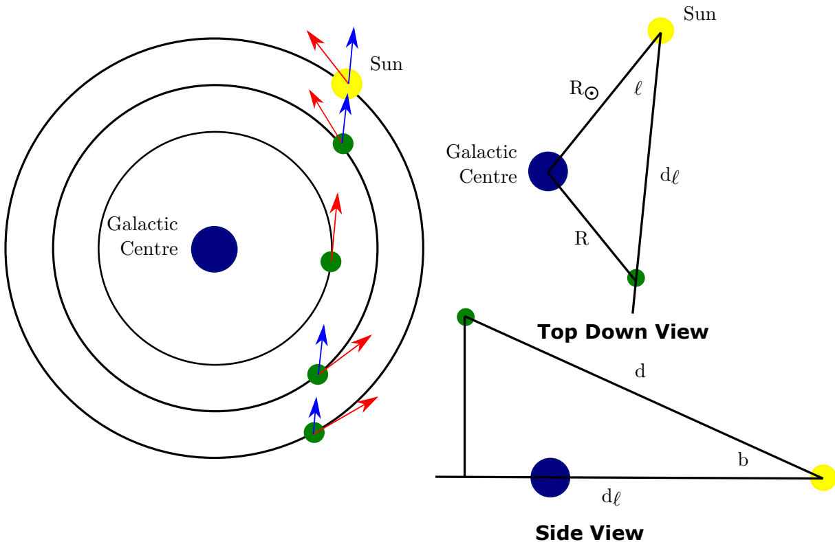
Figure 4.5: (Left) Rotation of the Galaxy around the GC (dark blue circle) with the yellow circle as the Sun, the red arrows are the tangential velocity of the green objects (e.g. gas cloud) and the blue arrows are their velocities projected along the line of sight to the Sun. (Right) Geometry of an object at Galactic longitude \ell , Galactic latitude b and distance d from the Sun.
