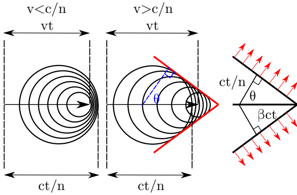
Figure 3.4: Huygens's construction of a charged particle travelling at speed v in a medium of refractive index n . Cherenkov light is emitted at angle \theta when the particle is travelling faster than the speed of light in the medium
