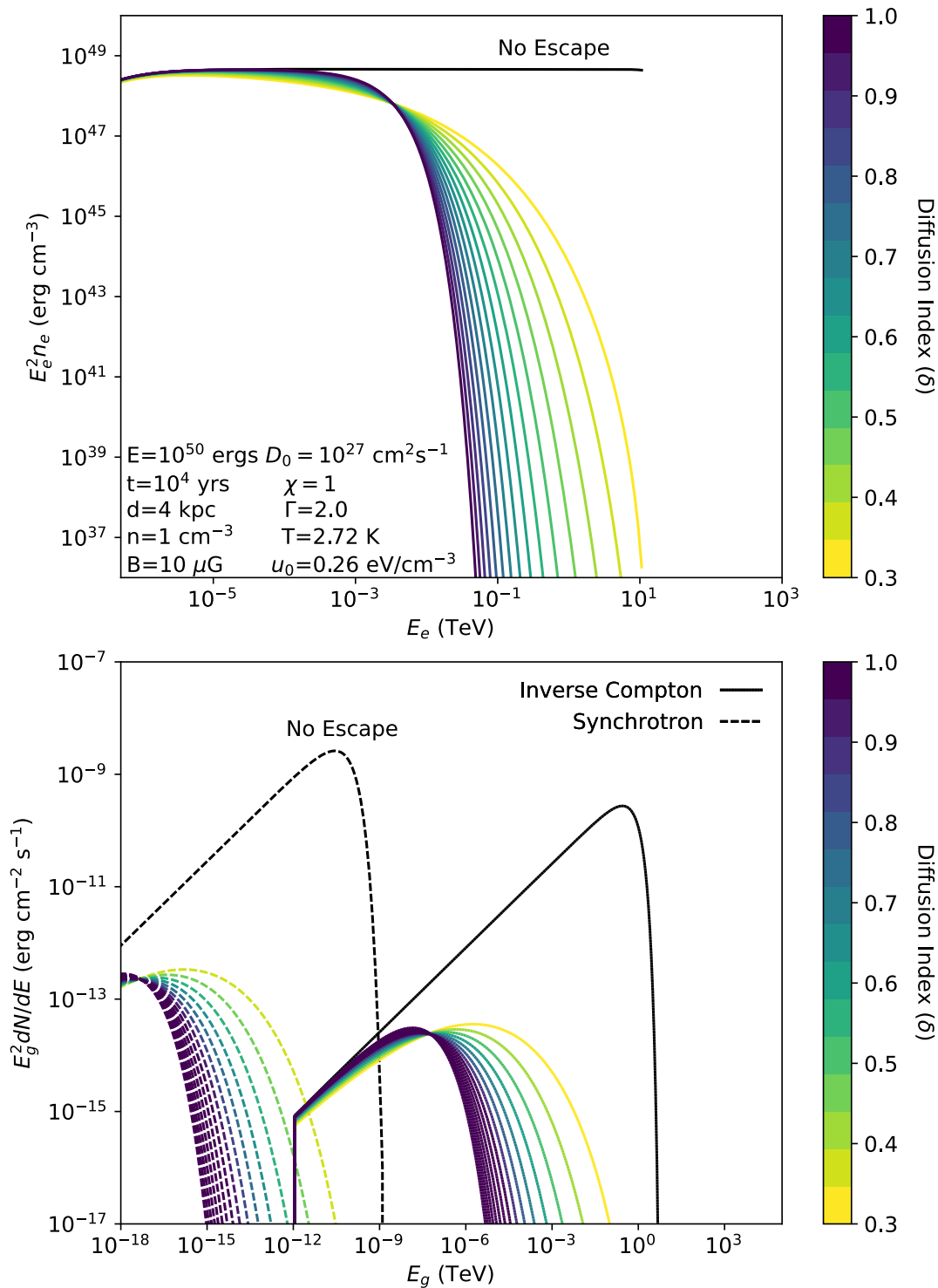
Figure 5.11: Variation of the electron energy density distribution ( top ) and subsequent synchrotron and inverse Compton SED ( bottom ) for an impulsive source of electrons escaping a cloud with radius 10 pc in the different diffusion regimes ( \delta ). Kolmogorov regime: \delta = \frac{1}{3} , Kraichnan regime: \delta = 0.5 and Bohm regime: \delta = 1 . Electrons are injected following a power law spectrum with \Gamma = 2 . The black line represents a situation where there is no escape of electrons.
