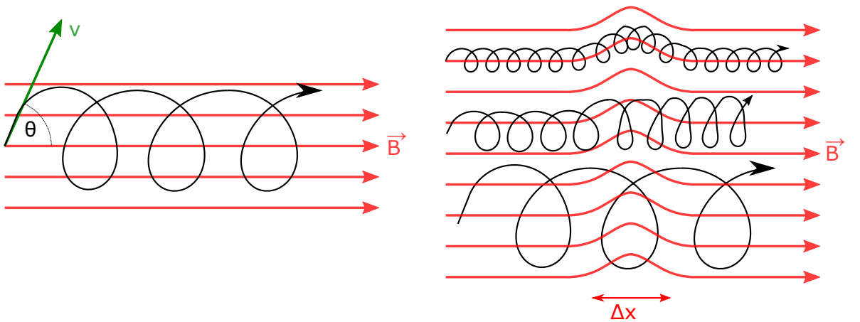
Figure 2.12: (left) The path (black) of motion taken by a charged particle with initial velocity v at angle \theta to a uniform magnetic field B (red). (right) Propagation of a charged particle in a magnetic field with turbulence of length \Delta x when r_g < \Delta x (top), r_g \approx \Delta x (middle) and r_g > \Delta x . (bottom)
