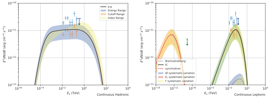
Figure D1. SED example for GeV-A with continuous hadronic SED (left-hand panel) and continuous leptonic SED (right-hand panel). This assumes that LS 5039 (at age 10^5 yr) is the source of acceleration. The upper data points represent the total SED as measured by Fermi -Lat. The lower data points is 36.9 per cent of this spectra due to source being only GeV-A. The green cross is the ROSAT X-ray upper limit towards GeV-ABC. The blue, pink, and yellow shaded regions represent the systematic variation of energy budget ( W ) or injection luminosity ( \dot{W} ), cutoff energy and spectral index, respectively. See Tables 4 and 5 for input parameters.
