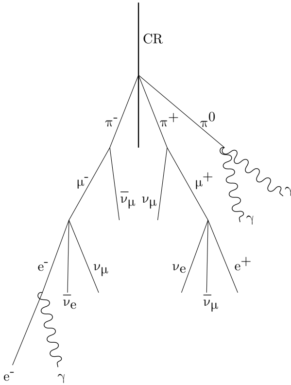
Figure 3.2: The formation of an air shower triggered by a cosmic ray entering the atmosphere. The cosmic ray undergoes proton-proton interactions to produce neutral and charged pions. Neutral pions decay into two photons (which can trigger an electromagnetic air shower) while charged pions decay into muons and neutrinos. The muons decay into electrons/positrons and neutrinos. Depending on its energy, the original cosmic ray can undergo further proton-proton collision.
