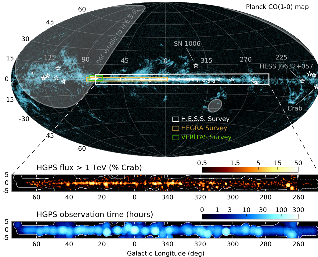
Figure 3.8: The H.E.S.S. Galactic plane survey superimposed onto Planck CO data. Image courtesy of H.E.S.S. Collaboration et al., 2018a .
