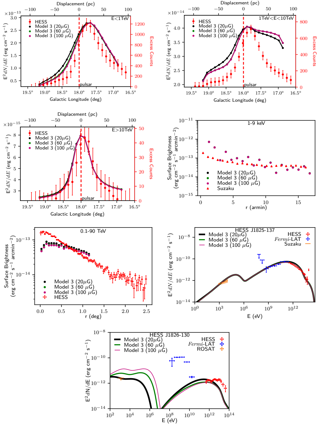
Figure 9. The energy flux along Galactic longitude profiles ( top & top-middle left ), surface brightness radial profiles ( top-middle right & bottom-middle left ) and SED towards HESS J1825-137 ( bottom-middle right ) and HESS J1826-130 ( bottom ) for Model 3 (20 μG, black), (60 μG, green) and (100 μG, purple) around HESS J1826-130. See Table 2 for model parameters.
