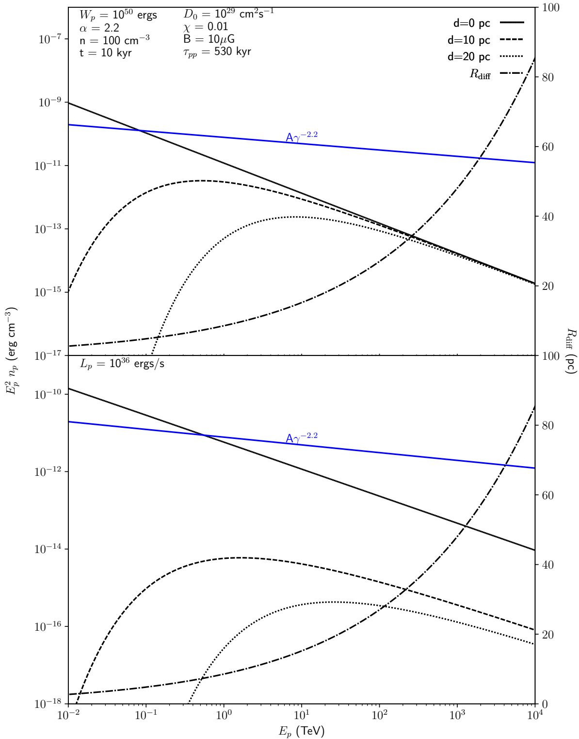
Figure 5.5: The cosmic-ray energy density distribution for an impulsive (top panel) and continuous (bottom panel) source of protons after 10 kyr as described by Eq. 5.38 and Eq. 5.39 respectively. The solid blue line shows the shape of the injected proton energy distribution ( \propto E^{-\Gamma} ). For reference, the diffusion distance ( Eq. 5.37 ) is represented by the dashed-dotted line.
