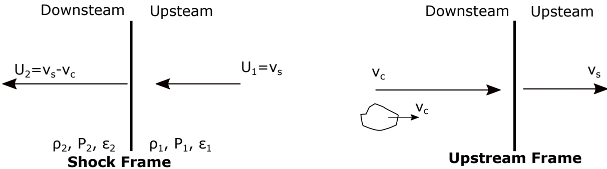
Figure B.3: A shock travelling through the ISM with velocity v_s in the upstream reference frame. ( left ) In the reference frame of the shock, the material upstream travels towards the shock at velocity U_1 = v_s . The material downstream of the shock travels at velocity U_2 = v_s - v_c , where v_c is the velocity of an ISM gas cloud in the upstream reference frame ( right ). The material upstream and downstream of the shock have densities, pressure and internal energy \rho , P and \epsilon respectively.
