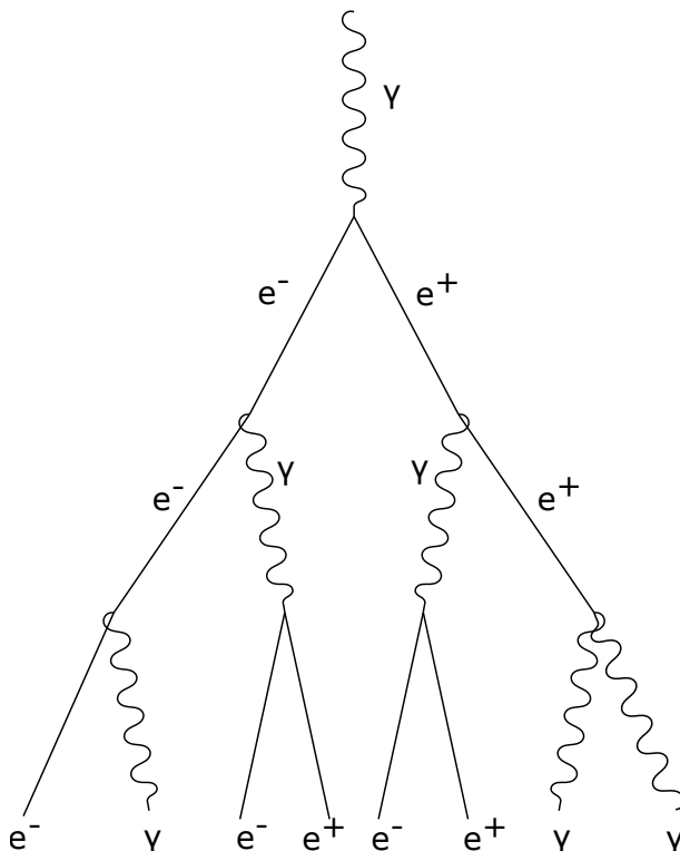
Figure 3.1: Heitler's model of the formation of an air shower triggered by a gamma ray (Heitler, 1954 ). The gamma ray undergoes pair production to produce an electron and positron. In turn, the electron/positron undergo Bremsstrahlung interactions and/or electron-positron annihilation to produce photons. This process cascades into the air shower.
