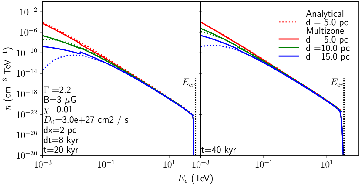
Figure 7.7: Energy distribution of electrons 20 kyr ( left ) and 40 kyr ( right ) after an impulsive accelerator injects electrons into a system with the same parameters as Fig. 7.5 . The electron energy distribution of electrons is taken 5 pc (red), 10 pc (green) and 15 pc (blue) from the accelerator with the analytical and numerical solutions being represented by the circles and solid lines respectively. The vertical black dotted lines represents the critical energy E_{cr} of electrons (see Eq. 5.24 ).
