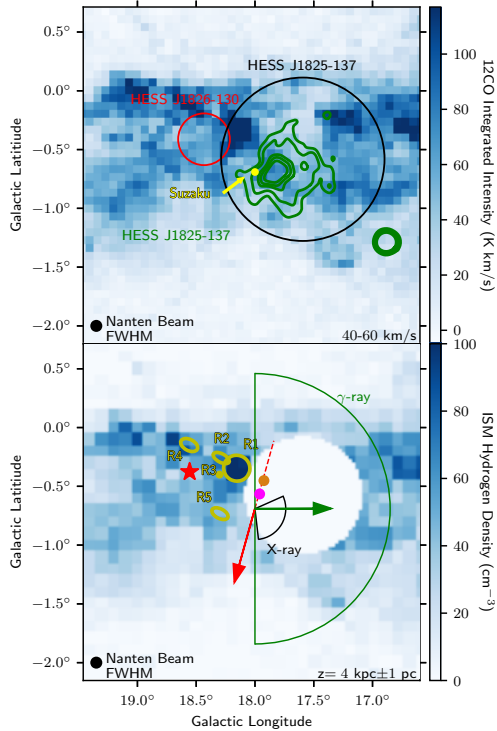
Figure 3. ( top ) Nanten ^{12}\text{CO}(1-0) integrated intensity in the velocity range 40\text{--}60\text{ km s}^{-1} corresponding to 3.5\text{--}4.5\text{ kpc} overlaid by green H.E.S.S. contours (at 4, 5, 6, 7, 8 and 9\sigma ). The yellow dot represents the Suzaku region A as defined in Uchiyama et al. (2009) and is used to extract the X-ray SED. The region used to obtain the gamma-ray spectra towards HESS J1825-137 and HESS J1826-130 are shown in black and red respectively. ( bottom ) Calculated ISM number density across the 3D grid at 4\text{ kpc} \pm 1\text{ pc} where the voxels within the PWN extent ( R < 0.5^\circ ) are set to a density of 0.5\text{ cm}^{-3} to represent the bubble that has been swept out by the stellar wind from the progenitor star. The proper motion of the pulsar is shown by the red arrow with the projected birthplaces indicated by the red-dashed line. The projected birthplaces for ages 21 kyr and 40 kyr are indicated by the magenta and brown dot respectively. The direction of advective particle transport suggested by H.E.S.S. Collaboration et al. (2019) is shown by the green arrow. The black and green segments represent the regions used to extract the X-ray and gamma-ray surface brightness radial profile respectively. Molecular clouds R1-R5 from Voisin et al. (2016) are shown in yellow with the position of PSR J1826-1256 indicated by the red star. The width and height of the voxel in the 2D slice is 2\text{ pc} compared to the minimum Nanten resolution of 5\text{ pc} (assuming a distance of 4\text{ kpc} ).
