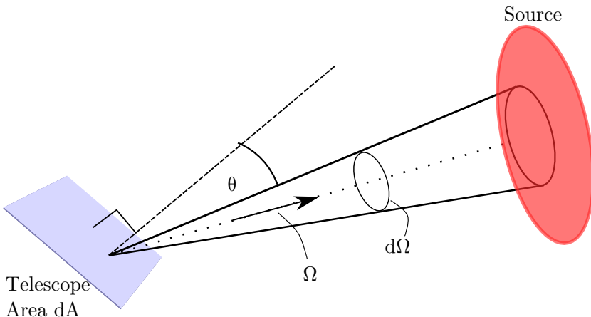
Figure 4.2: A basic illustration of a telescope with area dA observing a cloud of ISM gas with solid angle d\Omega at orientation \theta .
