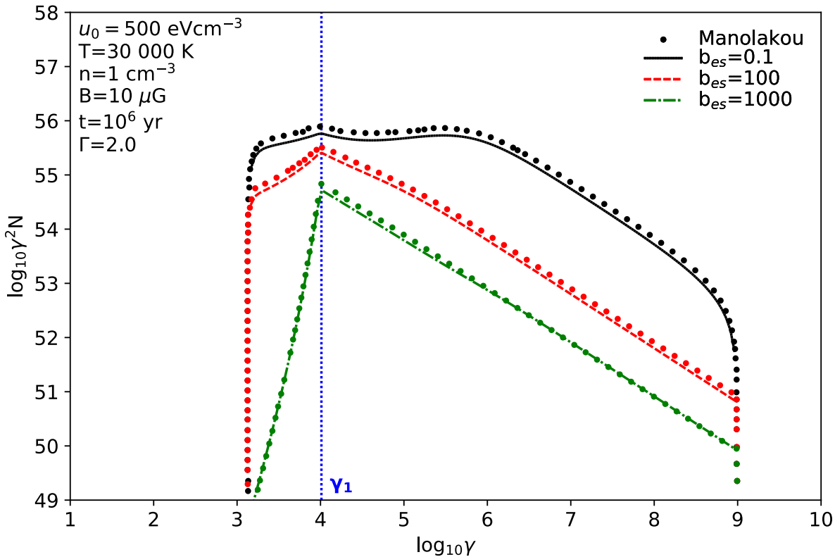
Figure 5.10: Comparison of Newsedprod (solid lines) to results by Manolakou et al., 2007 where electrons are allowed to escape the system at rate \nu_{\text{esc}} = b_{\text{es}} \gamma (see Eq. 5.55 ), i.e. Bohm diffusion regime. Electrons are injected with a power-law spectrum \Gamma = 2.0 . The position of \gamma_1 is represented by the vertical dotted line.
