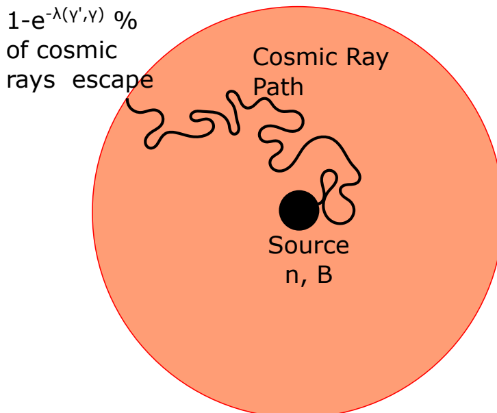
Figure 5.9: An accelerator inside a uniform region of ISM with number density n and magnetic field B . After injection, cosmic rays scatter off magnetic field turbulence resulting in net diffusion from the accelerator. The probability that a cosmic ray escapes the region while cooling from Lorentz factor \gamma' \rightarrow \gamma is 1 - \exp(-\lambda(\gamma', \gamma)) (see Eq. 5.10)
