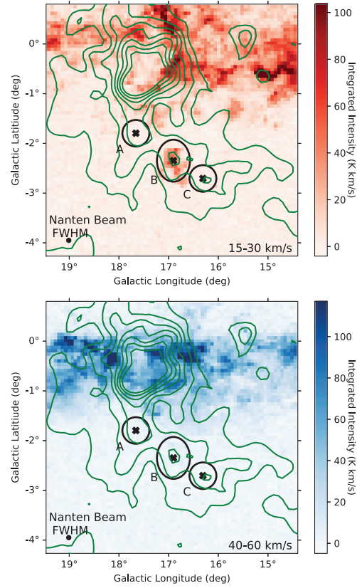
Figure 2. Nanten 12CO(1-0) integrated intensity in velocity ranges 15–30 \text{km s}^{-1} (top) and 40–60 \text{km s}^{-1} (bottom). The green contours represents GeV emission as seen by Fermi -LAT at 1\sigma to 7\sigma . The new regions of GeV emission, GeV-A, GeV-B, and GeV-C, are shown by black markers. The Nanten beam size, shown in bottom left, is 2.6 arcmin (Mizuno & Fukui 2004).
