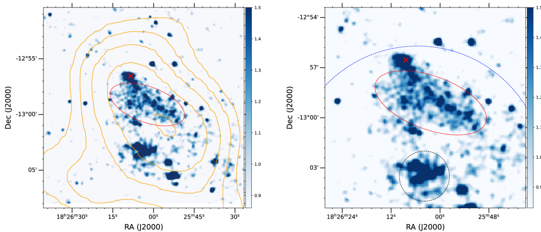
Figure 2.10: XMN-Newton 0.5 – 10 keV X-ray images towards HESS J1826-130. The positions of PSR 1826-1256 and the Eel Nebula are shown by the red cross and ellipse respectively. The orange lines represent the H.E.S.S. 3\sigma and 5\sigma significance contours. Nearby SNR G18.45-0.42 and star cluster Bica 3 are shown by the dashed blue and black circles respectively. Image courtesy of Burgess et al., [2022].
