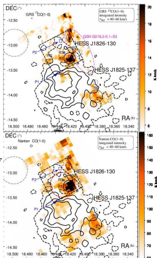
Figure 4.1: 13 CO(1 – 0) ( top ) and 12 CO(1 – 0) ( bottom ) integrated intensity between velocity range 40–60 km s -1 (equivalent to 3.5 – 4.5 kpc) towards HESS J1825-137. HESS TeV gamma-ray emission contours are shown by the solid and dashed black contours. Image courtesy of (Voisin et al., 2016)
