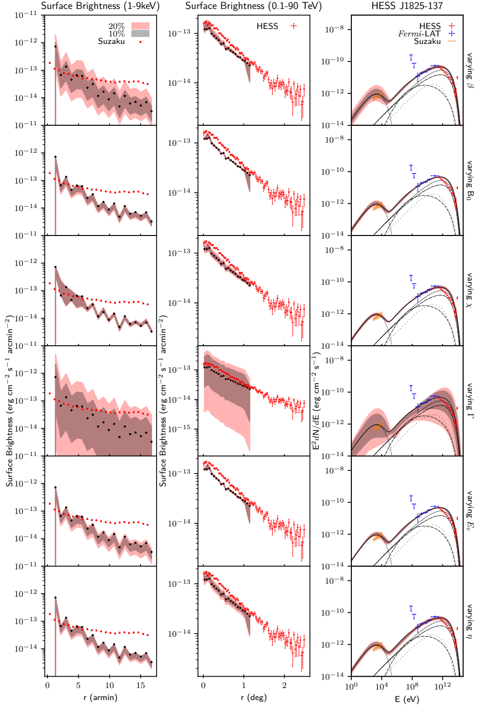
Figure D1. Model 1 (21 kyr) as in Figure 4 but with 10% (grey shaded band) and 20% (pink shaded band) variation in parameters. MNRAS 000 , 1–20 (2022)
