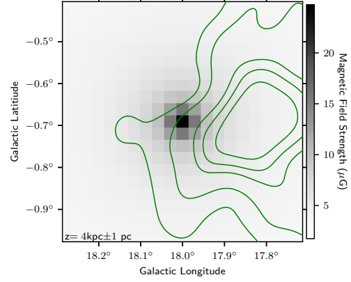
Figure 2. The radially symmetric magnetic field due to the pulsar at slice z = 4 \text{ kpc} \pm 1 \text{ pc} . Overlaid are the green H.E.S.S. contours at 4, 5, 6, 7, 8 and 9\sigma (H.E.S.S. Collaboration et al. 2019).
