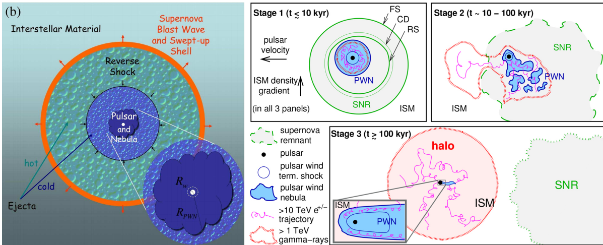
Figure 2.3: (left) Structure of a composite SNR and PWN. Image courtesy of Gaensler and Slane, [2006] (right) A PWN evolves within the SNR and is eventually crushed by the reverse shock. The pulsar escapes the SNR and the electrons escaping into the ISM form a TeV halo around the PWN. Image courtesy of Giacinti et al., [2020]
