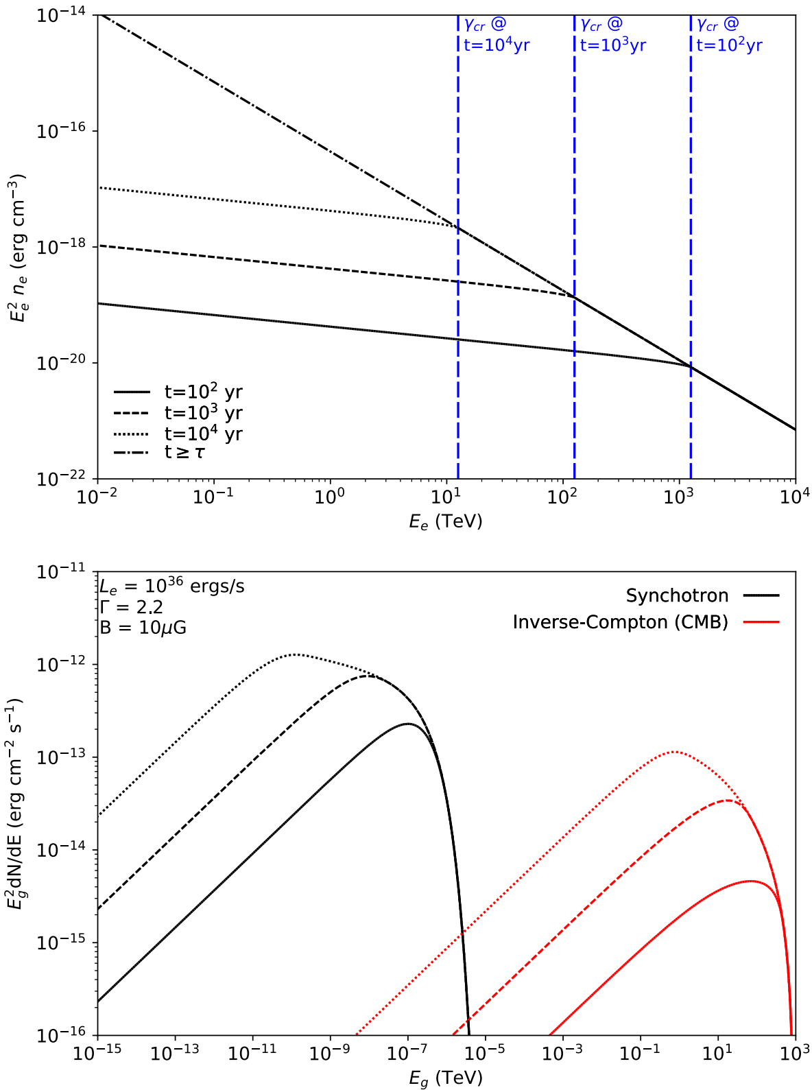
Figure 5.4: Evolution of the cosmic-ray energy density distribution ( top ) and subsequent gamma-ray SED ( bottom ) for a continuous source injecting electrons following a power law spectrum as given by Eq. 5.34 . The steady state of electrons ( t \gg \tau \approx \tau_{\text{sync}} , see Eq. 5.35 ) is represented by the dash-dot line. L_e is the energy of electrons injected per second into the system.
