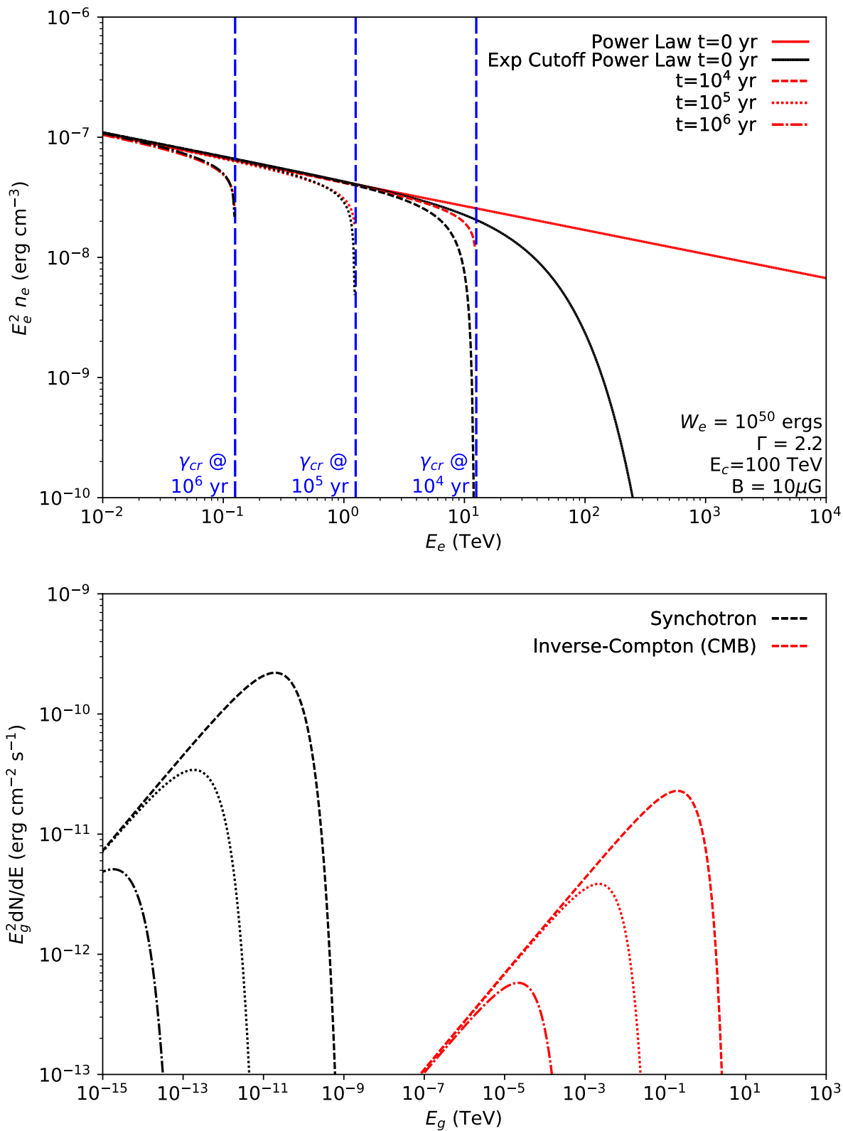
Figure 5.2: Evolution of the cosmic-ray energy density distribution ( top ) and subsequent gamma-ray SED ( bottom ) for an impulsive source injecting electrons following a power law spectrum (red) and an exponential cutoff power law spectrum (black) as given by Eq. 5.26. The critical Lorentz factor (Eq. 5.24) at different ages are shown by the vertical blue-dashed lines.
