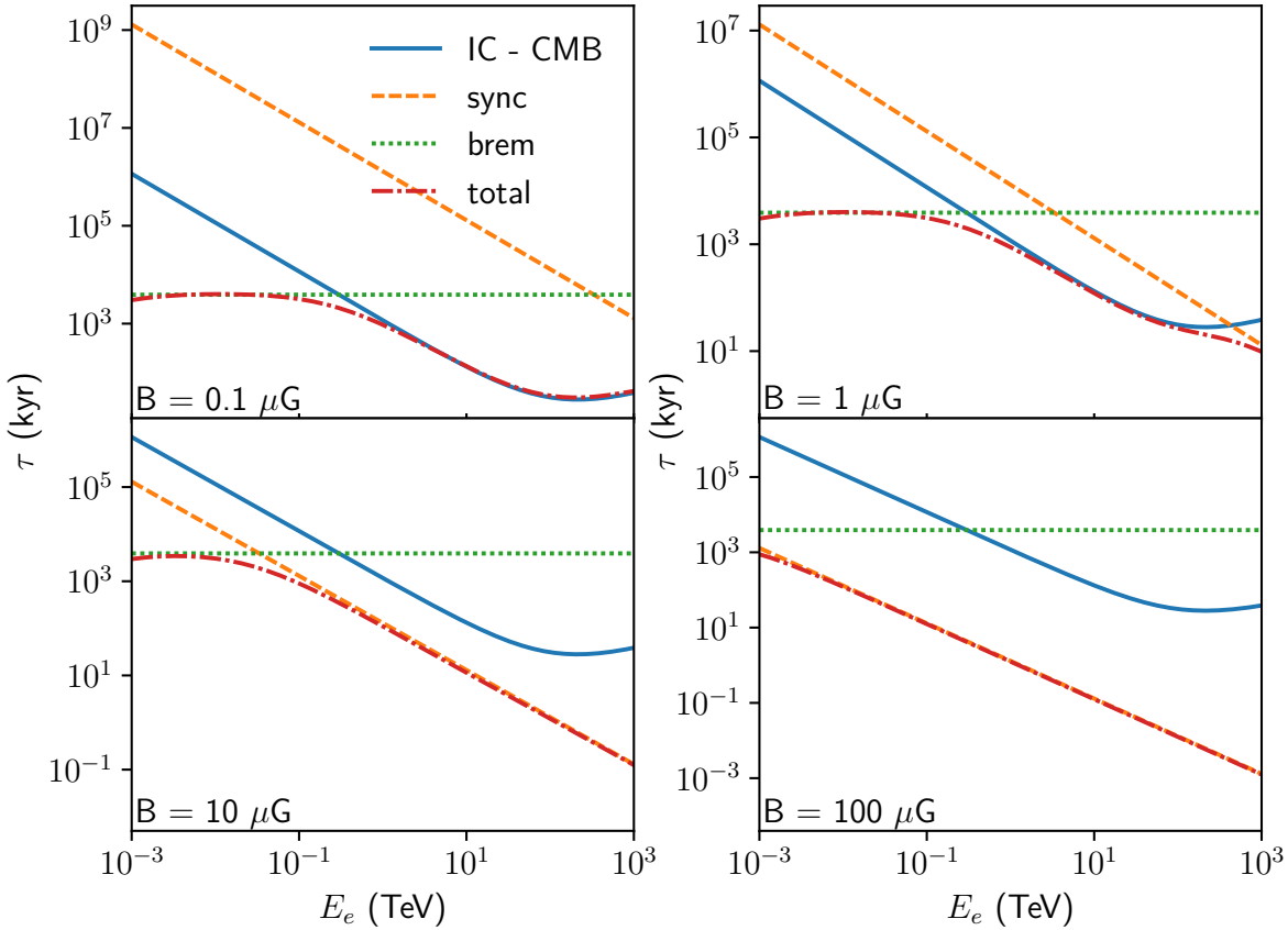
Figure 2.19: Cooling times for electrons at different energies in a uniform cloud with density n = 10 \text{ cm}^{-3} and magnetic field B = 0.1, 1, 10 \text{ \& } 100 \mu\text{G} . The solid blue line shows the cooling time for inverse Compton interactions against the CMB ( U_{\text{CMB}} = 0.26 \text{ eV cm}^{-3} ). The dashed yellow line shows the cooling time for synchrotron interactions while the dotted green line shows the cooling time for Bremsstrahlung interactions.
