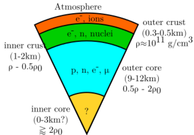
Figure 2.1: The neutron star/pulsar structure is composed of an inner & outer core, inner & outer crust and an atmosphere (Haensel et al., 2007 ).
