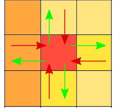
Figure 7.2: The electron energy distribution in each voxel will be calculated by tracking the flux in (red) and out (green) of neighbouring cells.
