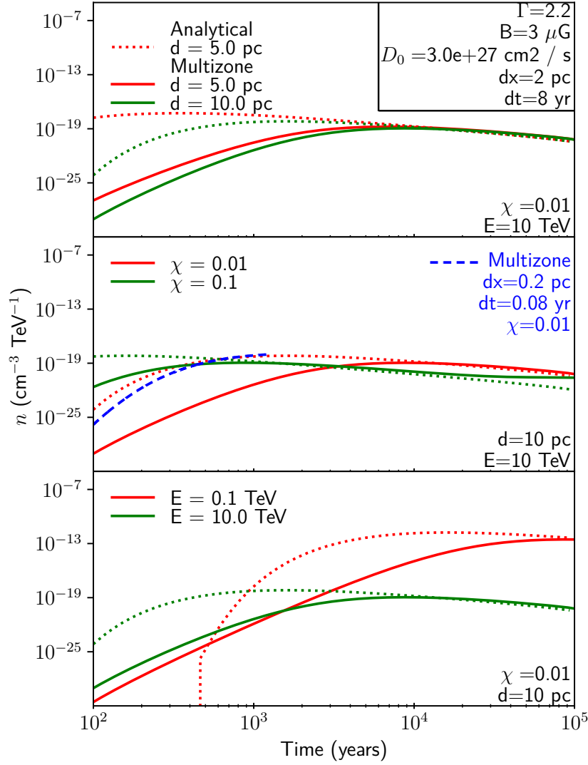
Figure 7.6: Evolution of the impulsive electron energy density distribution for the analytical solution (filled dots) and numerical solution (solid lines) with the same parameters to Fig. 7.5. The top panel shows the evolution at distance 5 pc and 10 pc from the source. The middle panel compares the evolution for a situation where \chi = 0.01 and \chi = 0.1 . The blue dashed line represents the numerical solution for \chi = 0.01 with a time and spatial resolution of dt = 0.08 yr and dx = 0.2 pc respectively. The bottom panel compares the evolution for electrons with energy E = 0.1 TeV and 10 TeV.
