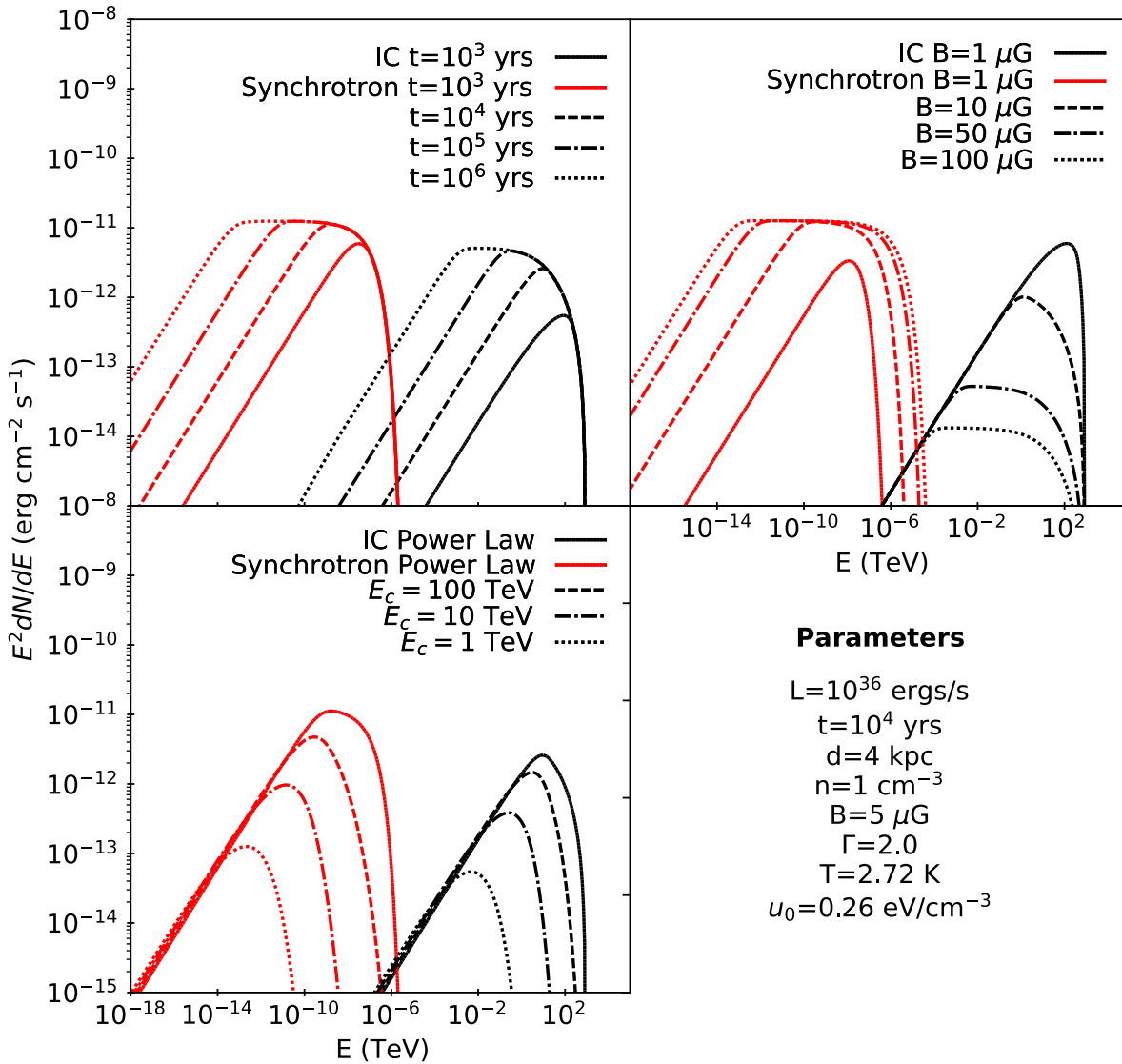
Figure 5.8: The multi-wavelength SED results from Newsedprod for different scenarios of a continuous source. Unless otherwise stated, the input parameters are shown in the bottom-right panel ( L =energy injection luminosity, t =age of system, d =distance to the cloud from Earth, n =density of ISM, B =background magnetic field, \Gamma =spectra of injected electrons, T and u_0 are the temperature and energy density of the background CMB field.)
