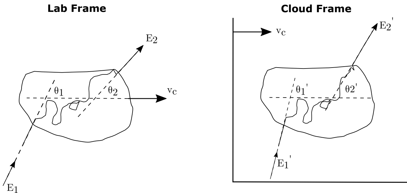
Figure B.1: In the lab frame ( left ), a cosmic ray with energy E_1 enters an ISM cloud (travelling at speed v_c ) at angle \theta_1 and scatters off magnetic field turbulence and exits the cloud with energy E_2 and angle \theta_2 . The same process is shown in the right, but in the reference frame of the cloud (labeled as primed).
