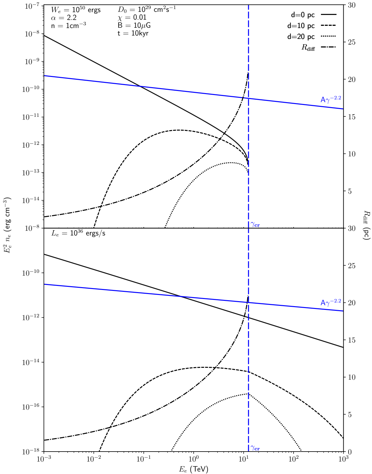
Figure 5.6: The cosmic-ray energy density distribution for an impulsive source ( top ) and continuous source ( bottom ) of electrons following a power law (solid blue line) after t = 10 kyr as described by Eq. 5.42 and Eq. 5.43 respectively. For reference, the diffusion distance is represented by the dashed-dotted line and the critical energy ( \gamma_{\text{cr}} \approx 13 TeV) is shown by the blue vertical dashed line.
