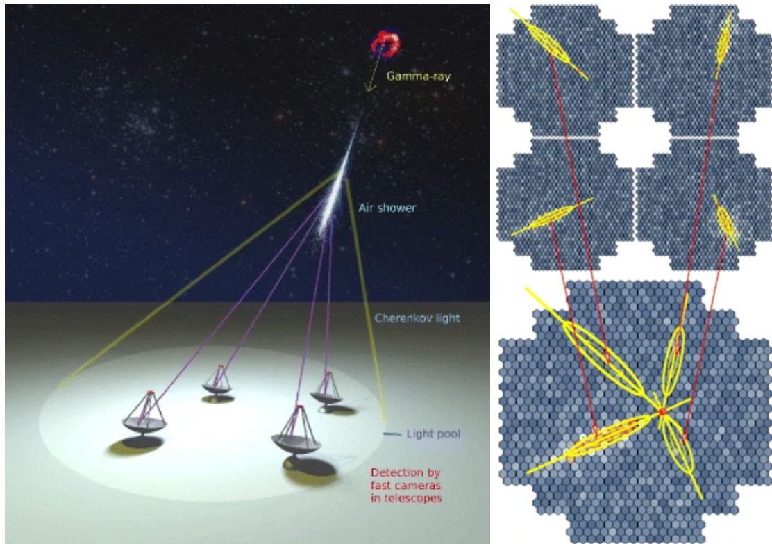
Figure 3.5: ( left ) Pool of Cherenkov light from an air shower observed by four telescopes in a stereo system. ( right ) Projection of the Cherenkov light onto one camera focal plane by the four telescopes. Images courtesy of Völk and Bernlöhr, [2009].
