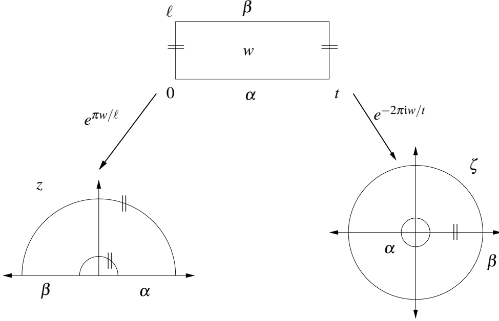
FIGURE 3.2. Changing coordinates from the half plane ( z ) to the annulus ( \zeta ) via the strip ( w ). Periodic boundary conditions are labelled with \parallel , and symmetry-preserving gluing conditions are labelled \alpha and \beta .
