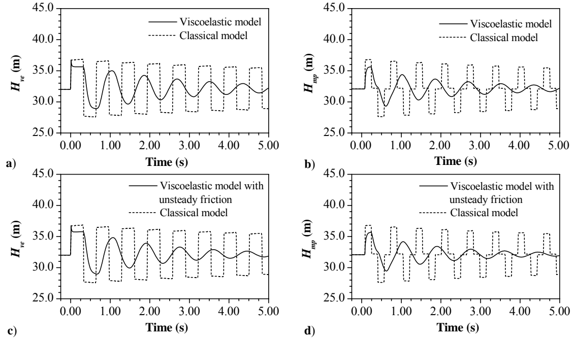
Figure 10 Comparison of heads at the valve ( H_{ve} ) and at the midpoint ( H_{mp} ) in a medium-density polyethylene pipeline; \text{Re}_0 = 4,360 .
