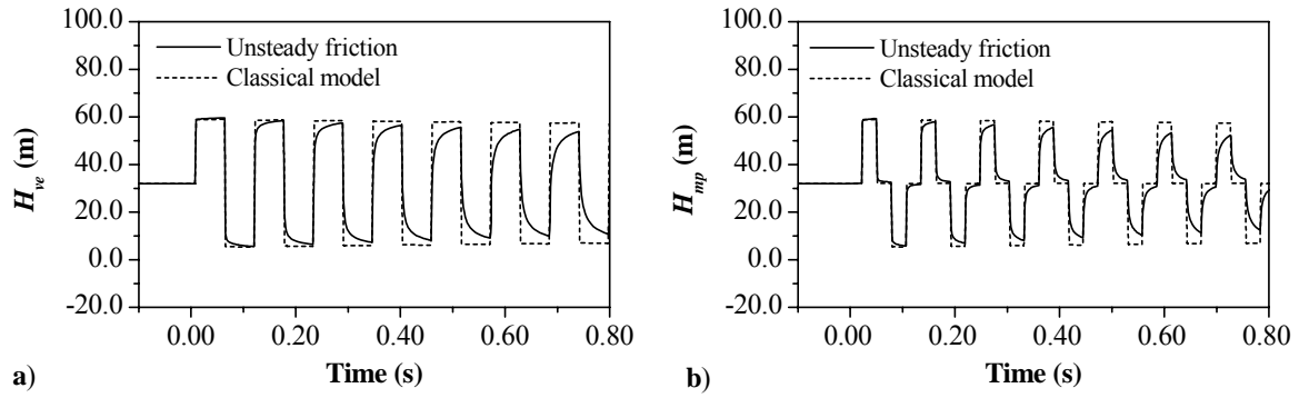
Figure 3 Comparison of heads at the valve ( H_{ve} ) and at the midpoint ( H_{mp} ) in a copper pipeline; \mathbf{Re}_0 = 4,360 .
