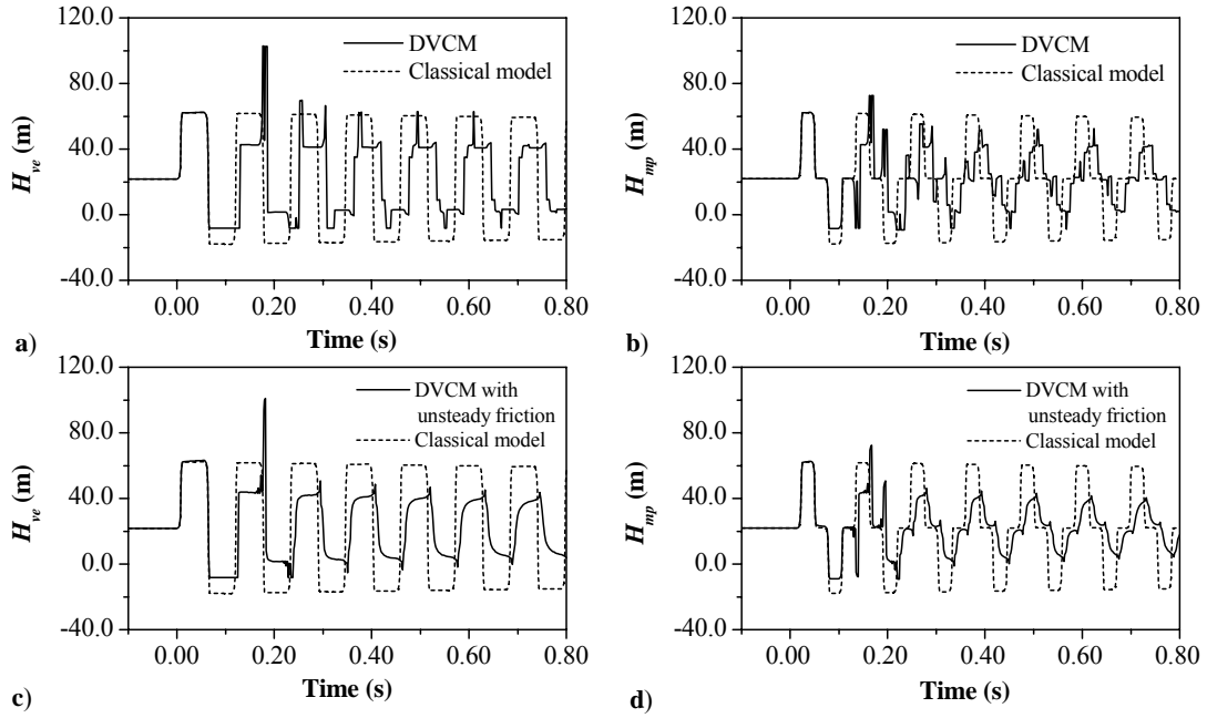
Figure 4 Comparison of heads at the valve ( H_{ve} ) and at the midpoint ( H_{mp} ) in a copper pipeline; \mathbf{Re}_0 = 6,540 .
