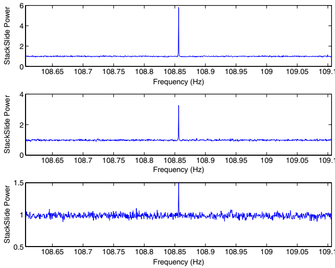
FIG. 25 (color online). The StackSlide Power vs frequency for H1 (top), L1 (middle), and H2 (bottom) using the sky position and the f value of the template that gives the outlier in H1, for outlier number 2 given in Table IX. Comparing with Tables V and VI this outlier is identified as due to hardware injection Pulsar3.
