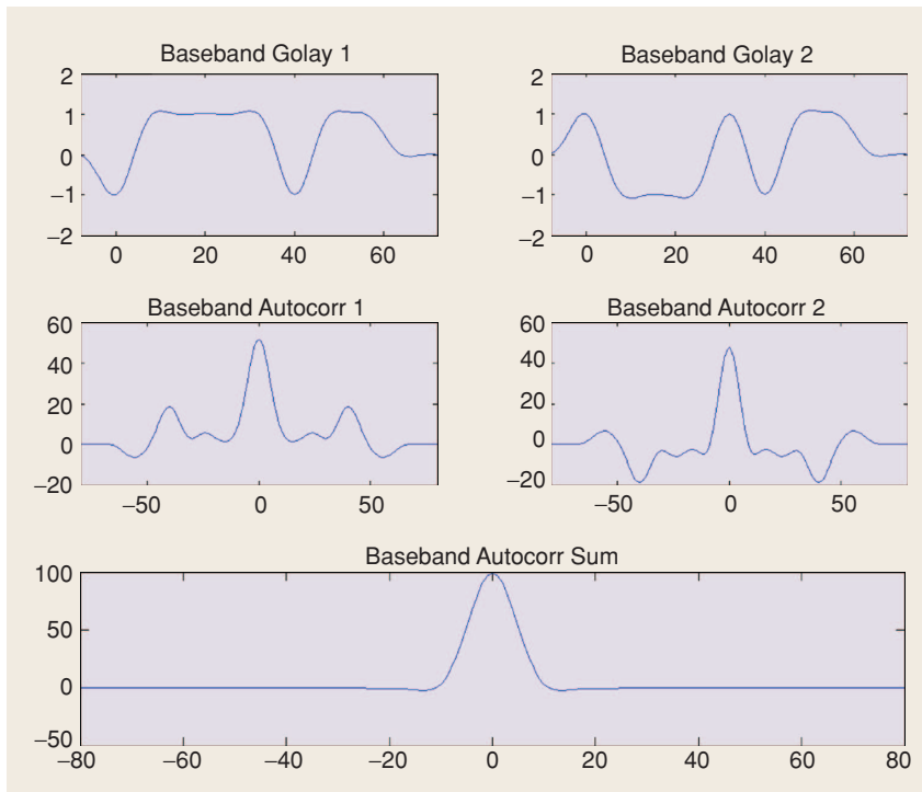
[FIG3] The Golay Property after low-pass filtering.
