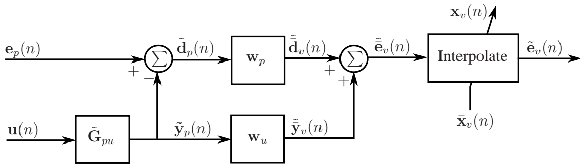
Figure 11. Block diagram of the adaptive LMS moving virtual microphone technique.
