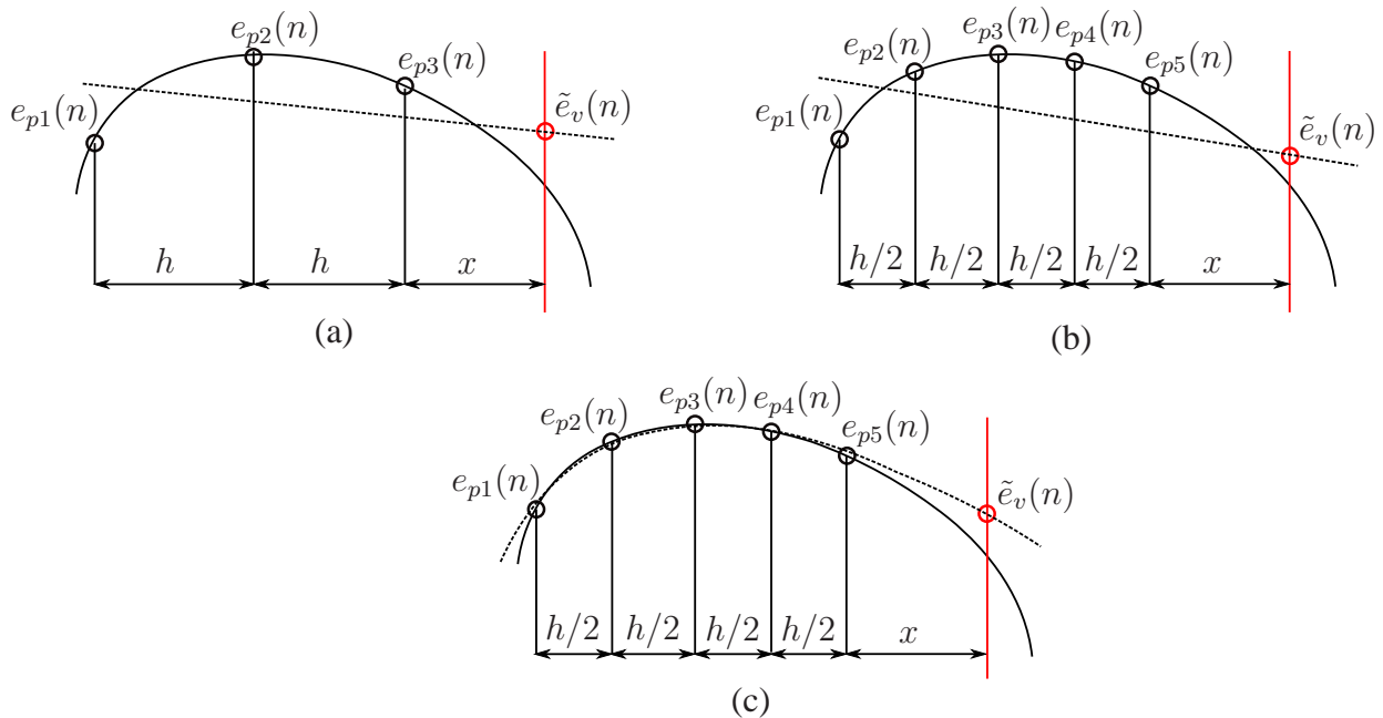
Figure 6. Diagram of (a) three microphone linear forward difference extrapolation; (b) five microphone linear forward difference extrapolation; and (c) five microphone quadratic forward difference extrapolation. The black curved line represents the actual pressure field and the dashed line represents the pressure estimate.
