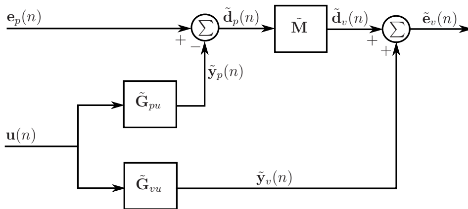
Figure 4. Block diagram of the remote microphone technique.
