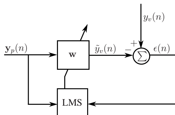
Figure 7. Block diagram of the adaptive LMS algorithm used to calculate the physical sensor weights.
