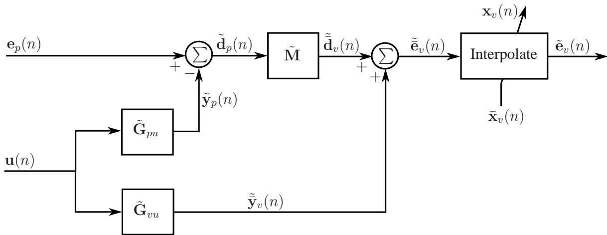
Figure 10. Block diagram of the remote moving microphone technique.
