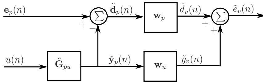
Figure 8. Block diagram of the adaptive LMS virtual microphone technique [38].
