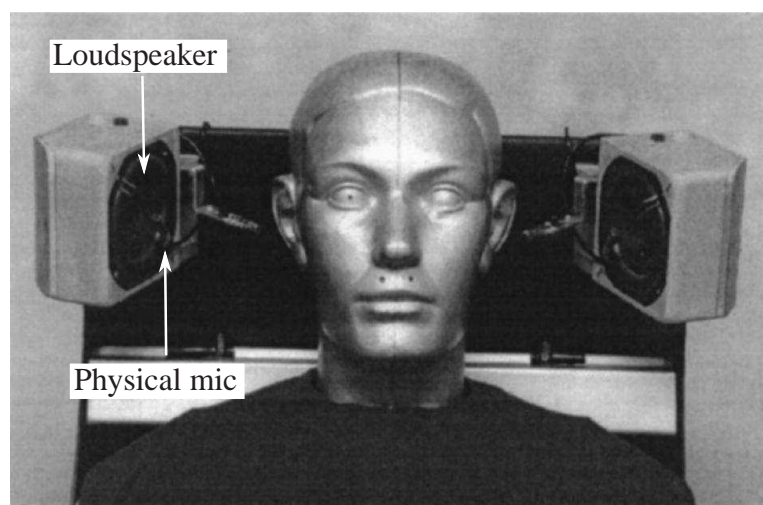
Figure 3. Local active headrest [23].
