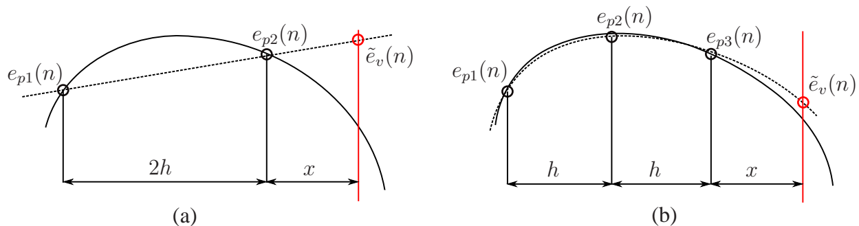
Figure 5. Diagram of (a) two microphone linear forward difference extrapolation; and (b) three microphone quadratic forward difference extrapolation. The black curved line represents the actual pressure field and the dashed line represents the pressure estimate.
