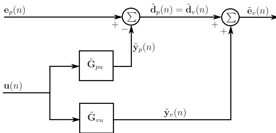
Figure 2. Block diagram of the virtual microphone arrangement.
