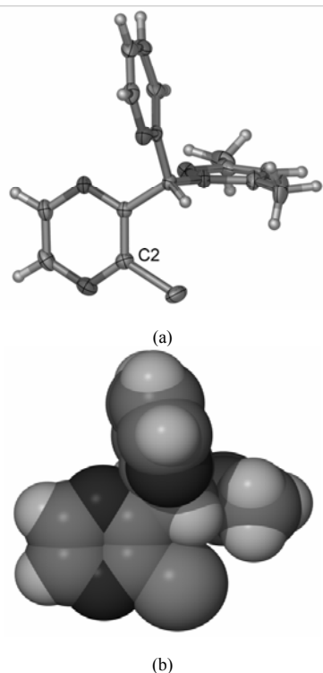
Figure 2. (a) A perspective view of the X-ray molecular structure of compound 9a showing the possible origin of the steric hindrance. Thermal ellipsoids are shown at the 50% probability level. (b) A space-filling representation of the structure.
