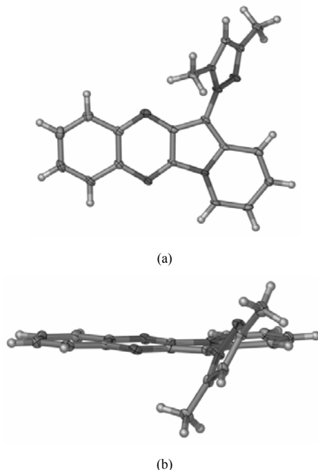
Figure 4. (a) A perspective view of the molecular structure of 5b showing the planar indolizino[2,3- b ]quinoxaline core with thermal ellipsoids at the 50% probability level. (b) A view of 5b perpendicular to the core showing the out-of-plane twist of the pyrazole ring.
