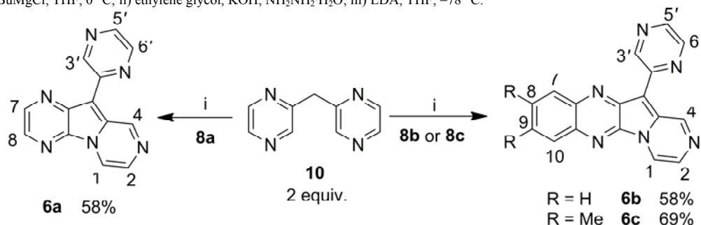
Scheme 3. i) n -BuLi, THF, -78 °C, r.t. to reflux.
