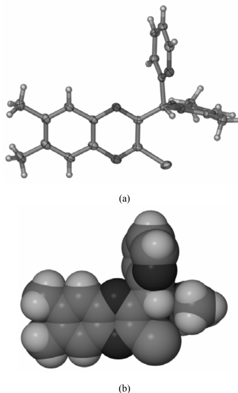
Figure 3. (a) A perspective view of the solid-state molecular structure of 9c . Thermal ellipsoids are shown at the 50% probability level. (b) A space-filling representation alludes to the possibility that the pyrazole ring hinders the approach of nucleophiles to C2 of 9c .
