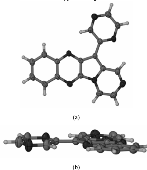
Figure 6. (a) A perspective view of the molecular structure of 6b showing the planar core, with thermal ellipsoids at the 50% probability level. (b) A view of 6b perpendicular to the core showing the near planar conformation of the pyrazine ring.
