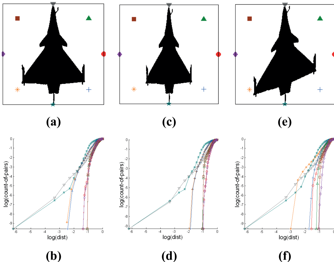
Figure 3. Effect of binary pattern with shape distortion and Cross-plots based signatures. The graphs demonstrate that the variation of Cross-plots can be attributed to the slight distortion in target patterns. The differences presented by the shape contrast indices of these variants are relatively insignificant.
