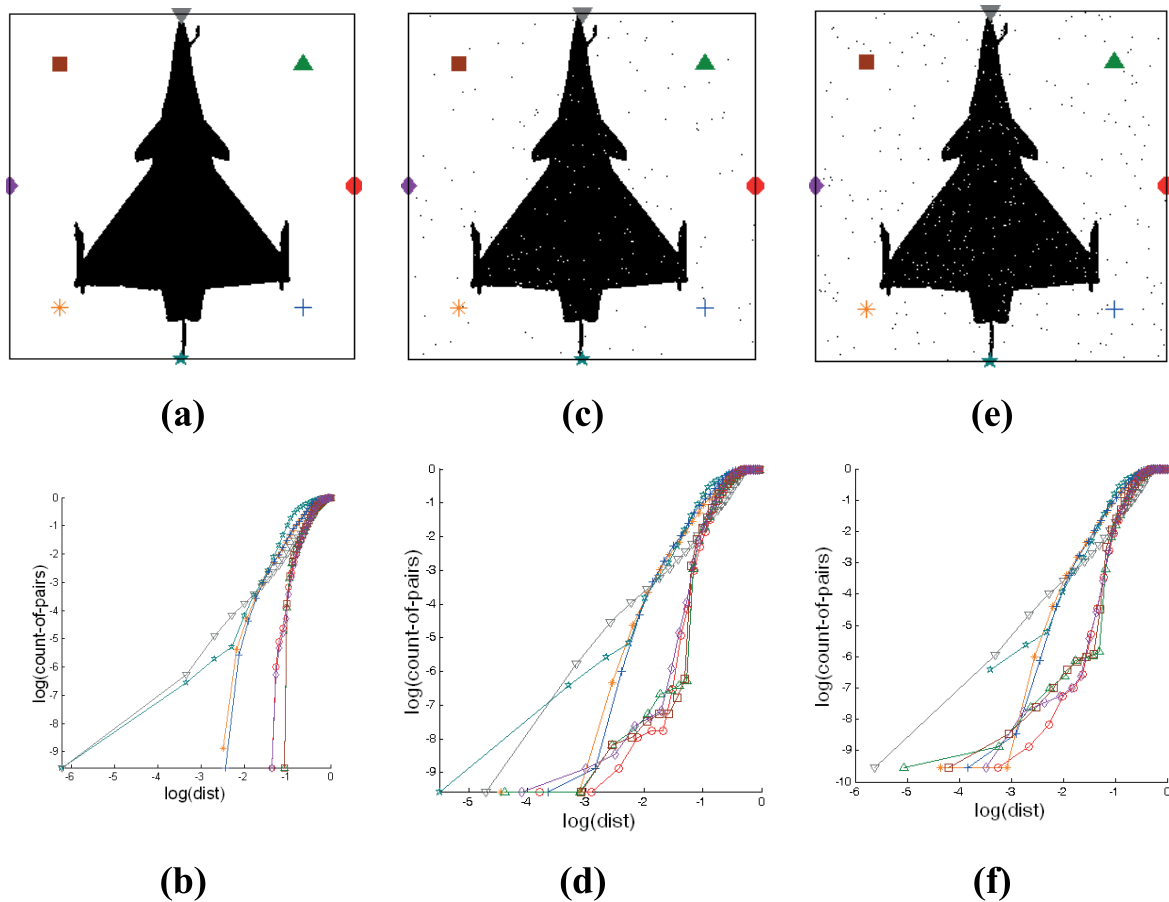
Figure 7. Effect of noise on Cross-plot based signatures. (a) Binary pattern of target without noise; (c) Binary pattern of target with SNR of 23dB; (e) Binary pattern of target with SNR at 20 dB; (b, d, f) are the Cross-plots of patterns from (a, c, e) respectively. doi:10.1371/journal.pone.0025621.g007
