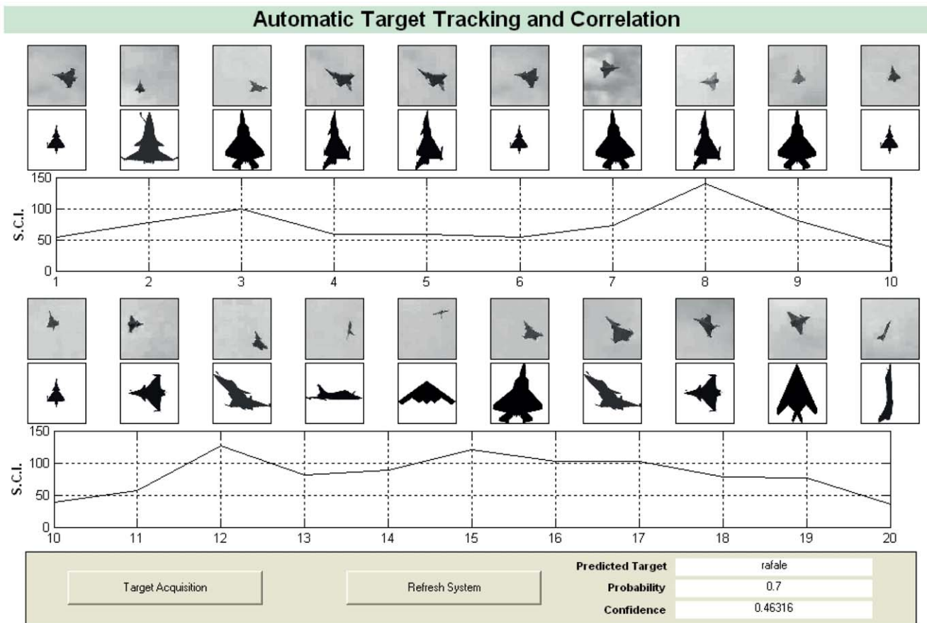
Figure 13. Correlation analysis of an airborne target based on acquired video clip. The data registration and feature extraction of a Dassault Rafale from a video database can be performed in real-time to consolidate sufficient content information of its shape. The time taken to verify its identity is in the order of milliseconds. The Shape Contrast Index (SCI) versus time graph demonstrates the variations in these indices as each image is captured per time frame increment. The probability and confidence of identification are output for decision makers. doi:10.1371/journal.pone.0025621.g013
