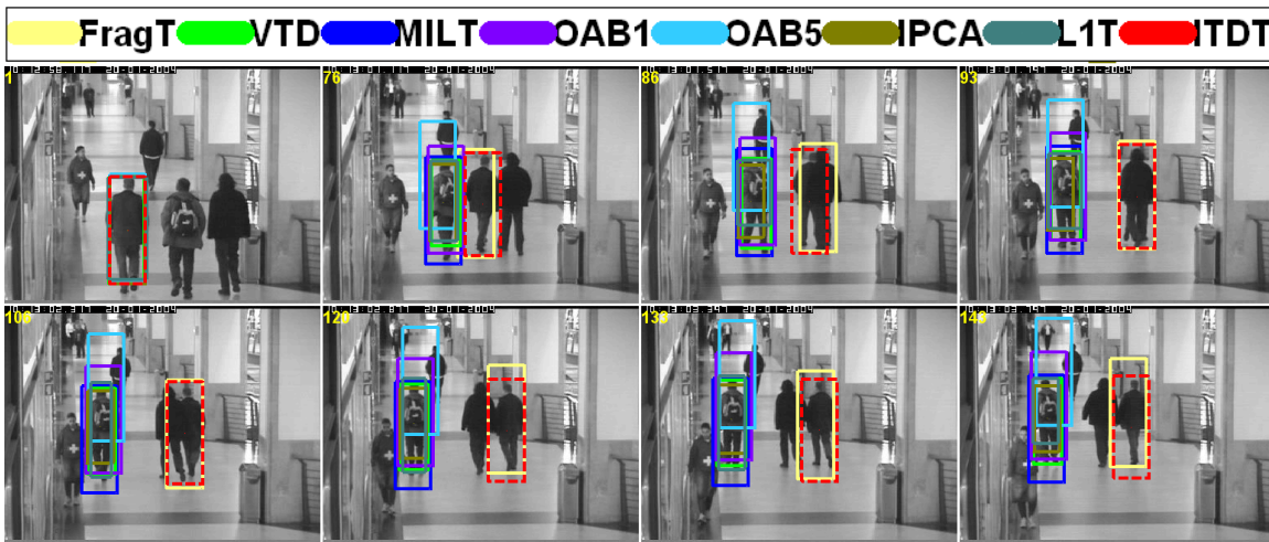
Fig. 11: The tracking results of the eight trackers over the representative frames (i.e., the 1st, 76th, 86th, 93rd, 106th, 120th, 133rd, and 143rd frames) of the “Sub-three-persons” video sequence [44] in the scenarios with severe occlusions.
