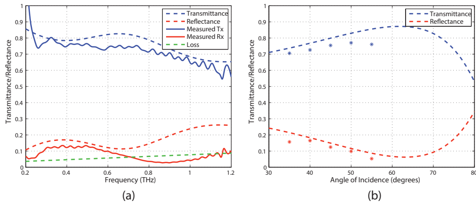
Fig. 6. Transmittance & reflectance plots of the PPY 1 \mu\text{m} thick sample. (a) Shows the transmittance & reflectance plot of the sample at 45° incidence, including the calculated loss, while (b) shows the angular dependence of the sample at varying angles of incidence at a fixed frequency of 0.5 THz. Again, as for the 1 \mu\text{m} PEDOT coating, the 1 \mu\text{m} thick PPY coating show a degradation of the reflectance compared to expectations because of the imperfect flatness of the sample.
