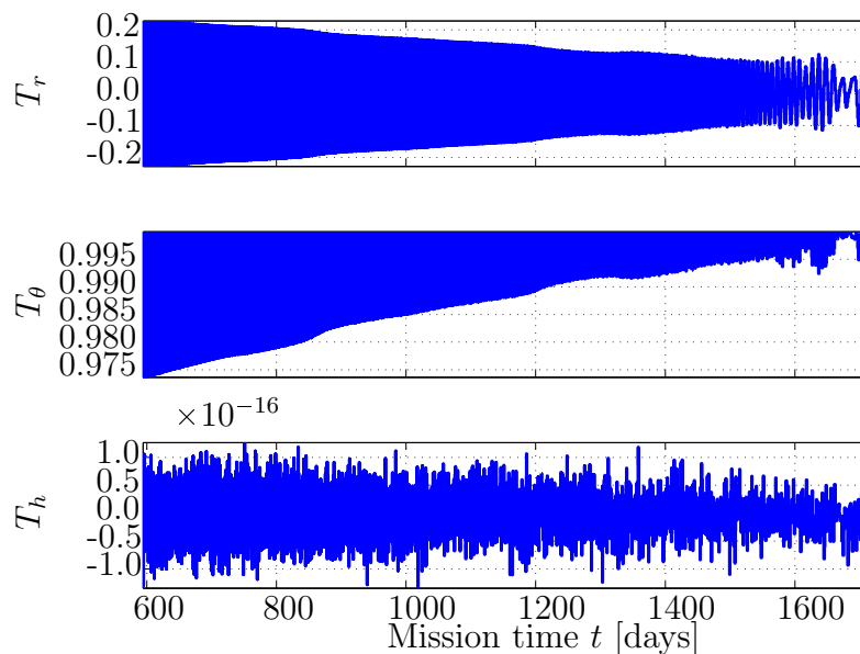
Figure 8.21: Direction of thrust vector during cruise phase.
