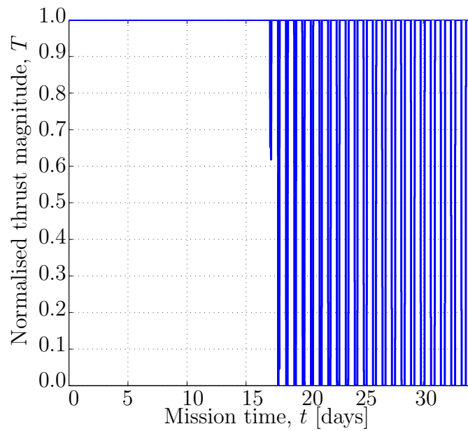
Figure 8.2: Magnitude of thrust vector shown in Figure 8.1 during reduced complexity ascent phase.
