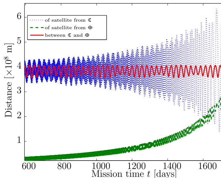
Figure 8.19: Satellite’s distance from Earth and Moon during cruise phase.
