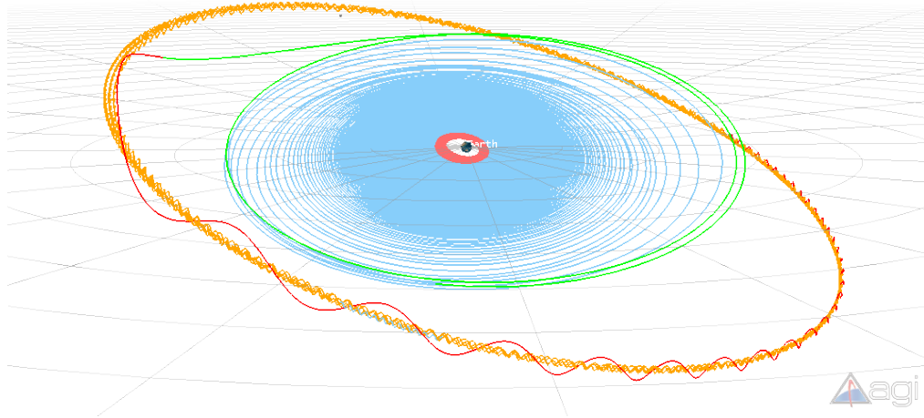
Figure 7.1: Continuous trajectory modelled in STK.
