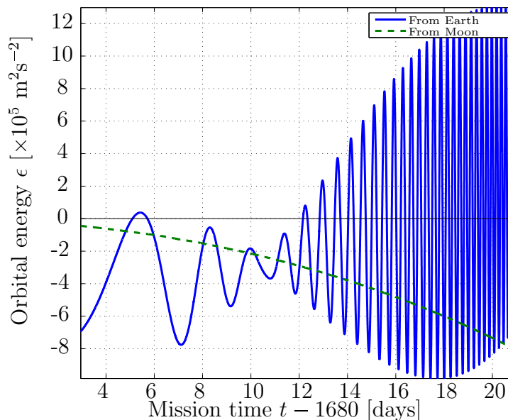
Figure 8.39: Orbital energy of the satellite relative to Earth and Moon during capture phase.
