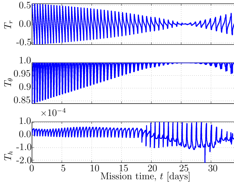
Figure 8.1: Direction of thrust vector during reduced complexity ascent phase. T_r is the radial component, T_\theta is the tangential component within the orbital plane, and T_h is the out-of-plane component.
