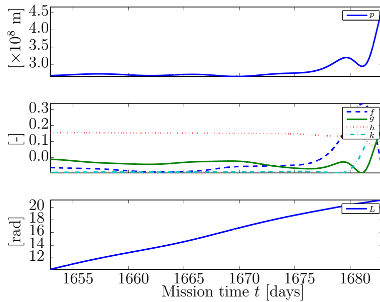
Figure 8.31: Equinoctial elements of satellite within ECI frame during propagate phase.
