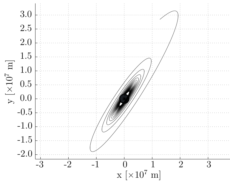
Figure 8.36: Capture trajectory of the satellite in LCI frame viewed from north pole.
