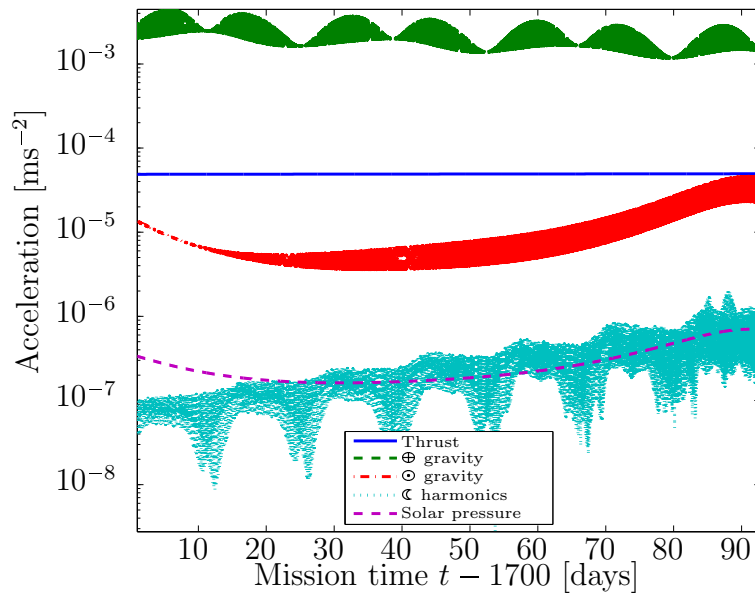
Figure 8.50a: Perturbing accelerations acting on spacecraft during descent phase.
