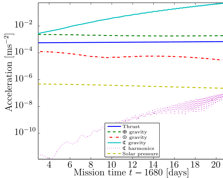
Figure 8.42a: Perturbing accelerations acting on spacecraft during capture phase.
