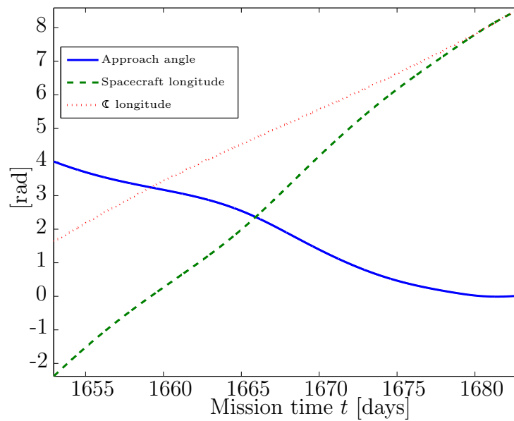
Figure 8.34: Longitude of spacecraft and Moon during propagate phase. The approach angle is the difference between spacecraft longitude and the Moon's longitude.
