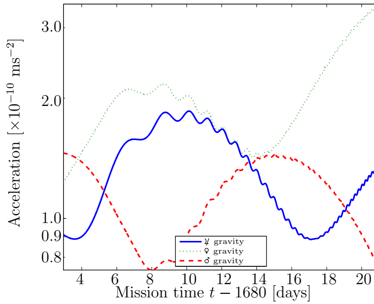
Figure 8.42b: Smaller magnitude perturbing accelerations acting on spacecraft during capture phase.
