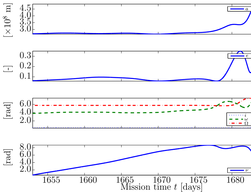
Figure 8.30: Keplerian elements of satellite within ECI frame during propagate phase.
