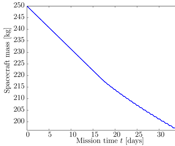
Figure 8.5: Mass of spacecraft during reduced complexity ascent phase.
