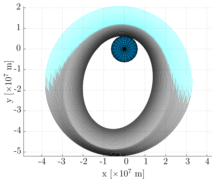
Figure 8.3: Reduced complexity ascent trajectory of the satellite in ECI frame viewed from north pole. Black represents full thrust magnitude, cyan represents zero thrust magnitude.
