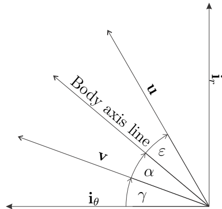
Figure 4.9: Flight angle \gamma , body orientation \alpha , and thrust vector angle \epsilon of the spacecraft relative to LVLH frame. \mathbf{i}_r and \mathbf{i}_\theta are the local vertical and horizontal, respectively (see Section 4.4 for definition). The thrust vector is \mathbf{u} and the velocity vector is \mathbf{v} . The body axis line represents the orientation of the vehicle.
