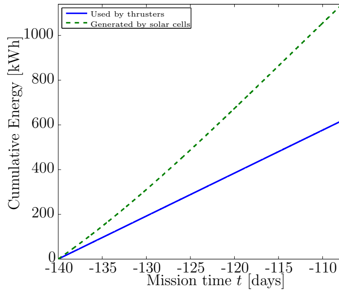
Figure 8.17: Power budget of spacecraft during ascent phase.
