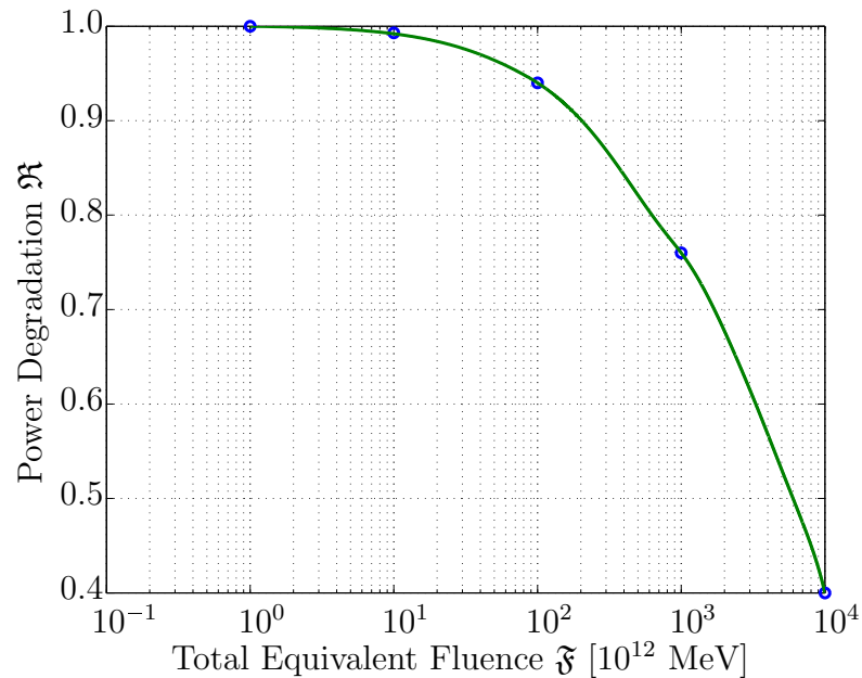
Figure 6.8: Power degradation as a consequence of radiation fluence, based on data from Erb (2002).
