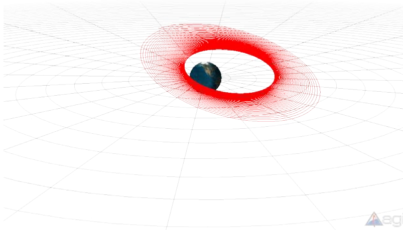
Figure 8.59: STK validation of ascent phase.
