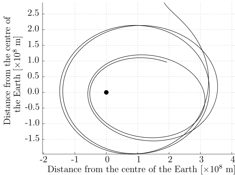
Figure 6.9: Trajectory of preliminary optimisation for Lunar Mission BW-1 showing a lunar resonance implicitly realised by the optimiser.
