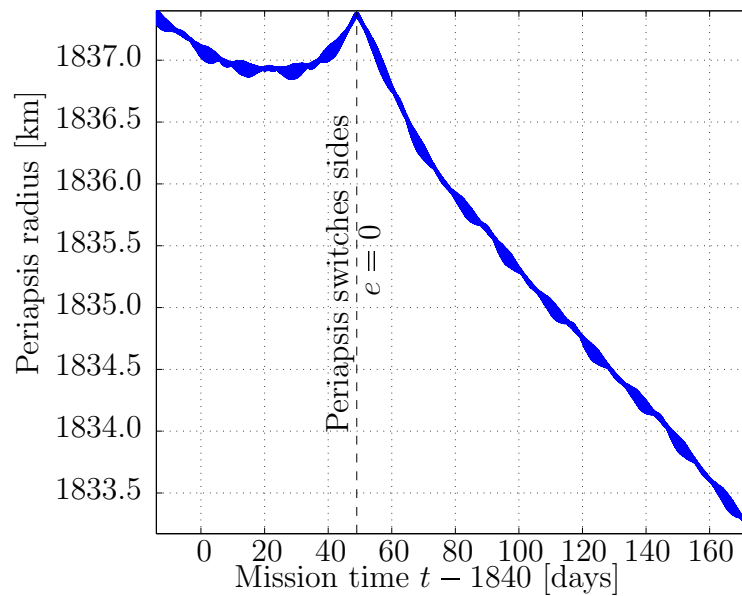
Figure 8.55: Periapsis of spacecraft during science phase. The periapsis switches from one side of the orbit to the other when e = 0 .
