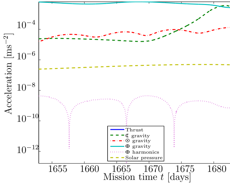
Figure 8.33: Perturbing accelerations acting on spacecraft during propagate phase.
