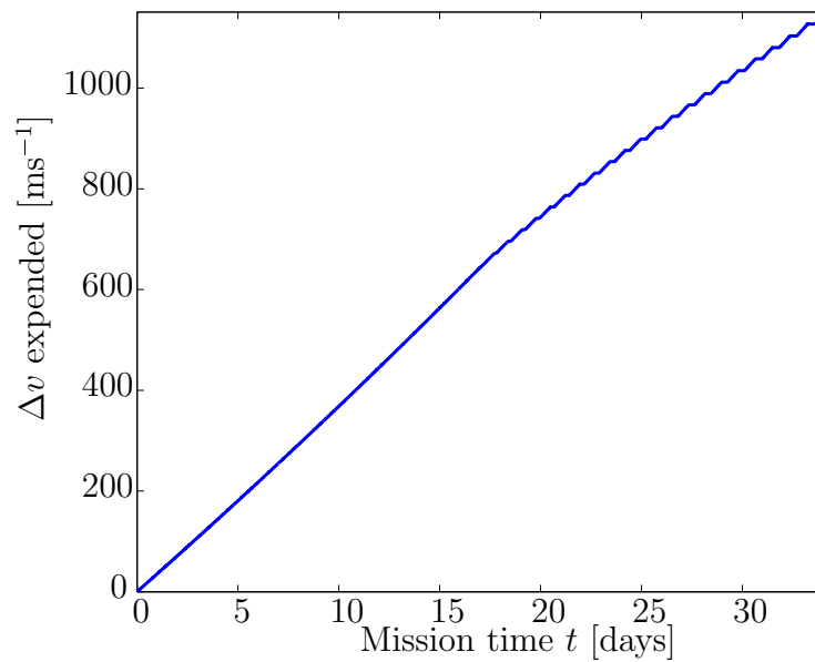
Figure 8.6: Delta-V generated by spacecraft during reduced complexity ascent phase.
