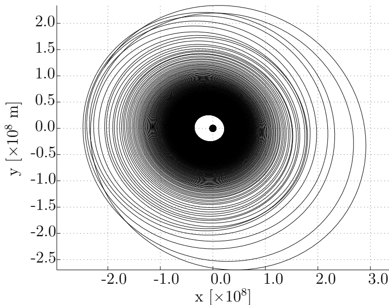
Figure 8.18: Cruise trajectory of the satellite in ECI frame viewed from north pole.
