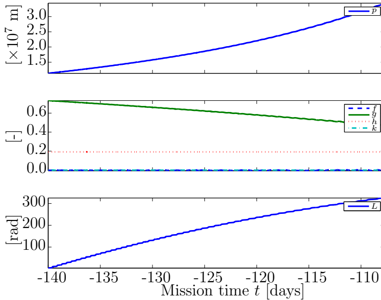
Figure 8.12: Equinoctial elements of satellite within ECI frame during ascent phase.
