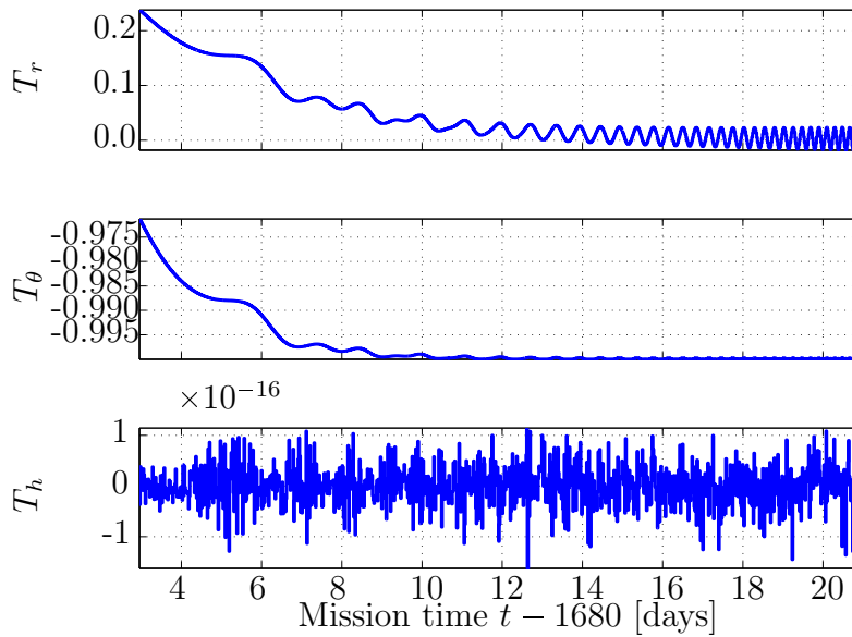
Figure 8.43: Direction of thrust vector during capture phase.
