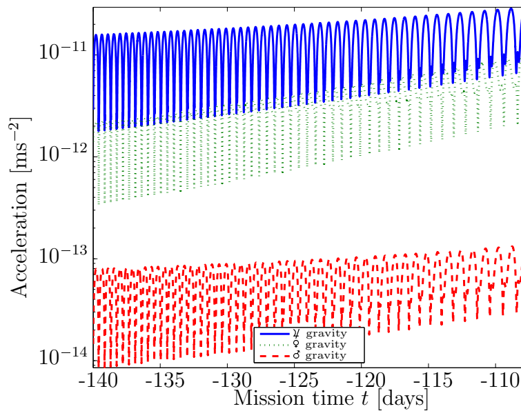
Figure 8.14b: Smaller magnitude perturbing accelerations acting on spacecraft during ascent phase.
