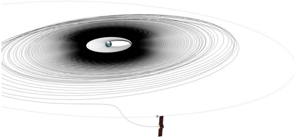
Figure 2.1: A simplified trajectory prepared for demonstration purposes early in the Kleinsatelliten program.
