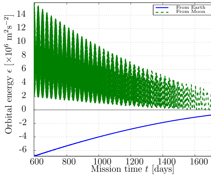
Figure 8.20a: Orbital energy of the satellite relative to Earth and Moon during cruise phase.
