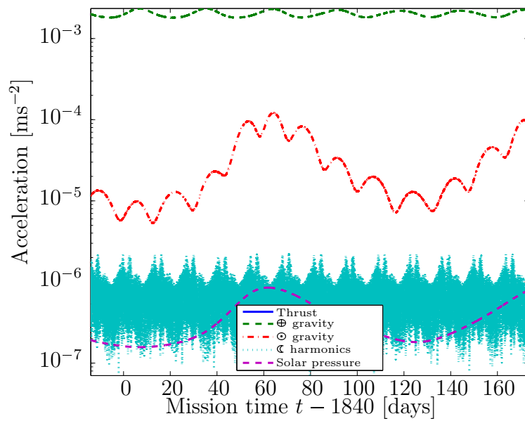
Figure 8.57: Perturbing accelerations acting on spacecraft during science phase.
