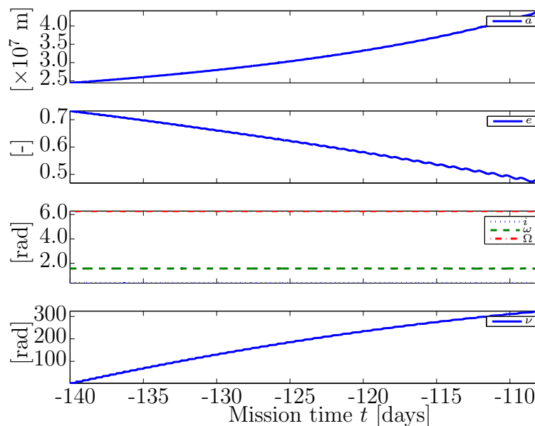
Figure 8.13: Keplerian elements of satellite within ECI frame during ascent phase.
