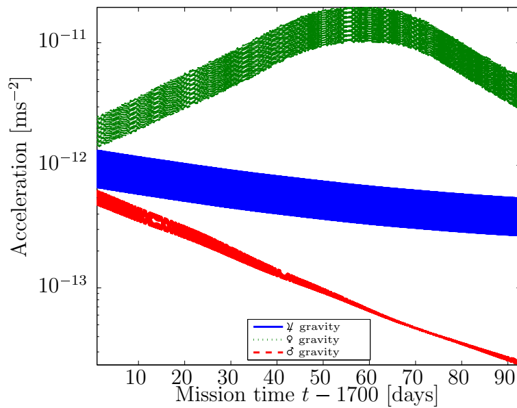
Figure 8.50b: Smaller magnitude perturbing accelerations acting on spacecraft during descent phase.
