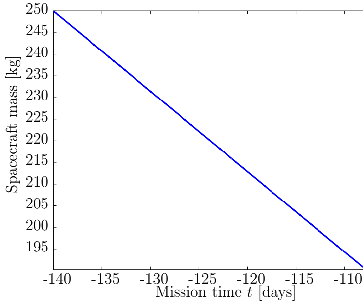
Figure 8.16: Mass of spacecraft during ascent phase.
