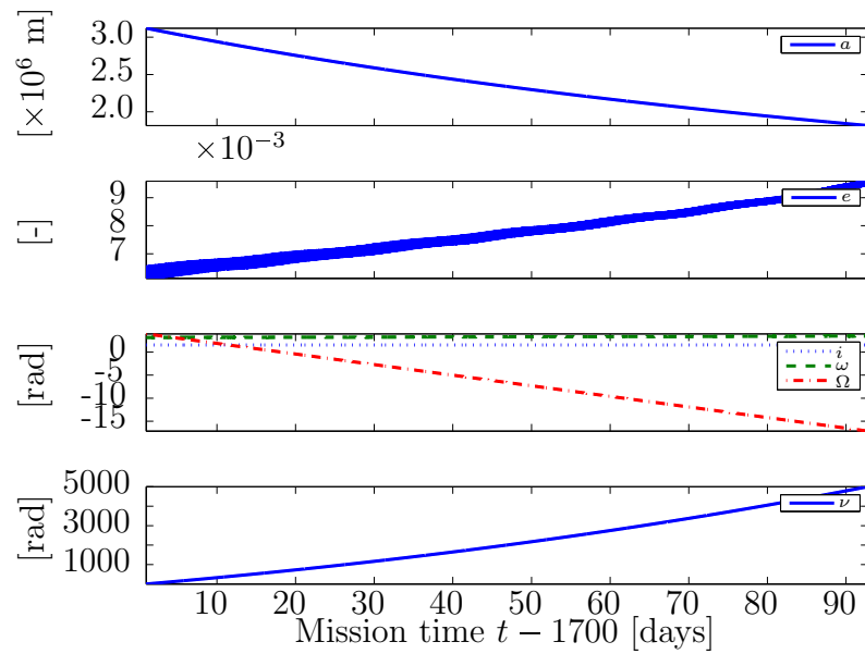
Figure 8.48: Keplerian elements of satellite within LCI frame during descent phase.
