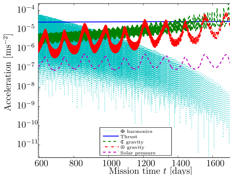
Figure 8.24a: Perturbing accelerations acting on spacecraft during cruise phase.
