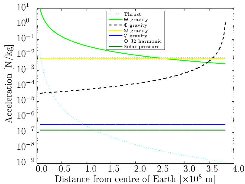
Figure 4.8: Upper limit on perturbing forces in the region between the Earth and the Moon.
