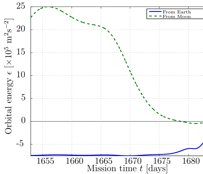
Figure 8.29: Orbital energy of the satellite relative to Earth and Moon during propagate phase.
