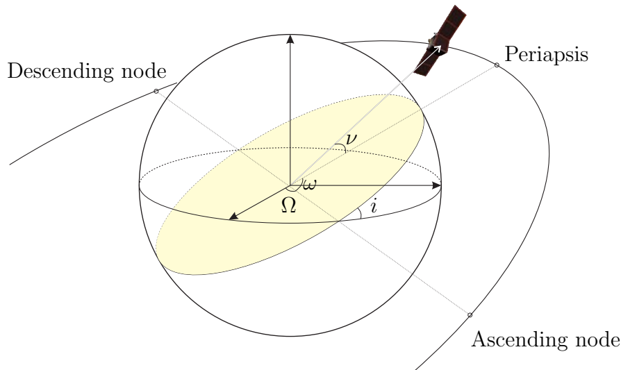
Figure 4.6: Keplerian orbital elements. Semimajor axis a and eccentricity e define the shape of the elliptical orbit. Inclination i represents the angle between the orbital plane from the equatorial plane, while right ascension of the ascending node \Omega defines the axis along which the orbital plane is inclined, relative to the vernal equinox. The argument of periapsis \omega defines the orientation of the orbit within this plane, by locating the periapsis relative to the ascending node. The true anomaly \nu was defined in Figure 4.5.
