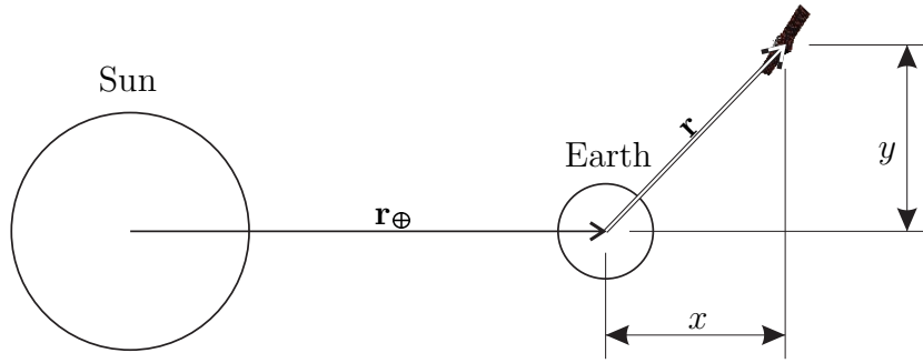
Figure 6.6: Spacecraft position \mathbf{r} broken down into components x and y relative to Earth-Sun line \mathbf{r}_\oplus .
