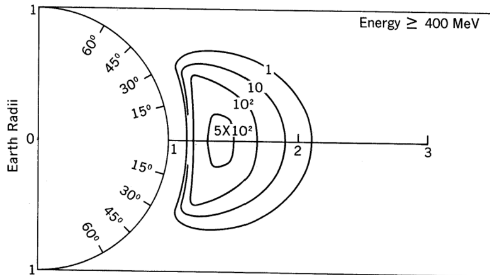
Figure 4.12: NASA's AP8MIN van Allen Belt proton flux distribution model (Sawyer and Vette 1976). Contours represent particles per square centimetre per second.
