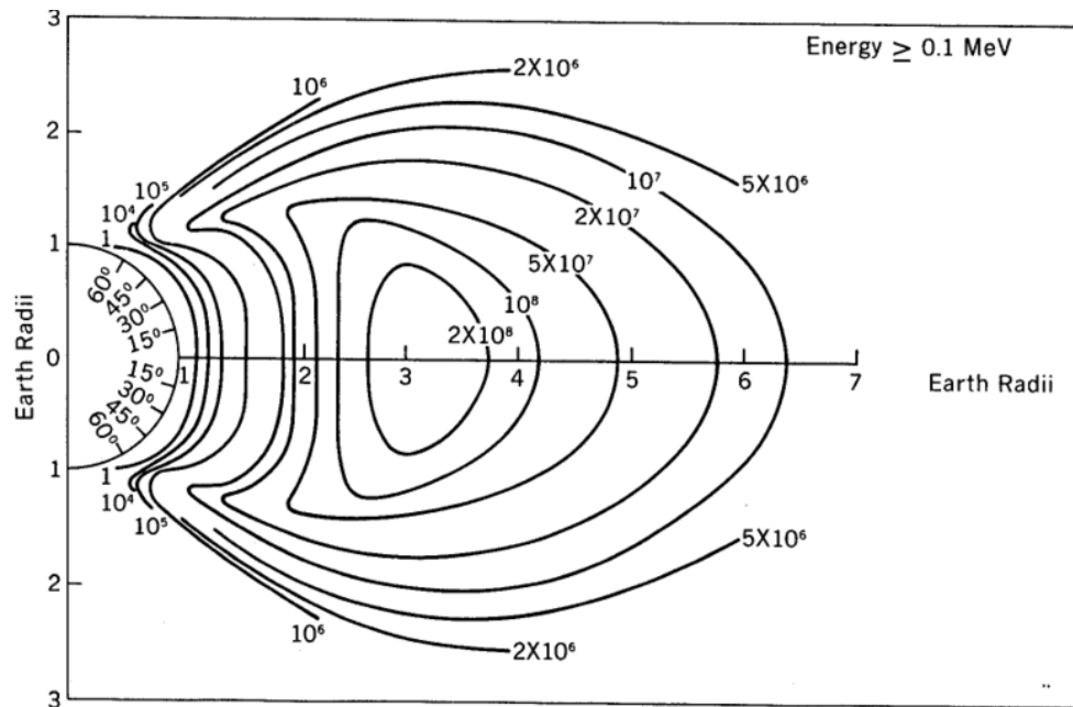
Figure 4.11: NASA's AP8MIN van Allen Belt proton flux distribution model (Sawyer and Vette 1976). Contours represent particles per square centimetre per second.
