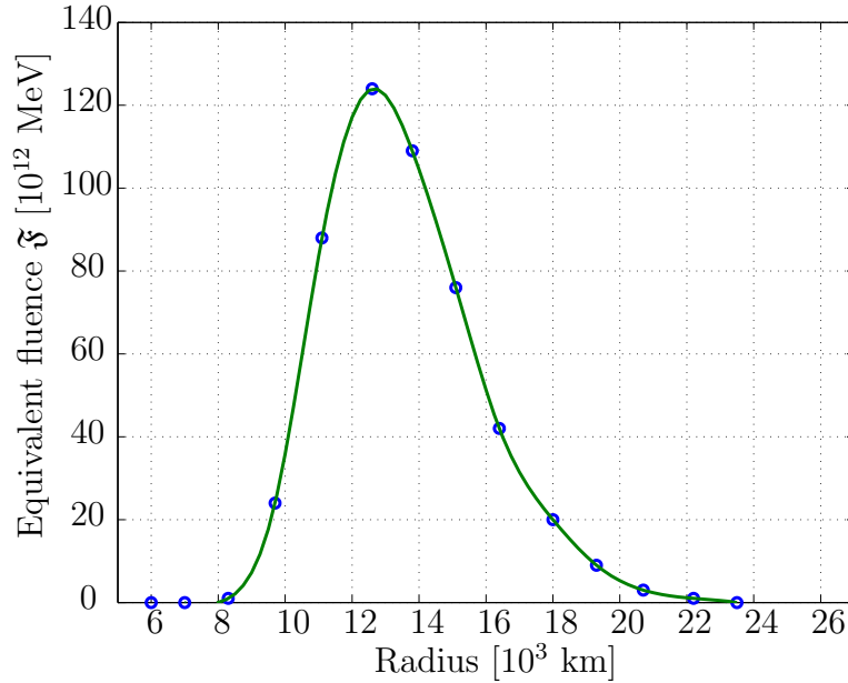
Figure 6.7: Radiation fluence during a 24 hour orbit as a function of distance from Earth, based on data from Erb (2002). The obvious peak is due to the higher concentration of radiation in the van Allen belt.
