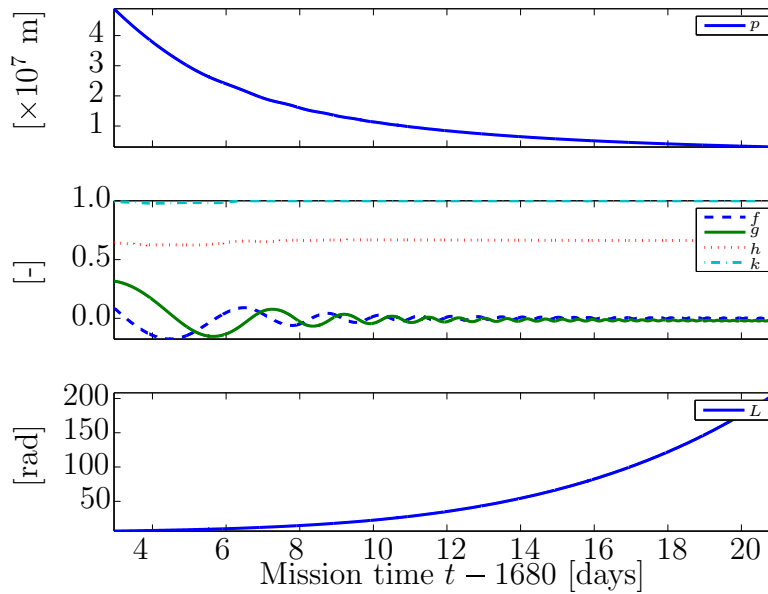
Figure 8.41: Equinoctial elements of satellite within LCI frame during capture phase.
