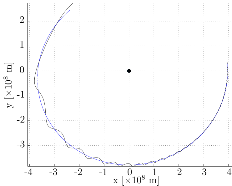
Figure 8.35: Capture trajectory of the satellite in ECI frame viewed from north pole. The Moon's orbit is shown in blue.
