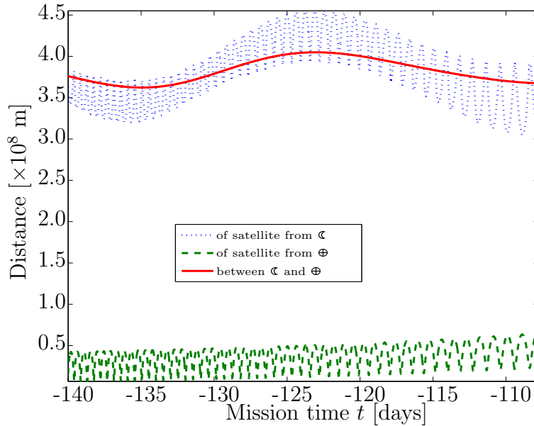
Figure 8.9: Satellite's distance from Earth and Moon during ascent phase.
