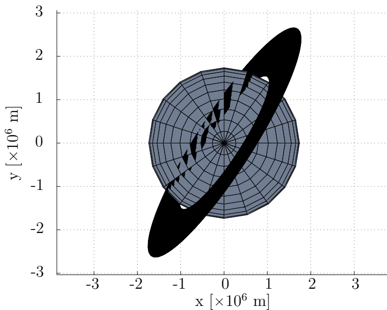
Figure 8.44: Descent trajectory of the satellite in LCI frame viewed from north pole. The orbits behind the Moon partly show through due to a flaw in the vector graphics renderer.
