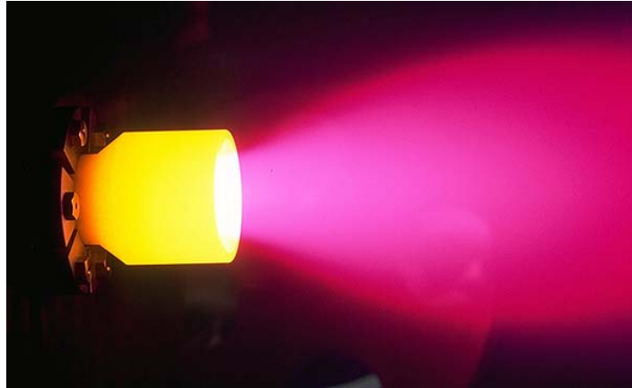
Figure 6.2: TALOS arcjet during a laboratory test. An arc is generated between the axial cathode and the nozzle anode, which heats up the ammonia, accelerating it outwards.
