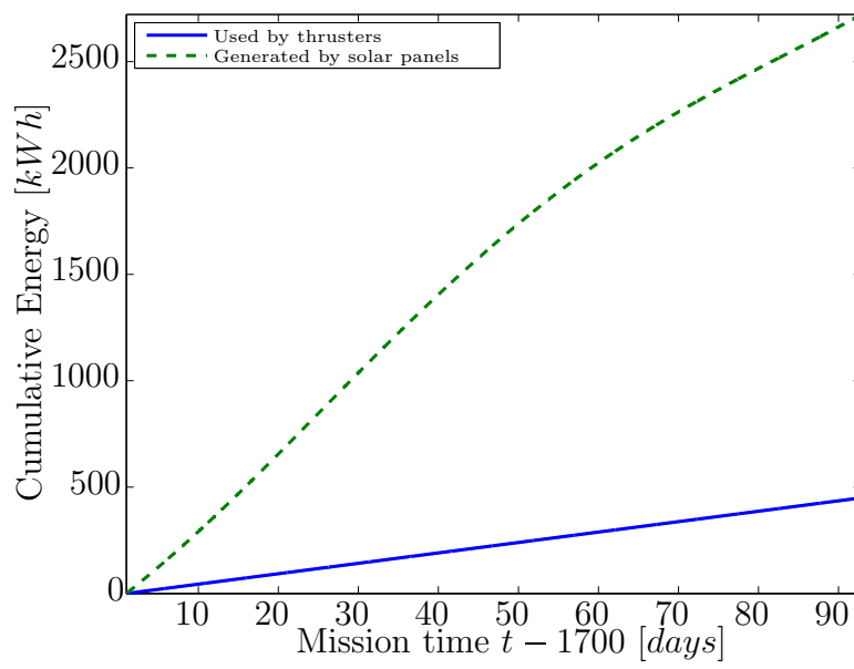
Figure 8.52: Power budget of spacecraft during descent phase.
