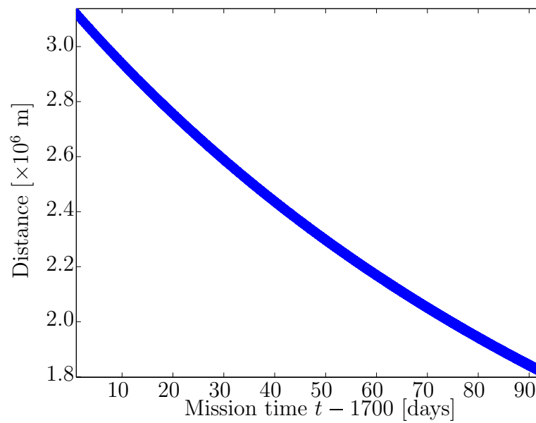
Figure 8.46: Satellite's distance from the Moon during descent phase.
