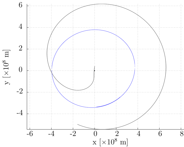
Figure 8.26: Propagated trajectory of the satellite in LCI frame viewed from north pole. The Earth's orbit is shown in blue.
