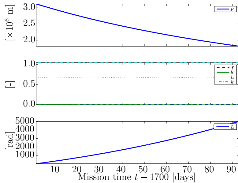
Figure 8.49: Equinoctial elements of satellite within LCI frame during descent phase.
