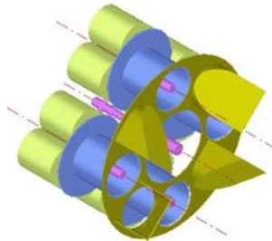
Figure 1.2: Arrangement of arcjet (centre) and 4 PPTs on Lunar Mission BW-1, with a conceptual mechanism allowing for thrust vectoring. Image used courtesy of Röser et al. (2006).
