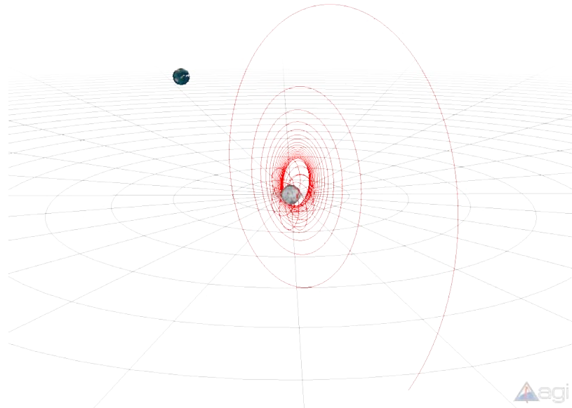
Figure 8.61: STK validation of capture phase.
