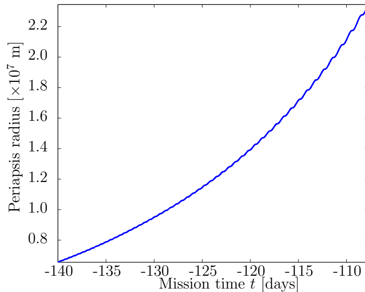
Figure 8.15: Periapsis of spacecraft during ascent phase.
