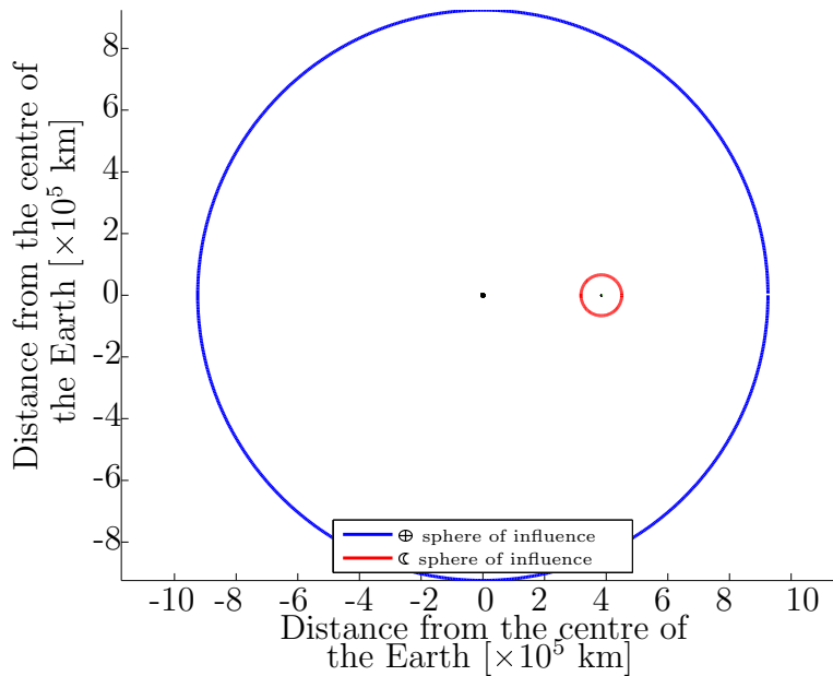
Figure 4.2: Earth and Moon spheres of influence.
