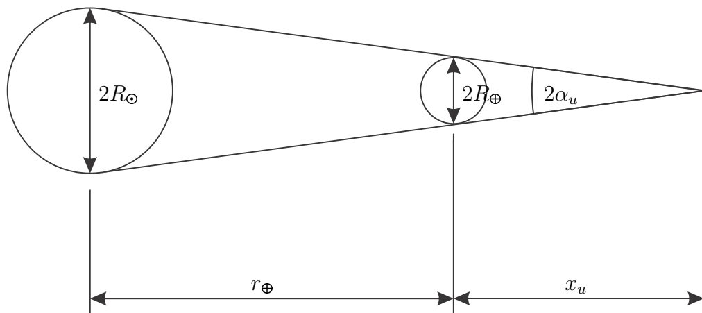
Figure 6.4: Geometry associated with the umbral cone. R_{\odot} and R_{\oplus} are the radii of the Sun and the Earth respectively. The distance between the Earth and the Sun is r_{\oplus} , allowing the calculation of the length of the umbral cone x_u and the apex angle \alpha_u .
