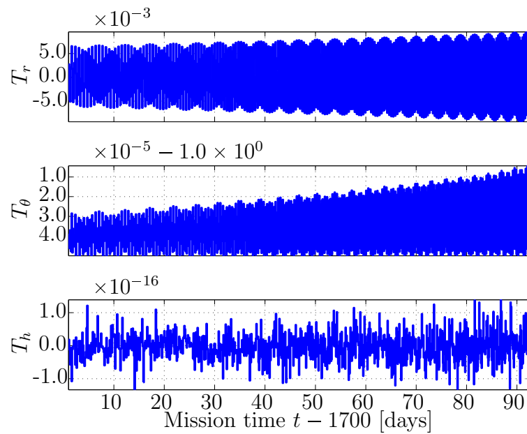
Figure 8.51: Direction of thrust vector during descent phase.
