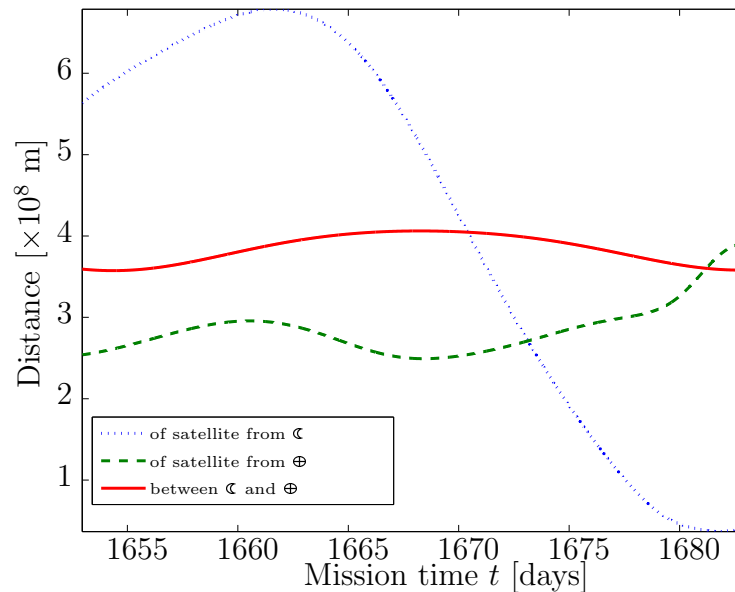
Figure 8.28: Satellite's distance from Earth and Moon during propagate phase.
