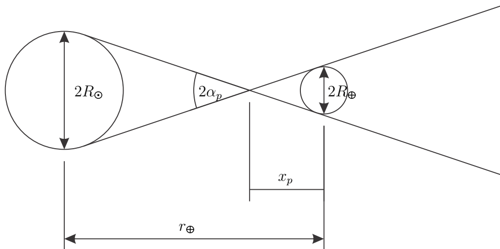
Figure 6.5: Geometry associated with the penumbral cone. R_{\odot} and R_{\oplus} are the radii of the Sun and the Earth respectively. The distance between the Earth and the Sun is r_{\oplus} , allowing the calculation of the length of the penumbral cone x_p and the apex angle \alpha_p .
