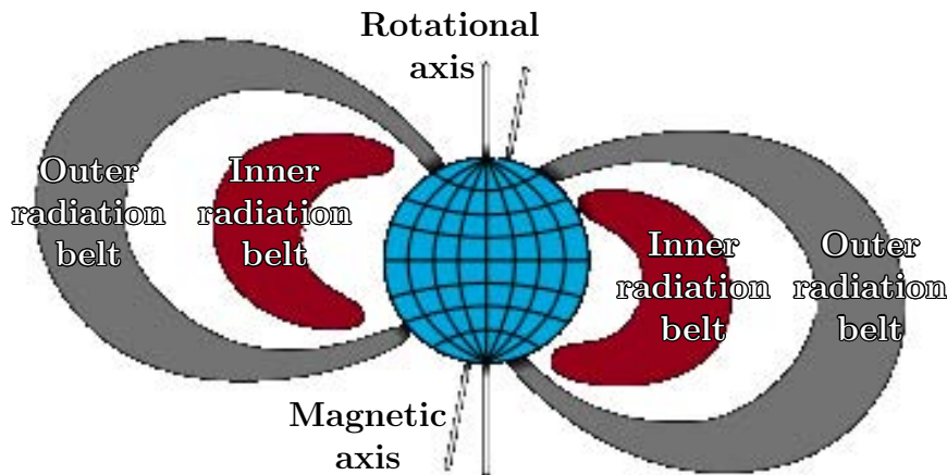
Figure 4.10: Conceptual image of the van Allen belts.
