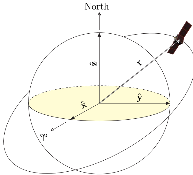
Figure 4.4: Earth-Centred Inertial frame. Axes \hat{\mathbf{x}} , \hat{\mathbf{y}} , \hat{\mathbf{z}} represent the J2000.0 frame, where \hat{\mathbf{x}} points towards the vernal equinox \varphi and \hat{\mathbf{z}} points through the North pole of the Earth.
