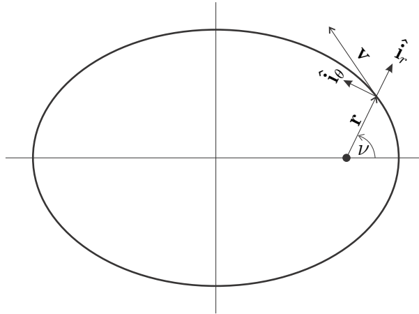
Figure 4.5: Local Gauss frame. Vector \mathbf{v} represents the spacecraft's velocity. Vector \mathbf{r} represents the spacecraft's position relative to the primary body. True anomaly \nu represents the angle of this position relative to the periapsis.
