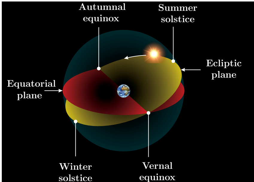
Figure 4.3: Ecliptic and equatorial planes. From an Earth-centred frame, the Sun appears to orbit the Earth. The plane of its orbit is the ecliptic plane. The solstices and equinoctia are labelled based on the northern hemisphere seasons.
