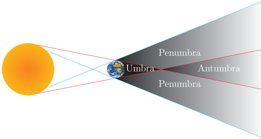
Figure 6.3: Umbra, penumbra and antumbra.
