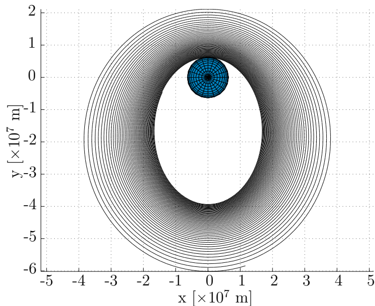
Figure 8.8: Ascent trajectory of the satellite in ECI frame viewed from north pole.
