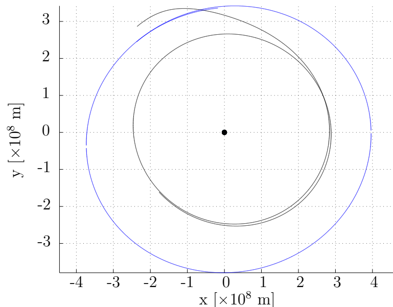
Figure 8.25: Propagated trajectory of the satellite in ECI frame viewed from north pole. The Moon's orbit is shown in blue.
