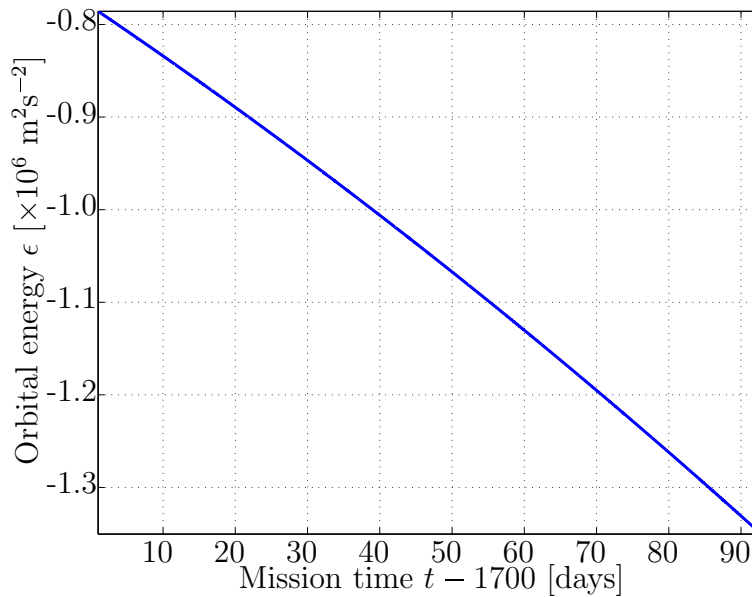
Figure 8.47: Orbital energy of the satellite relative to the Moon during descent phase.
