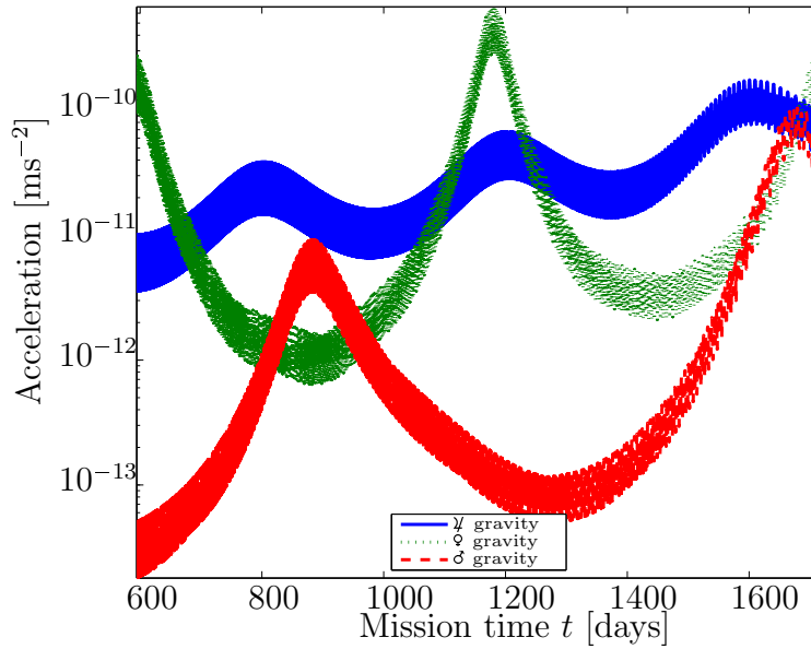
Figure 8.24b: Smaller magnitude perturbing accelerations acting on spacecraft during cruise phase.
