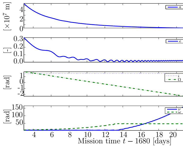
Figure 8.40: Keplerian elements of satellite within LCI frame during capture phase.
