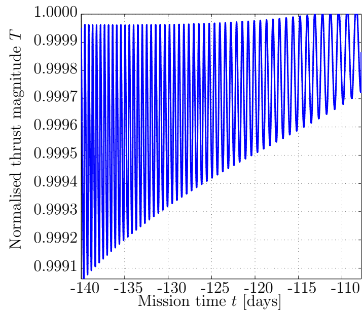
Figure 8.11: Magnitude of thrust vector during ascent phase.
