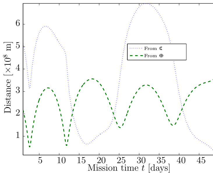
Figure 6.10: Distance of spacecraft from Earth and Moon during preliminary optimisation showing a lunar resonance implicitly realised by the optimiser.
