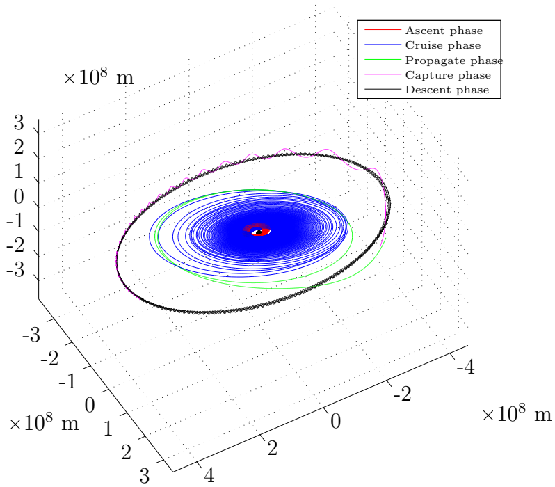
Figure 8.58: The complete GESOP trajectory shown in an ECI frame, with orthographic view.
