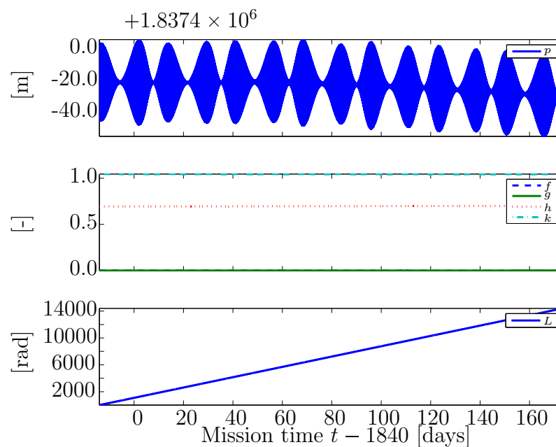
Figure 8.56: Equinoctial elements of satellite within ECI frame during science phase.
