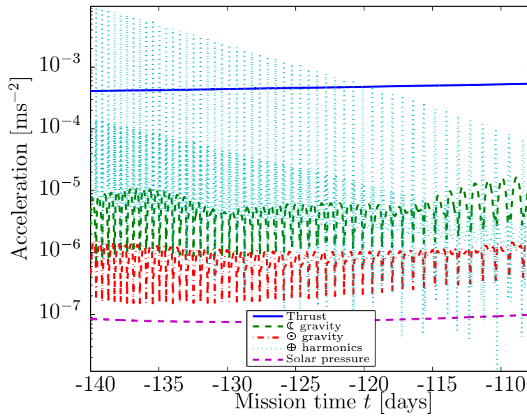
Figure 8.14a: Perturbing accelerations acting on spacecraft during ascent phase.
