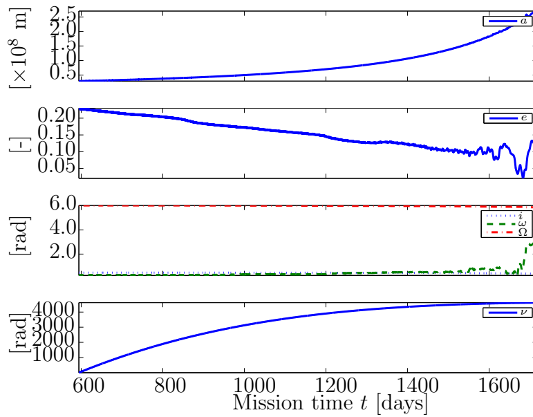
Figure 8.22: Keplerian elements of satellite within ECI frame during cruise phase.
