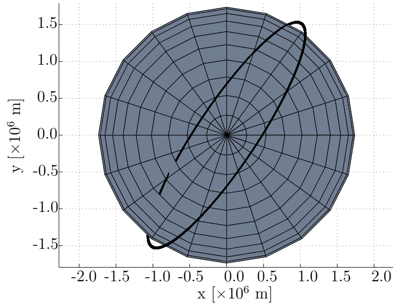
Figure 8.53: Science trajectory of the satellite in LCI frame viewed from north pole. The orbits behind the Moon partly show through due to a flaw in the vector graphics renderer.
