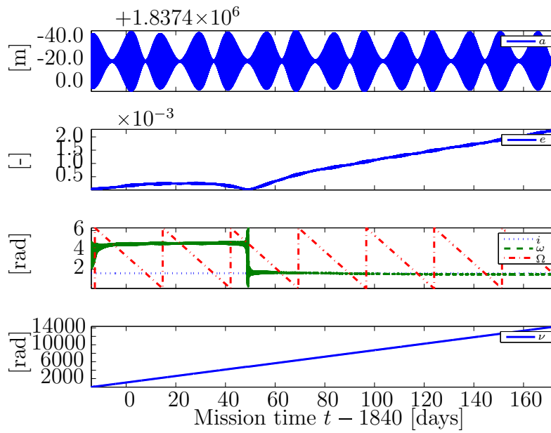
Figure 8.54: Keplerian elements of satellite within LCI frame during science phase.
