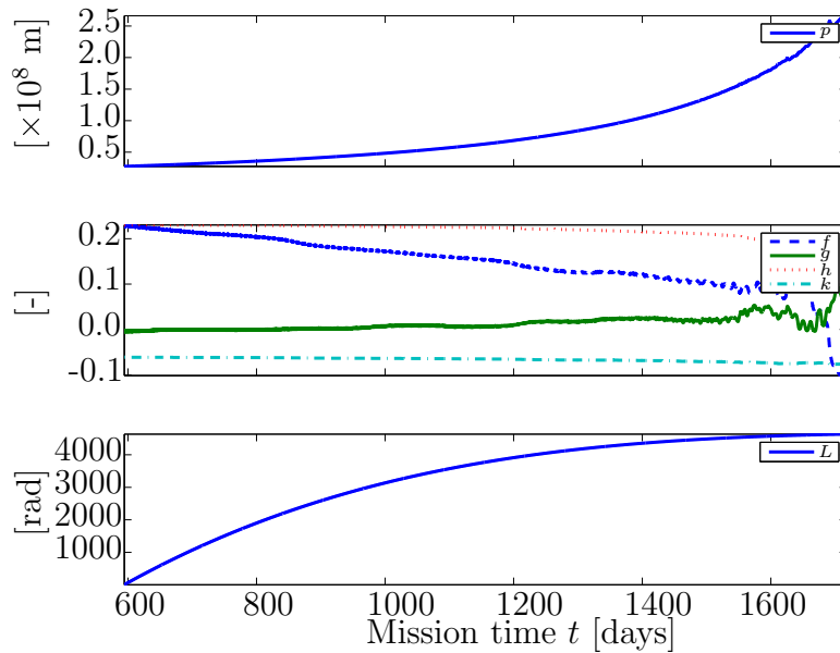
Figure 8.23: Equinoctial elements of satellite within ECI frame during cruise phase.
