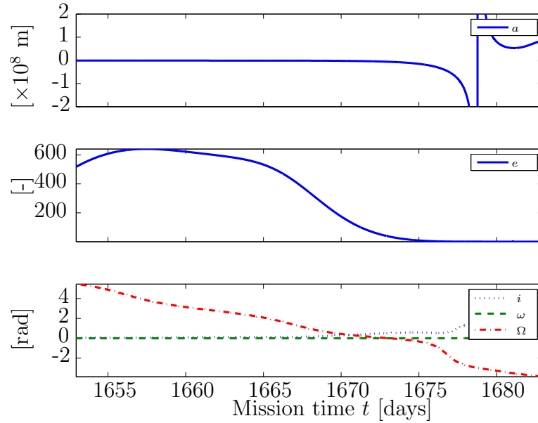
Figure 8.32: Keplerian elements of satellite within LCI frame during propagate phase.
