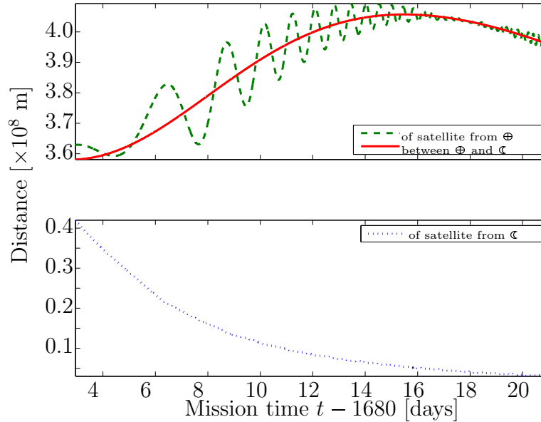
Figure 8.38: Satellite's distance from Earth and Moon during capture phase.
