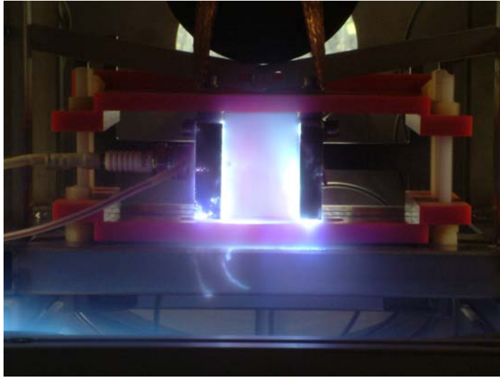
Figure 6.1: SIMPLEX PPT during a laboratory test. The spark plug (centre left) ignites an arc between the two electrodes (pointing towards the camera) which vapourises the surface of the block of white PTFE between them. The electric field between the two electrodes then accelerates the plasma towards the camera.
