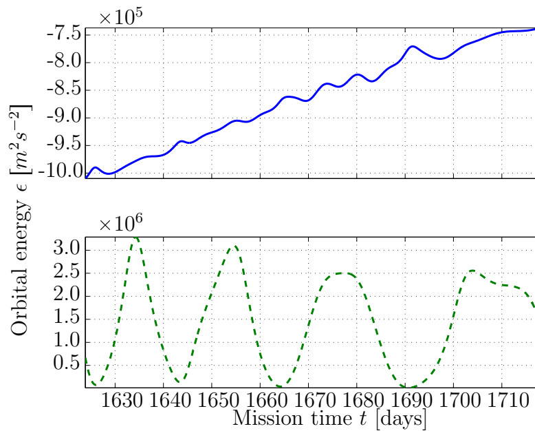
Figure 8.20b: Orbital energy of the satellite relative to Earth and Moon during cruise phase (zoomed in).
