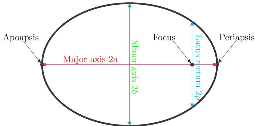
Figure 4.1: Elliptical parameters.
