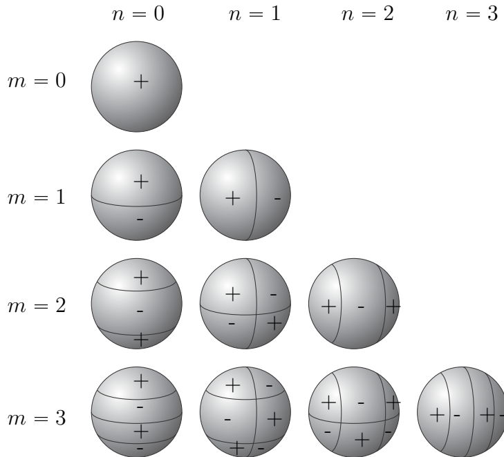
Figure 4.7: Spherical Harmonics. The degree of the zonal harmonic is m , and the order of the sectorial harmonic is n .
