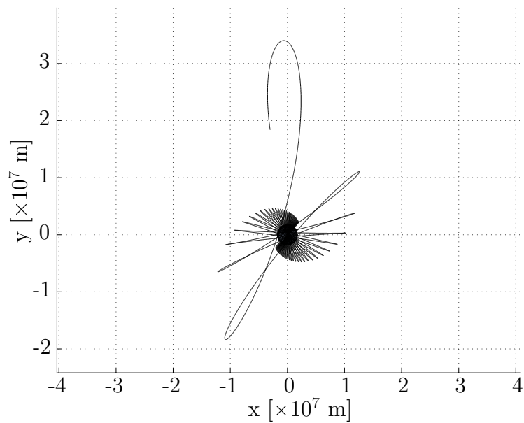
Figure 8.37: Capture trajectory of the satellite in SEL frame viewed from north pole.
