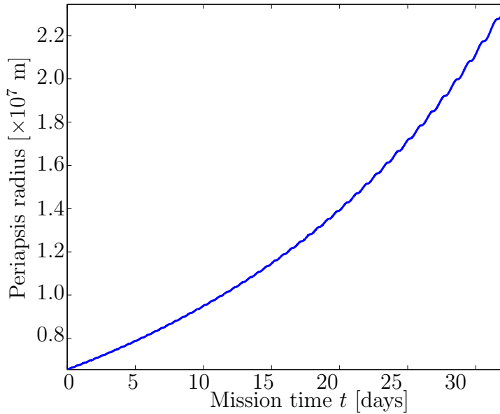
Figure 8.4: Periapsis of spacecraft during reduced complexity ascent phase.
