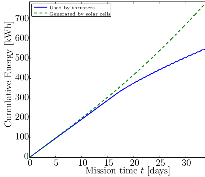
Figure 8.7: Power budget of spacecraft during reduced complexity ascent phase.
