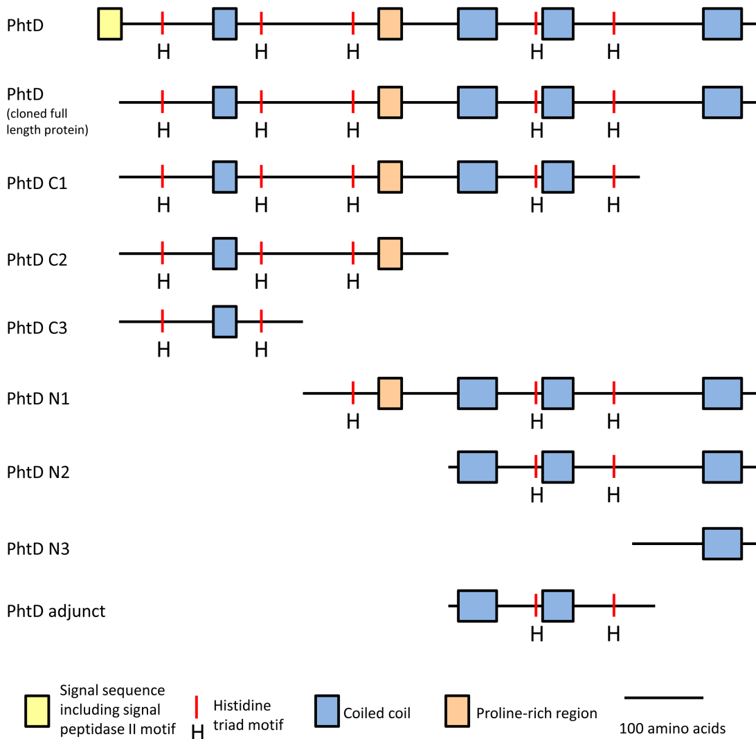
Figure 2. Truncated forms of PhtD used in this study. Proteins are shown with known or predicted domains annotated. The N termini are to the left. doi:10.1371/journal.pone.0078916.g002
