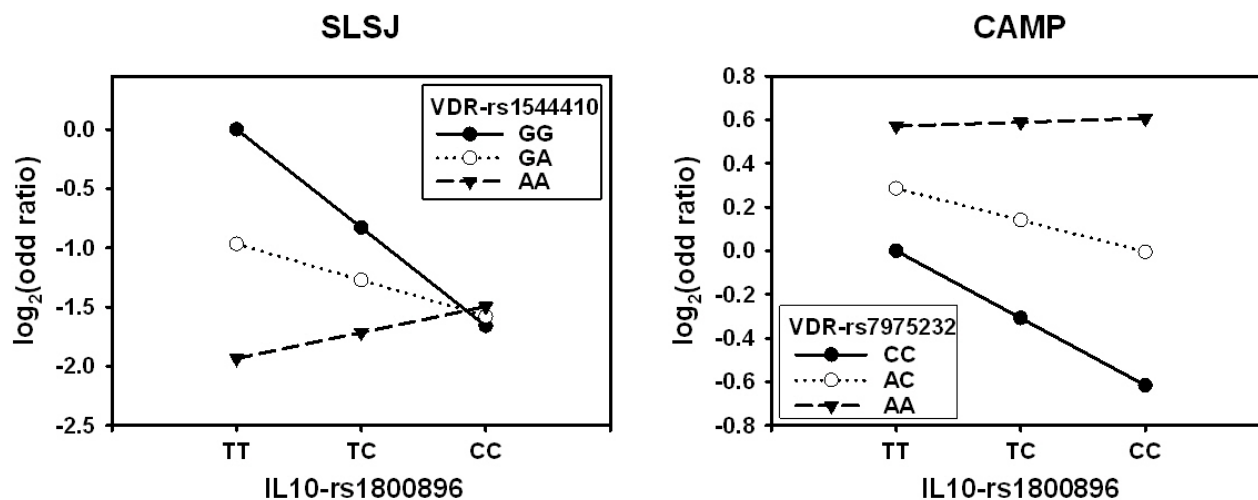
Figure 6 Two-gene models on asthma involving the IL10 and VDR genes in the SLSJ and the CAMP studies. With two bi-allelic SNPs (3 genotypes per SNP), a 3 by 3 odds ratio matrix is calculated and visually represented. The y-axis shows the odds ratio on a \log_2 scale, which makes the odds ratio above and below 1 on the same visual scale. The IL10 genotypes are illustrated on the x-axis. Different panels of SNPs were genotyped between the two studies and the comparison for the VDR gene is made with different SNPs that are in LD ( D' = 1.0 and r^2 = 0.59 , based on the HapMap CEU genotyping dataset). In the SLSJ study, the risks are evaluated relative to the VDR -GG and IL10 -TT genotypes. In CAMP, the risks are evaluated relative to the VDR -CC and IL10 -TT genotypes.
