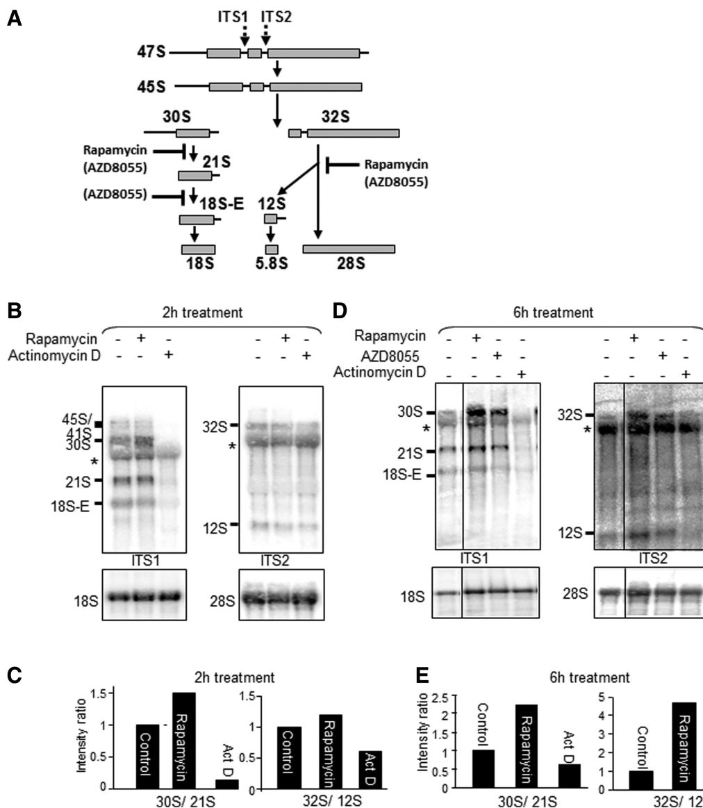
Figure 3. Rapamycin affects pre-rRNA processing in HeLa cells. (A) Schematic diagram of pre-rRNA processing pathways in HeLa cells. Structure of the primary 47S rRNA transcript containing two internal transcriber spacers (ITS1 and ITS2) and two external transcribed spacers. The 47S pre-rRNA is processed through intermediate precursors to mature 18S, 28S and 5.8S rRNAs. The locations of the probes used are shown (ITS1 and ITS2). (B and D) Effects of rapamycin and AZD8055 (each used at 100 nM) on rRNA processing in serum-fed cells. Northern hybridization of total RNA from HeLa cells after treatment with rapamycin or actinomycin D (20 ng/ml). After 2–6 h treatment (as indicated), total RNA was extracted and subjected to northern blotting analysis for pre-rRNA species. Membranes were hybridized with the ITS1 and ITS2 probes and probes for 18S and 28S rRNAs. The asterisk indicates cross-reaction with 28S rRNA and the vertical line denotes that these are non-adjacent lanes from the same gel/northern blot. (C and E) Ratios of different pre-rRNA species. Bar graphs show signal quantification using a phosphorimager and the bars indicate the ratios of 30S to 21S and 32S to 12S after rapamycin or actinomycin D treatment.
