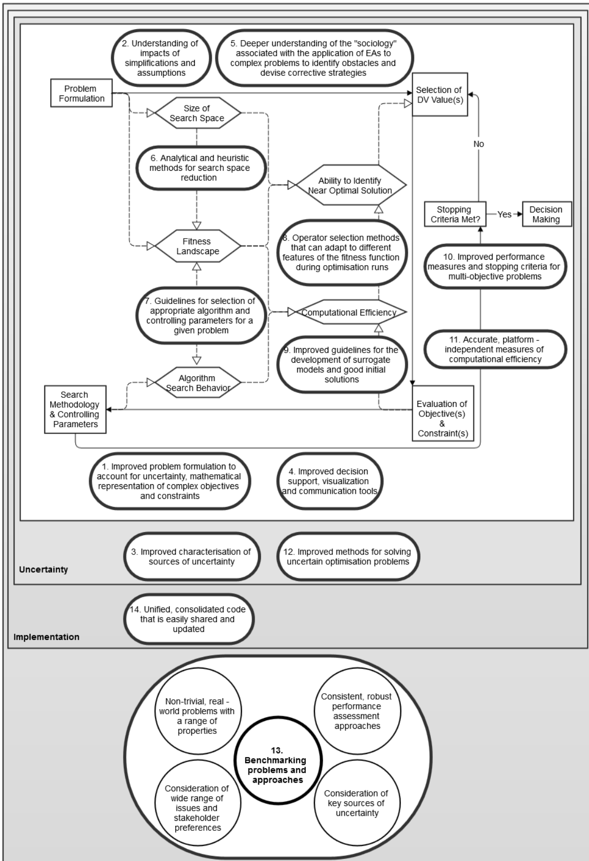
Figure 4: Roadmap of future research challenges and directions for the application of evolutionary algorithms in water resources. The square shapes represent the steps in the EA process and the hexagonal shapes represent problem and algorithm characteristics resulting from choices made at different steps of
