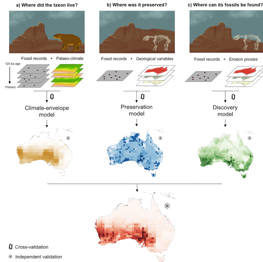
Fig 1. Approach to identify potential fossil areas with combined models. For a given taxon, the areas with greatest potential to yield new fossils (red map) are those where the species used to live (brown map), where its fossils could be preserved (blue map), and where it is now possible to find its fossils (green map). (a) We used palaeo-climate data and fossil records with reliable ages to model the climate envelope of different genera of the Australian megafauna, geological variables to model the suitability for fossil preservation (b) and erosion proxies to model the suitability for fossil discovery (c). The average of the suitability rankings predicted by the climate-envelope, preservation, and discovery models can be used as an indicator of the potential of an area to yield new fossils of a given taxon. We cross-validated each model and used an independent subset of the data to validate the final predictions of each model and their combination.
