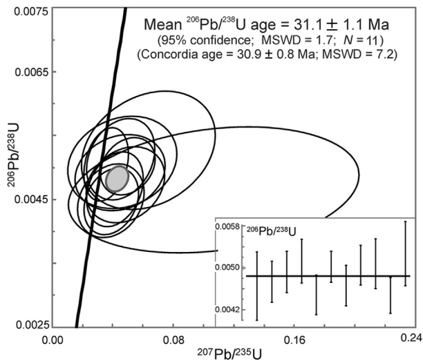
Figure 4. Concordia plot for LA-ICP-MS zircon U/Pb measurements on sample “GR” with indication of average ^{206}\text{Pb}/^{238}\text{U} ratio.
