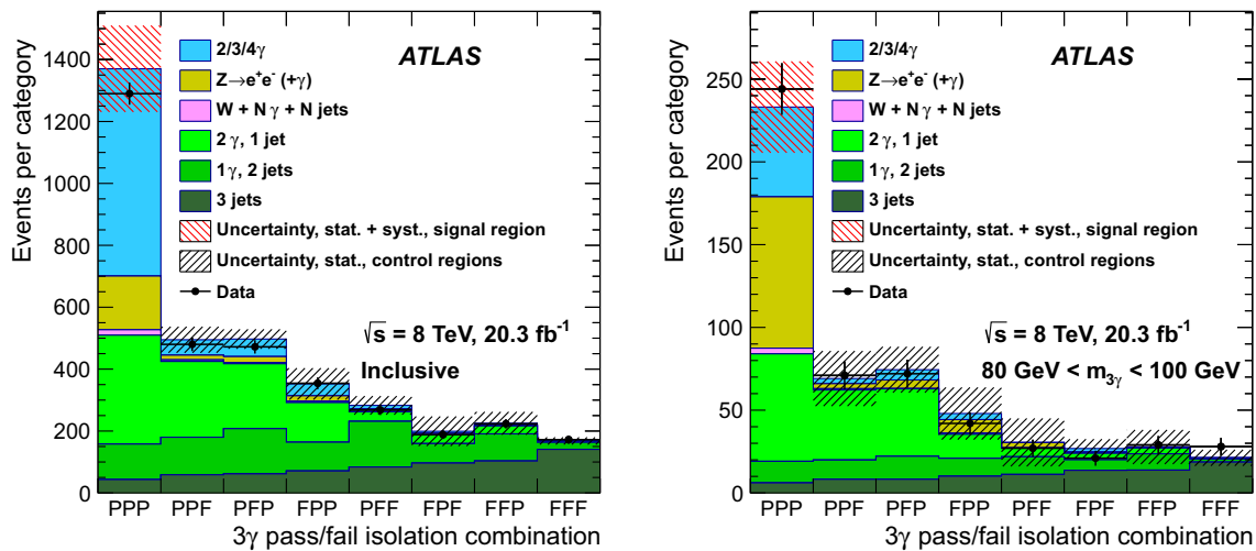
Fig. 2 Observed and expected yields in signal and control regions for the full mass range (left) and the restricted range of 80 \text{ GeV} < m_{3\gamma} < 100 \text{ GeV} (right), for events where all three photon candidates satisfy the tight photon identification criteria. The bins along the horizontal axis correspond to orthogonal subsets of events where each subset is categorised by whether the three photons – ordered from largest to smallest values of p_T – passed (“P”) or failed (“F”) the isolation criterion. The leftmost bin is the signal region, composed of events satisfying PPP, and
